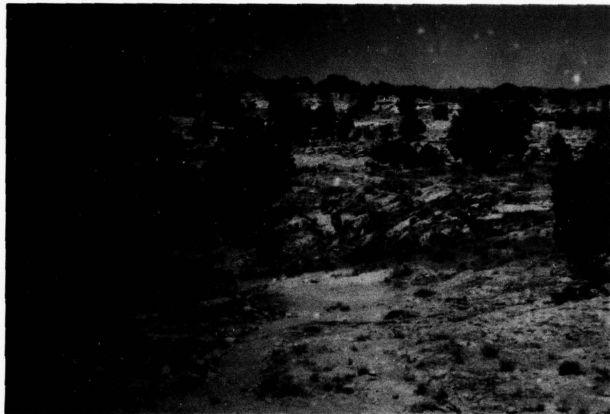
Figure 27. Land Type Blue Green (Sample subarea 18, in Moenkopi Wash)
