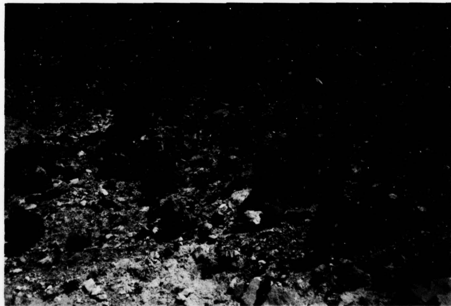
Figure 22. Land Type Light Blue Tan (Sample subarea 55, in the San Juan Basin west of Sheep Springs)
