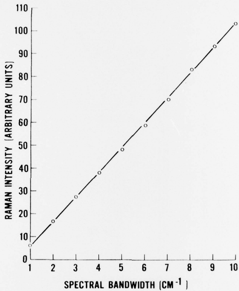
Figure 6. Plot of Raman peak height intensity for the 4155 \text{cm}^{-1} band vs. spectral bandwidths (results from Figure 5 spectral measurement).
