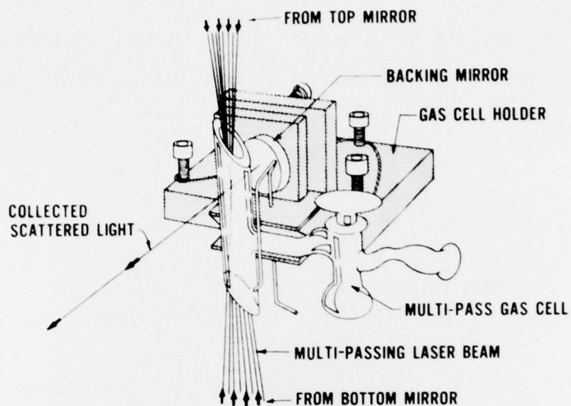
Figure 2. Multipass Raman gas cell.
