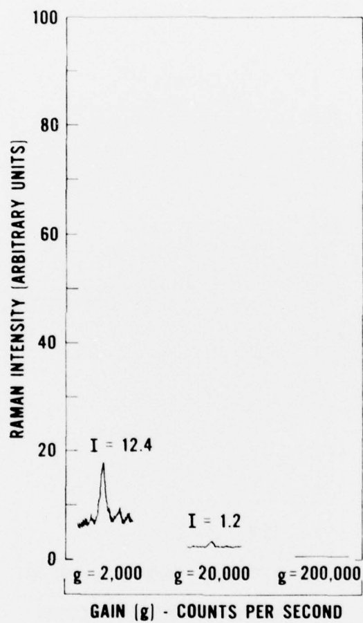
Figure 11. Raman spectra of 0.1% H 2 for the region 4100-4200 cm -1 (experimental conditions the same as in Figure 7, except SBW = 8 cm -1 ).
