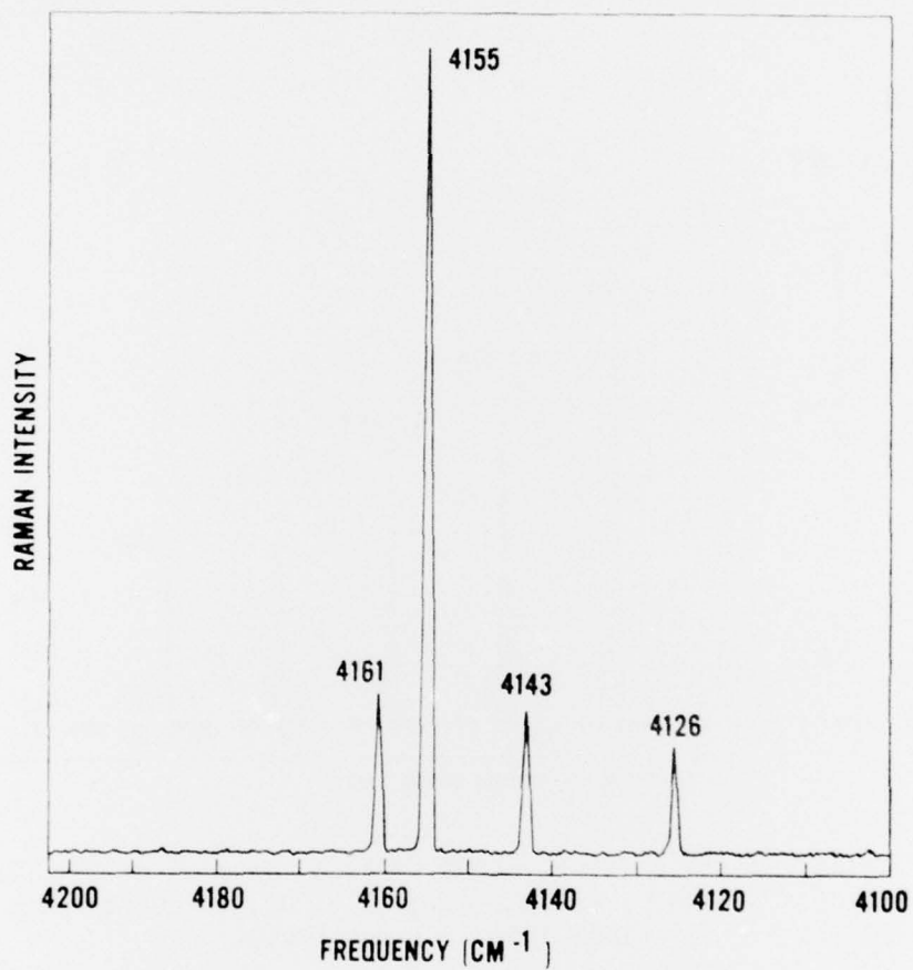
Figure 4. Raman spectrum of vibration-rotation region at high gain (laser power = 1.0 watt at sample; SBW = 0.5 cm -1 ; gain = 1,500 counts/sec; period = 2 sec; scan speed = 0.2 cm -1 /sec).
