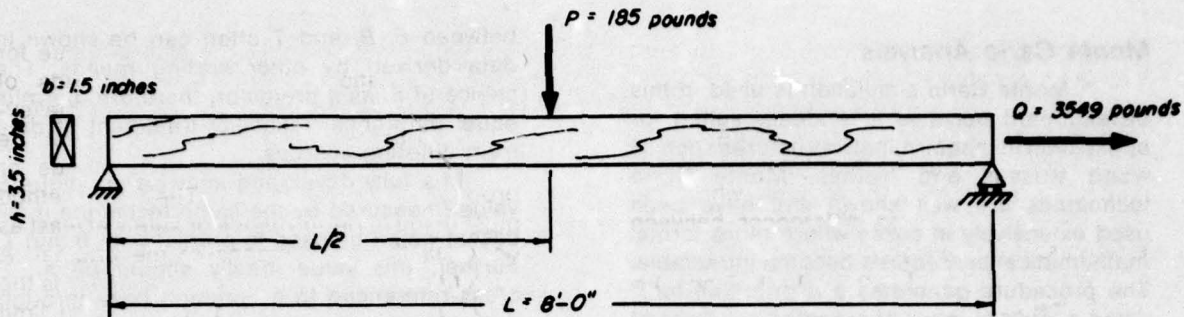
Figure 1.—This structure, which serves as an example in the analysis, is a lumber bending member bearing a single concentrated load, P , while also being subjected to a tensile load, Q . The loads have been proportioned so that both
