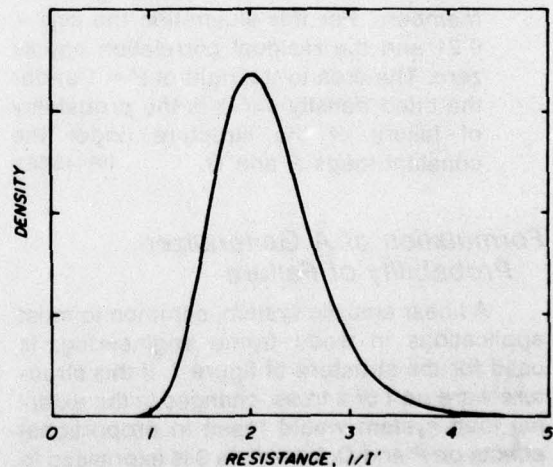
Figure 8.—The random variable 1/I' is a resistance variable. The distribution is defined by the reciprocals of I' values shown in figure 6. The I' data were fitted by the lognormal distribution and consequently 1/I' is fitted equally well by the lognormal distribution. (M 145 657)
