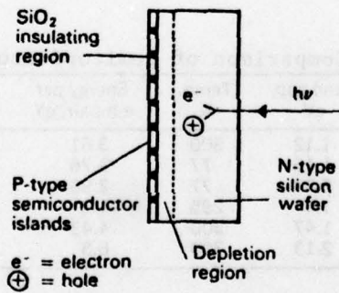
Figure 2. Target for Silicon Vidicon Tube.
