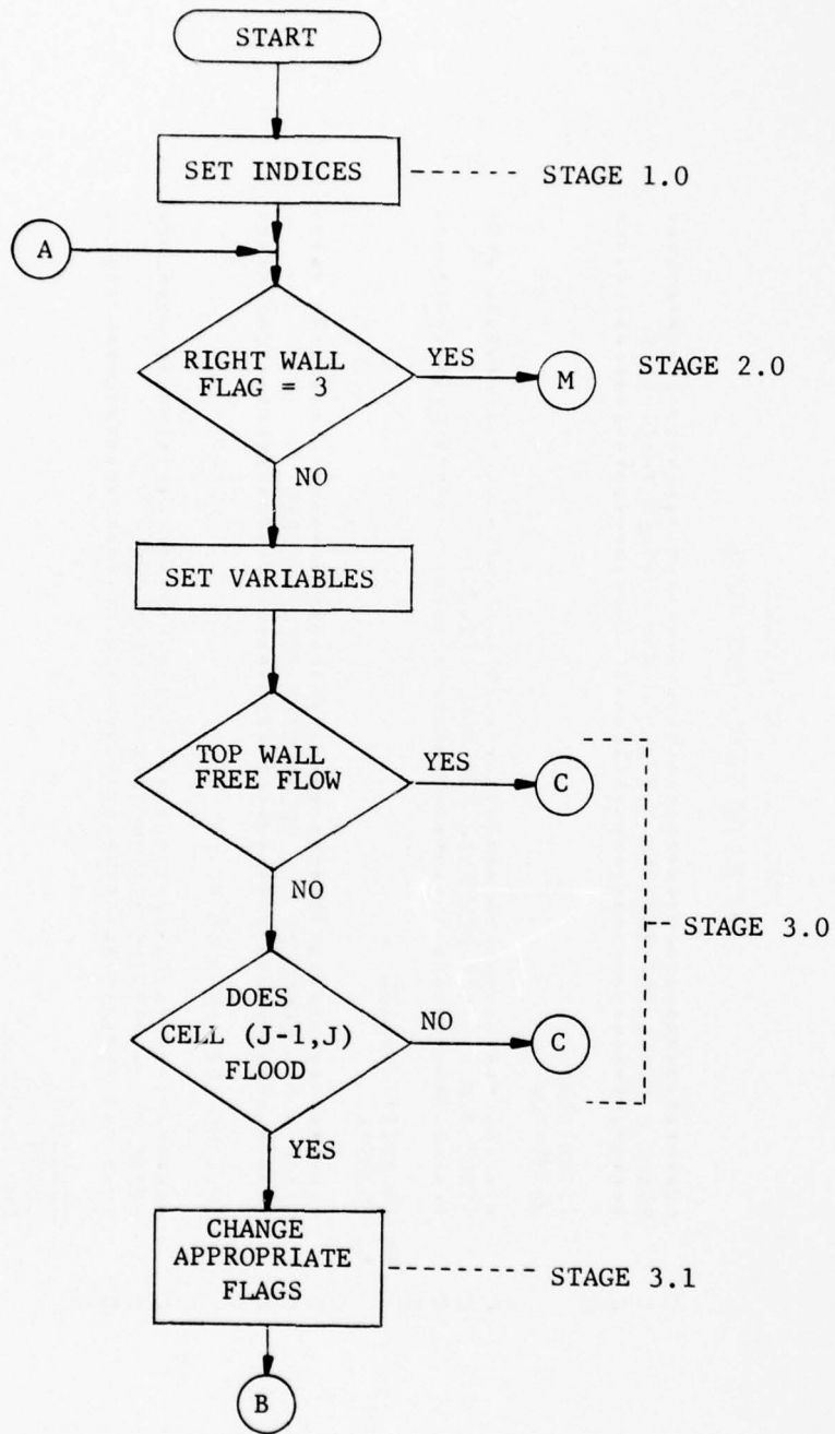
FIG. 5.4 FLOW CHART FOR SUBROUTINE TRACE
