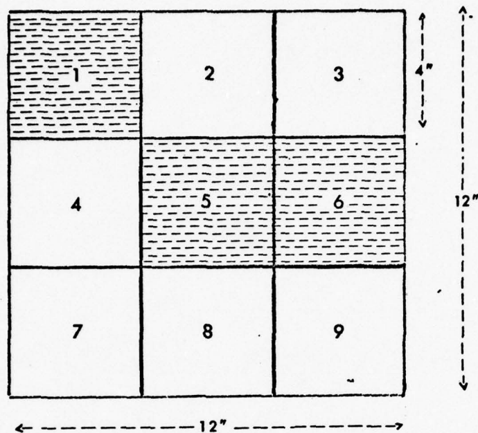
FIGURE 3.12 THE THREE SHADED POSITIONS REPRESENT THE AREAS OF A MICROWAVE OVEN CHECKED FOR OUTPUT WATTAGE
