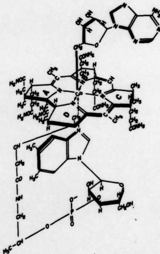
SPATIAL STRUCTURE OF COENZYME B 12
