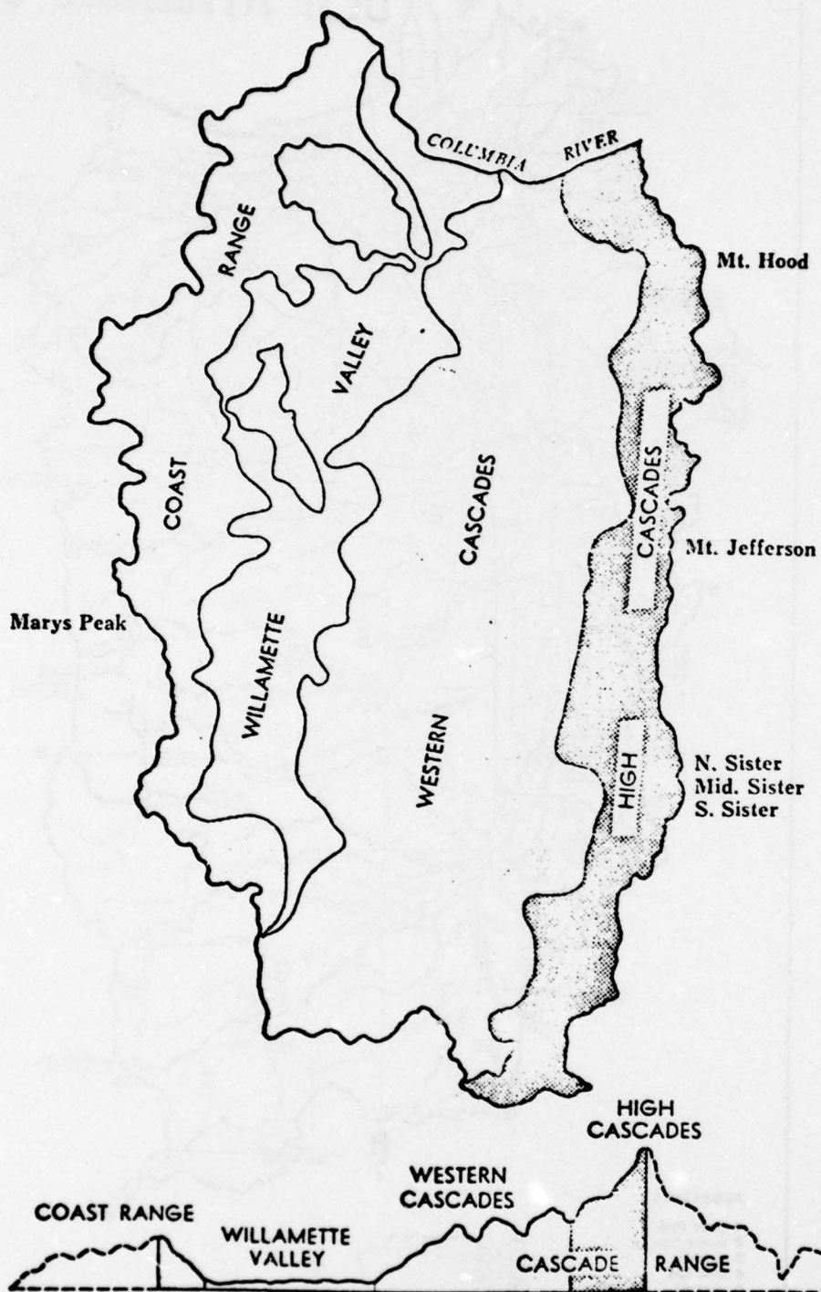
Physiographic units.
