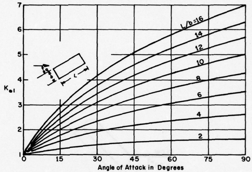
Fig. 6.05. Multiplying Factor for Angle of Attack
