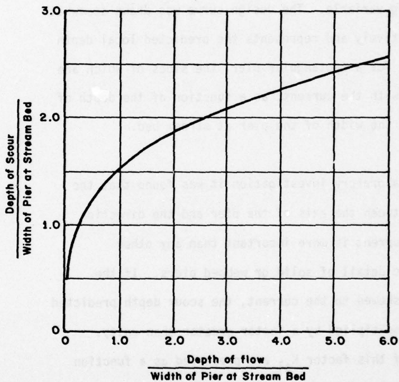
Fig. 6.04. Scour Around A Pier
