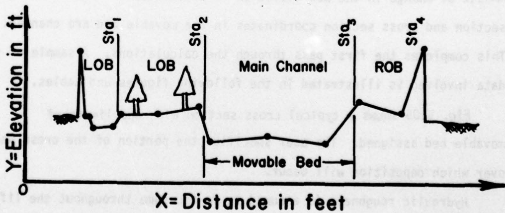
Fig. 5.05. Modeling Complex Cross Sections
