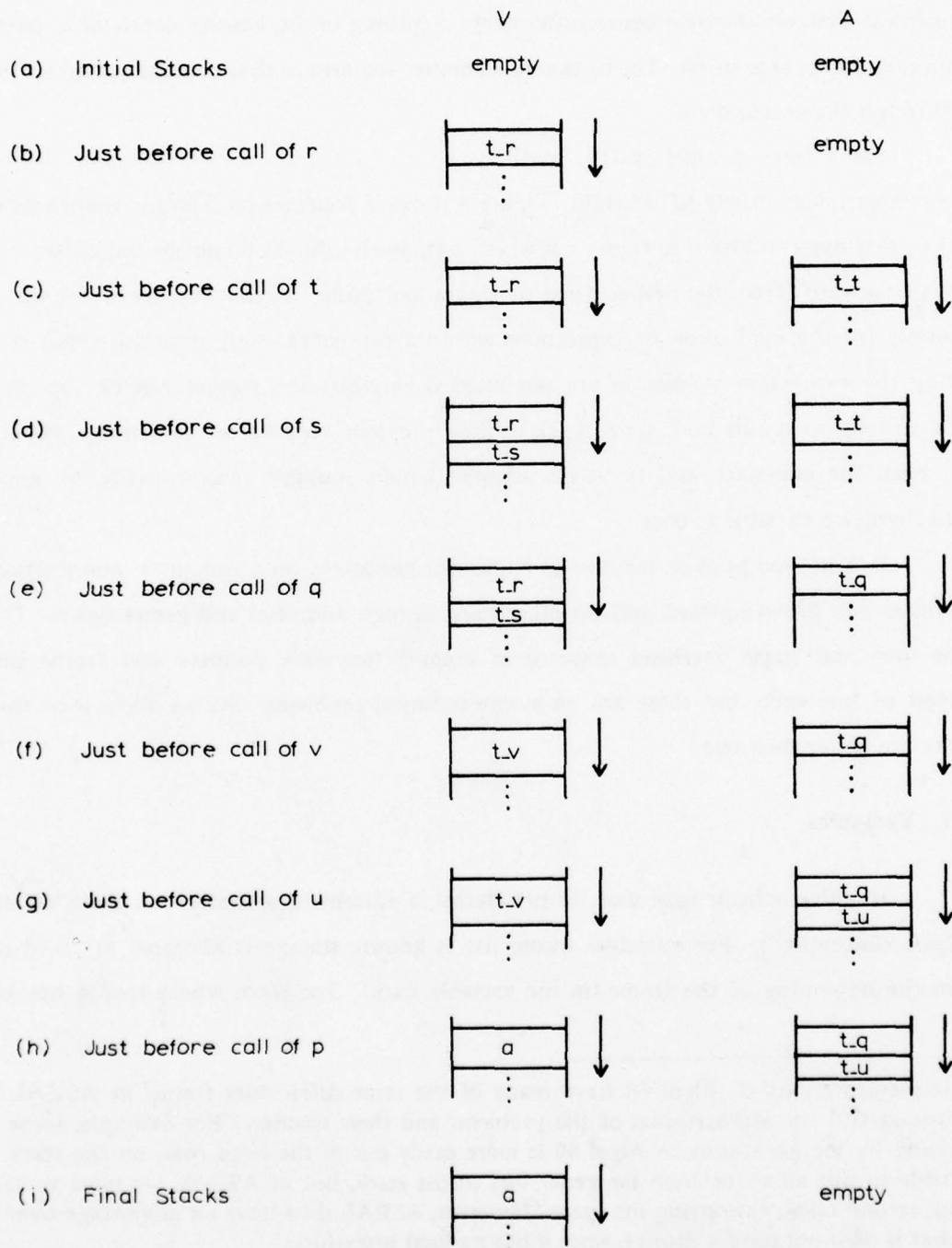
Figure 2. Scenario of the Two Stack Method Execution of 'var a: foo := p( q(r(), s(t())), u(v()) );'
