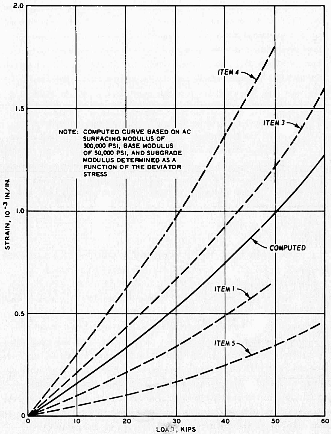
Figure A12. Comparison between computed and measured subgrade strain
