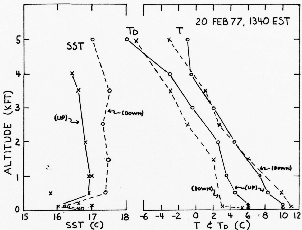
VARIATION OF IR-SST FROM AIRCRAFT AS FUNCTION OF ALTITUDE; MEASUREMENTS MADE OVER FLORIDA QUEEN NEAR STAGE ONE PLATFORM OFF PANAMA CITY, FLA. WHEN SHIP BUCKET TEMPERATURE = 13.8 C AND SATELLITE TEMPERATURE = 10.5 C
