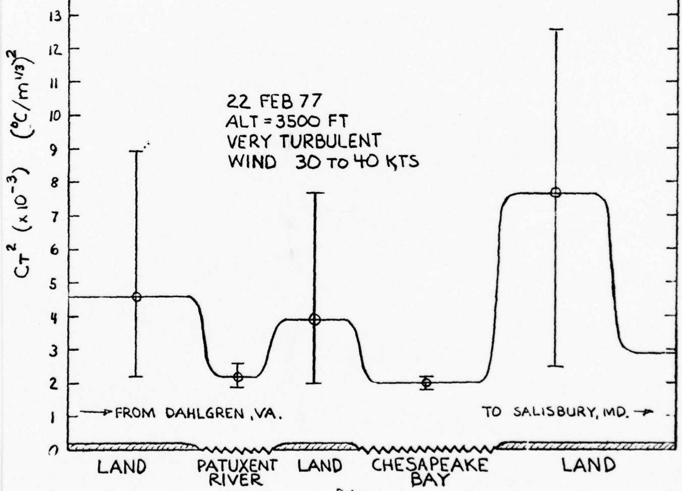
21 CT 2 TURBULENCE VARIATION LAND vs WATER
