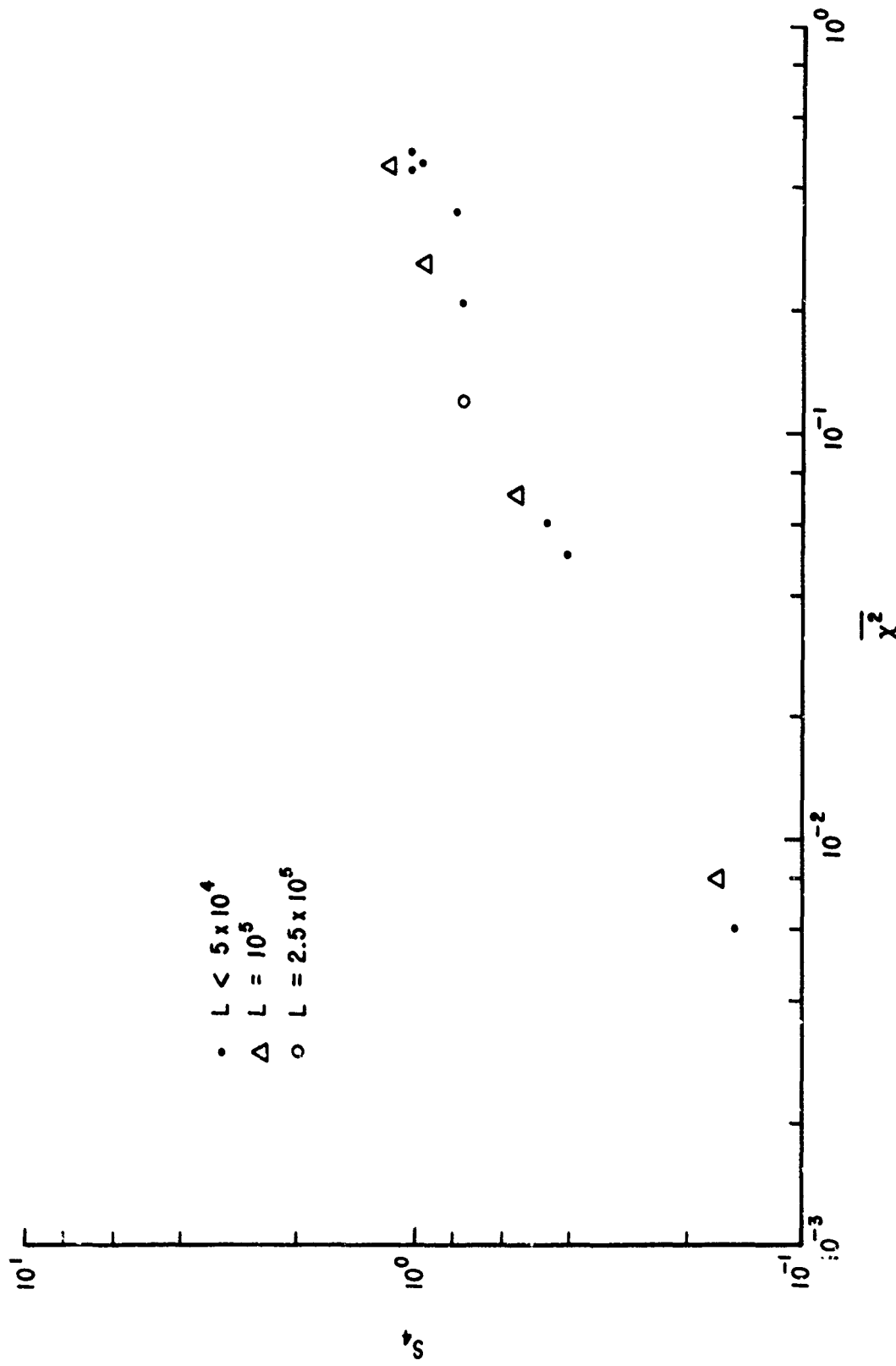
Figure 41. S_4 vs. \overline{X_2^2} for K_p^{-3} Spectrum
