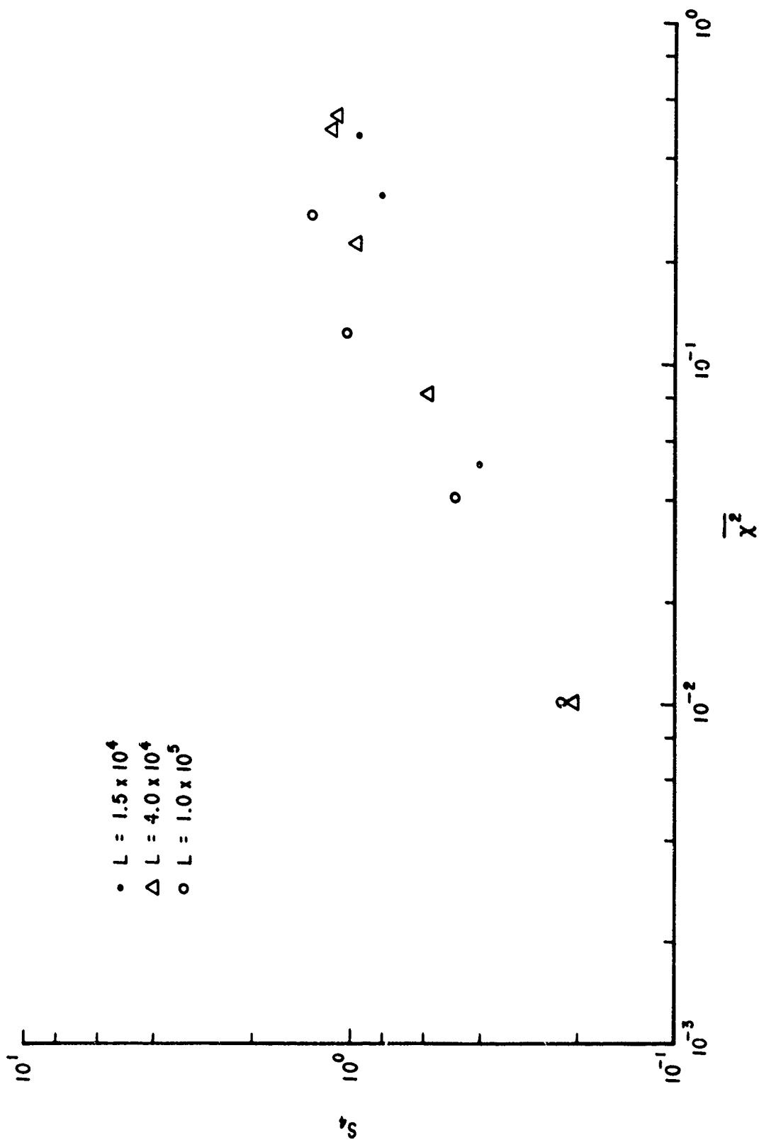
Figure 58. S_4 vs. X^2 for K_\rho^{-5} Spectrum
