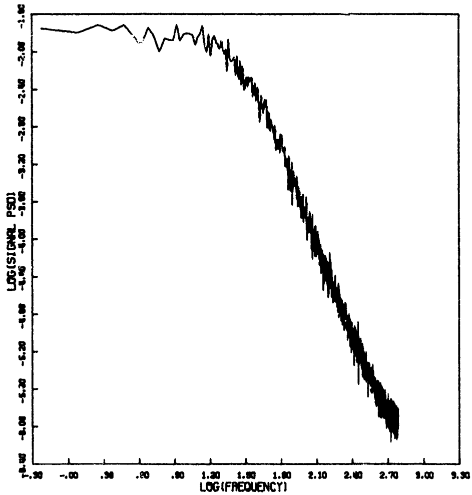
Figure 25f. Signal Power Spectral Density
