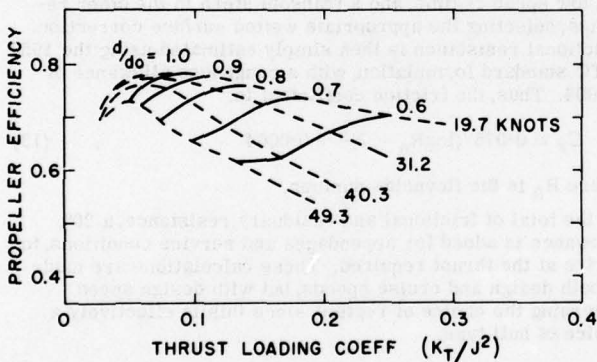
Fig. 11. Performance envelopes for controllable-pitch propellers
