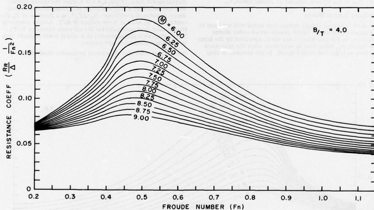
Fig. 6. Residuary resistance coefficient—High speed regime, B/T = 4.0
