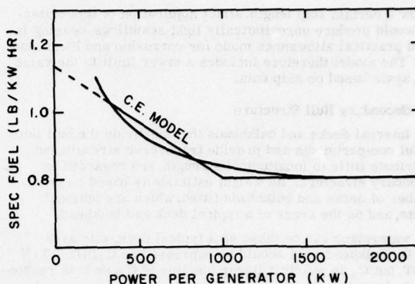
Fig. 15. Specific fuel consumption (electrical)
