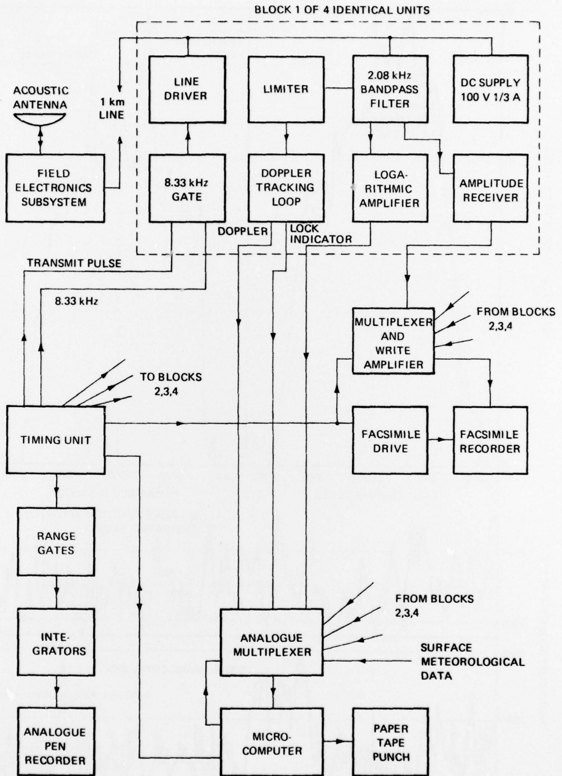
Figure 16. Simplified block diagram of the mobile acoustic wind-sensing facility.
