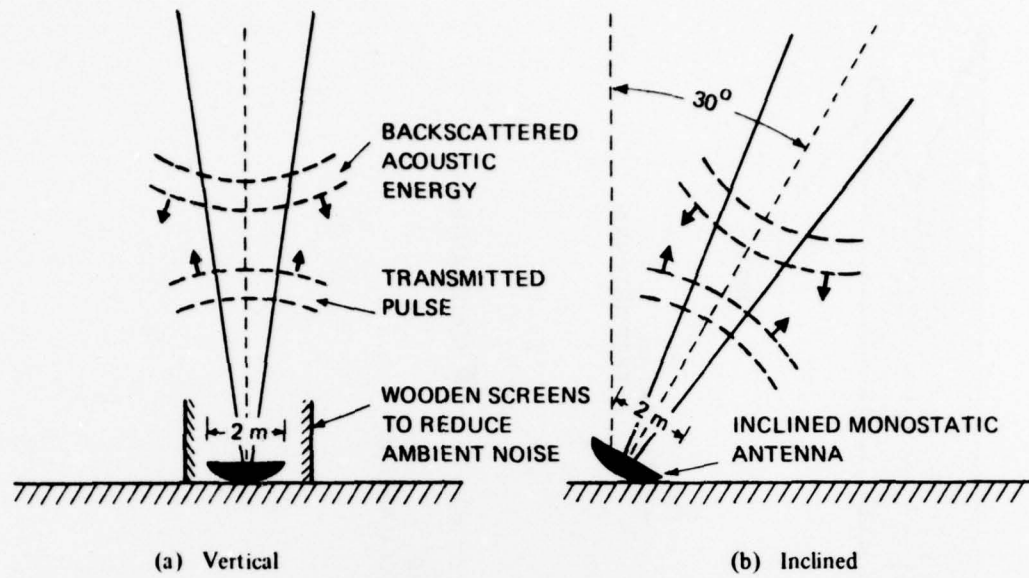
Figure 2 (a) & (b). Acoustic antenna configurations employed for monostatic wind measurements.
