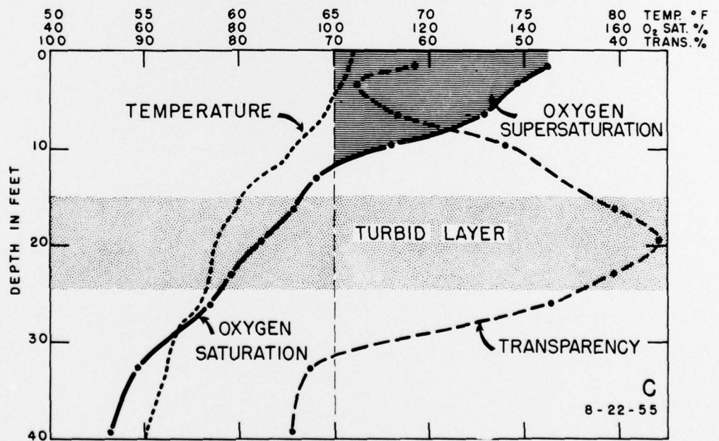
FIGURE 8. RELATION OF VERTICAL TEMPERATURE, TRANSPARENCY AND OXYGEN SATURATION OFF MISSION BEACH.
