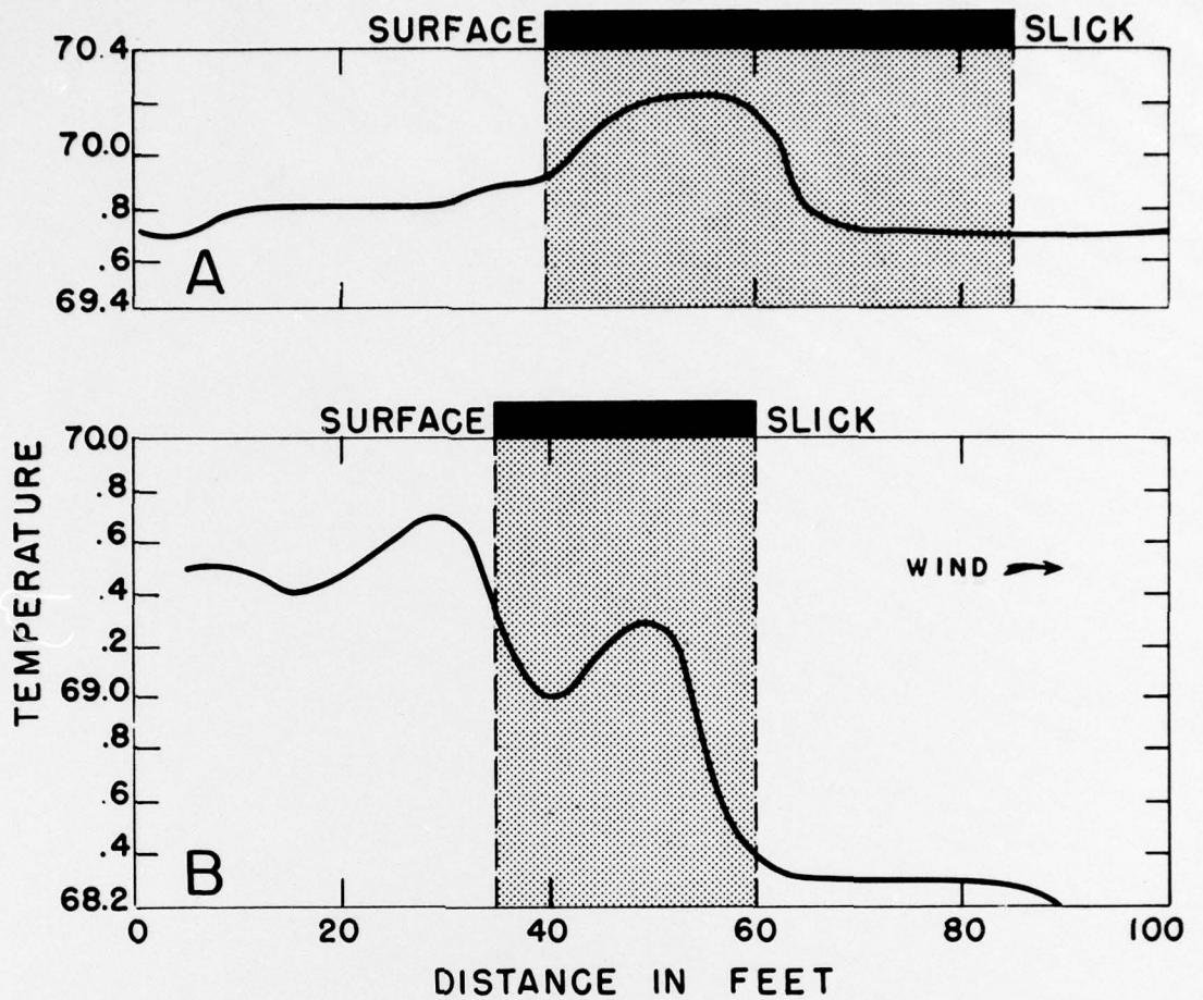
FIGURE 9. SURFACE TEMPERATURES THROUGH FOAM SLICKS IN AUGUST. A. CONVERGENCE TYPE SLICK. B. BOUNDARY TYPE SLICK.
