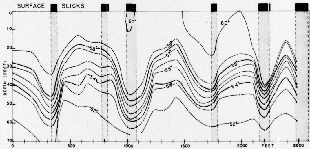
FIGURE 4. VERTICAL TEMPERATURE STRUCTURE UNDER A SERIES OF SIX SLICKS. (°F).
