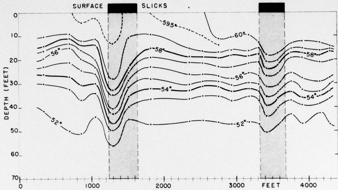
FIGURE 3. VERTICAL TEMPERATURE STRUCTURE UNDER TWO ADJACENT SLICKS (°F).
