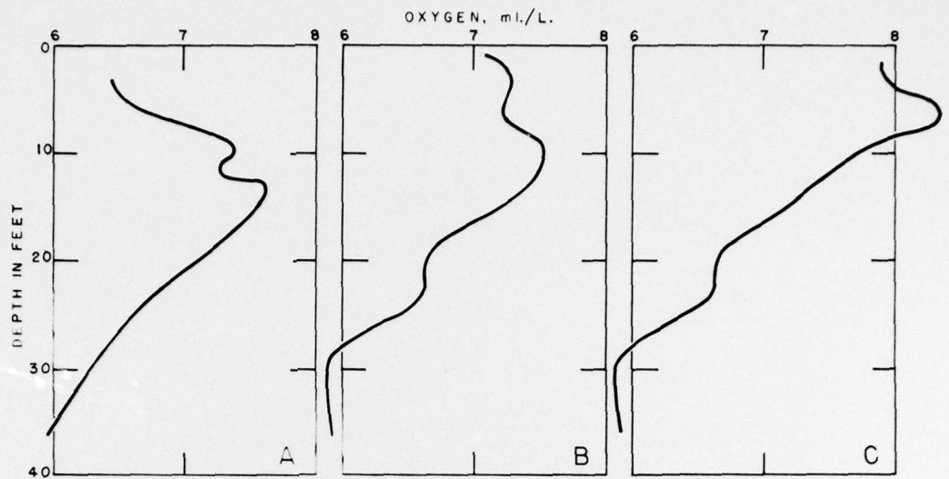
FIGURE 7. VERTICAL DISTRIBUTION OF TOTAL DISSOLVED OXYGEN AT THREE STATIONS OFF MISSION BEACH.
