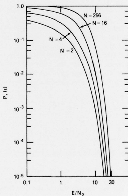
Fig. 6 — Error probability: N orthogonal signals
