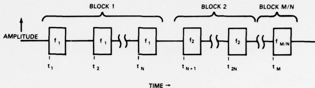
Fig. 1 — Block-to-block frequency-agile radar signal ( f_n = carrier frequency)
