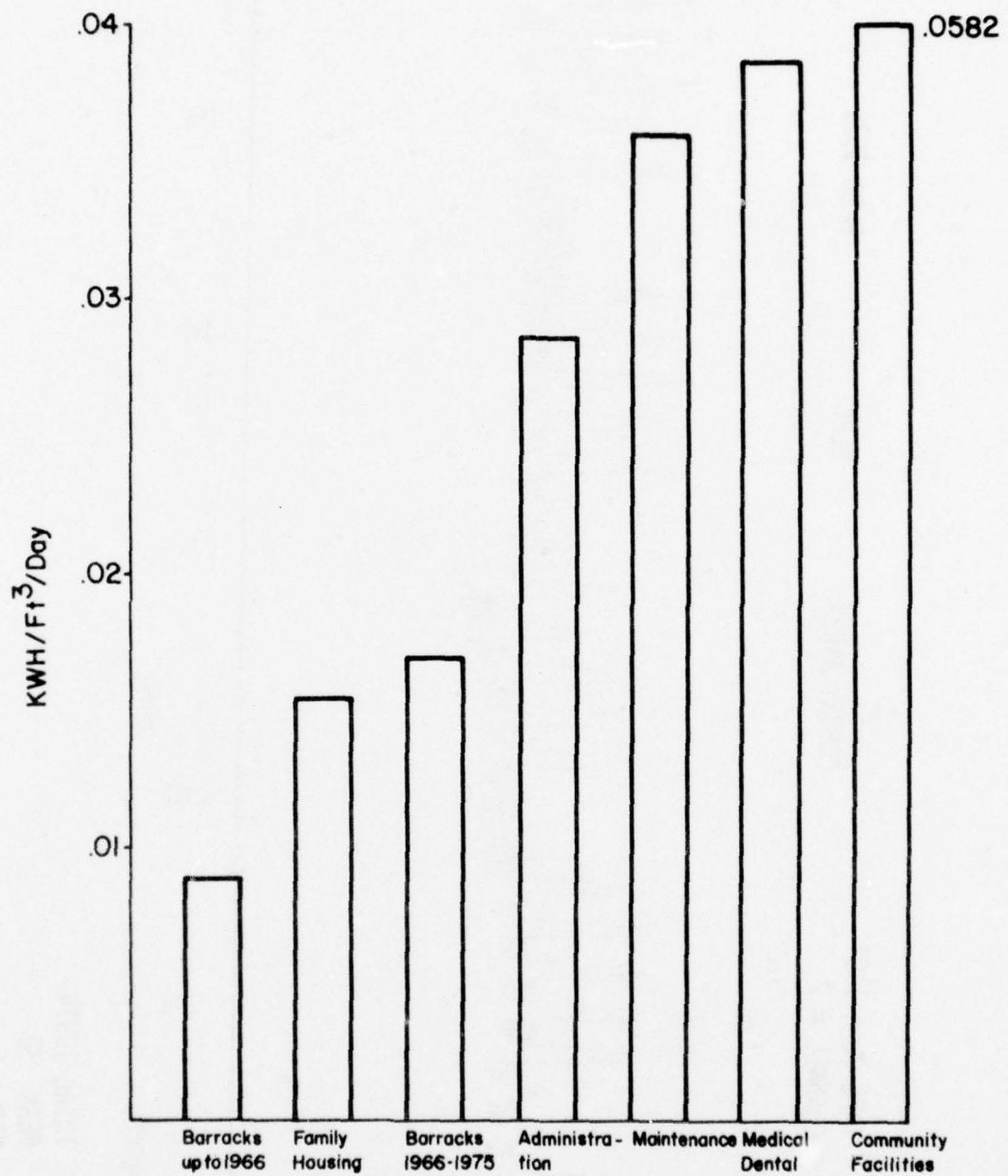
Figure 30. Average electrical energy usage by consumer group. SI conversion factor: 1 kWh/sq ft/day = 10.8 kWh/m 2 /day.
