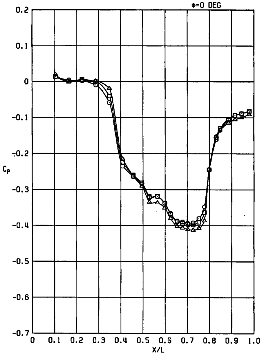
b. M_\infty = 1.2 Figure A-17. Concluded.
