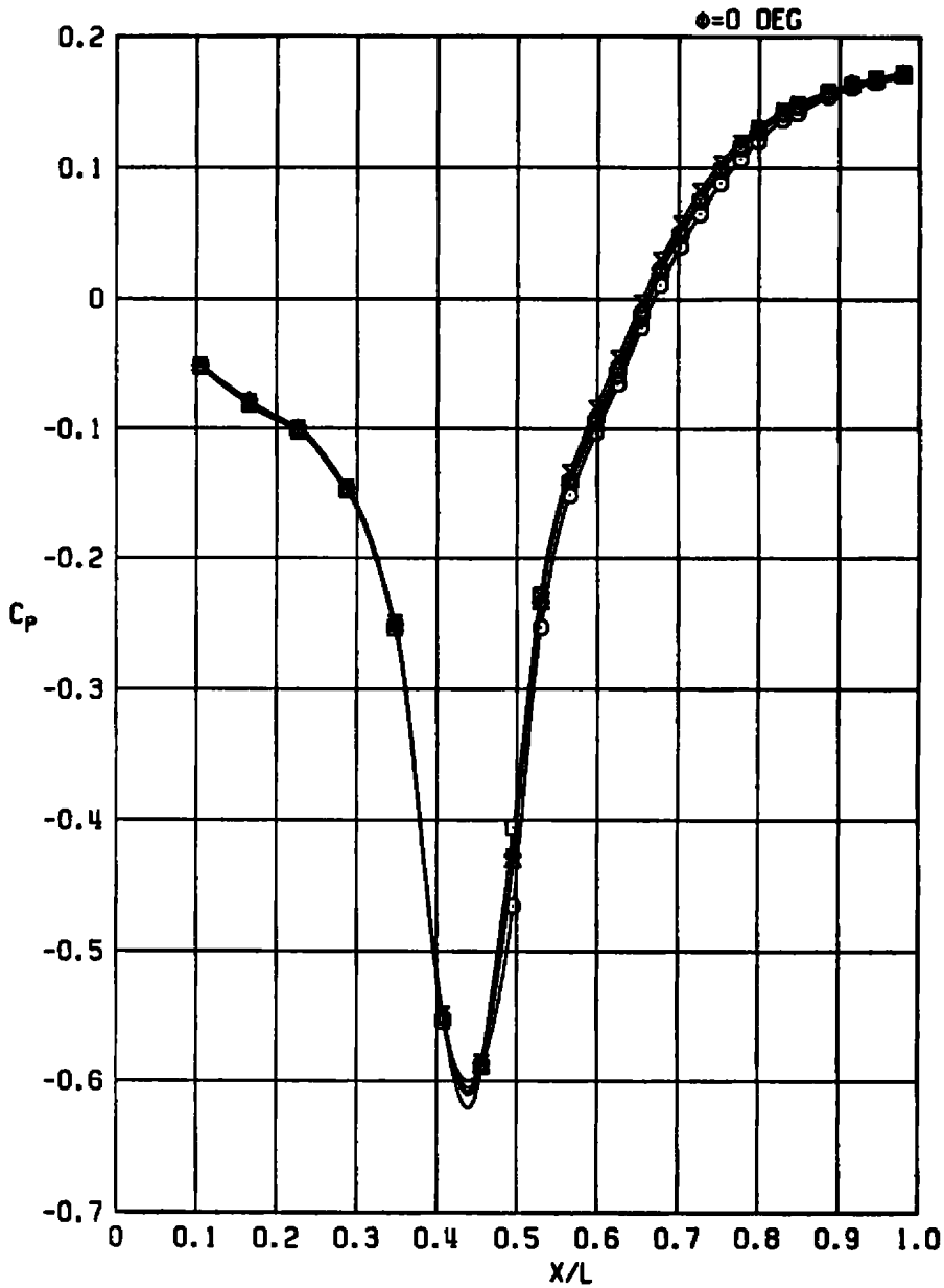
b. M_\infty = 0.9 Figure A-10. Continued.
