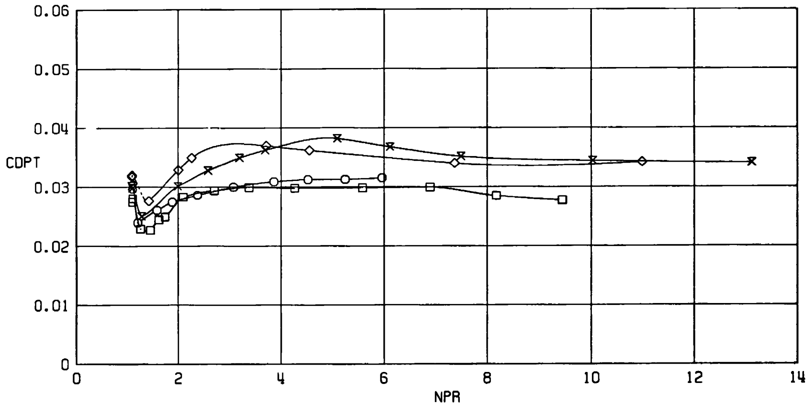
b. M_\infty = 0.9 Figure 21. Continued.
