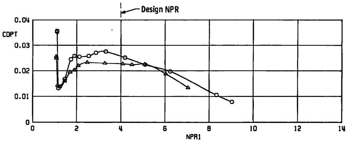
a. M_\infty = 0.6 Figure 33. Correlation of Sting Size Effects on Afterbody Drag, A/A^* \approx 1.22 .
