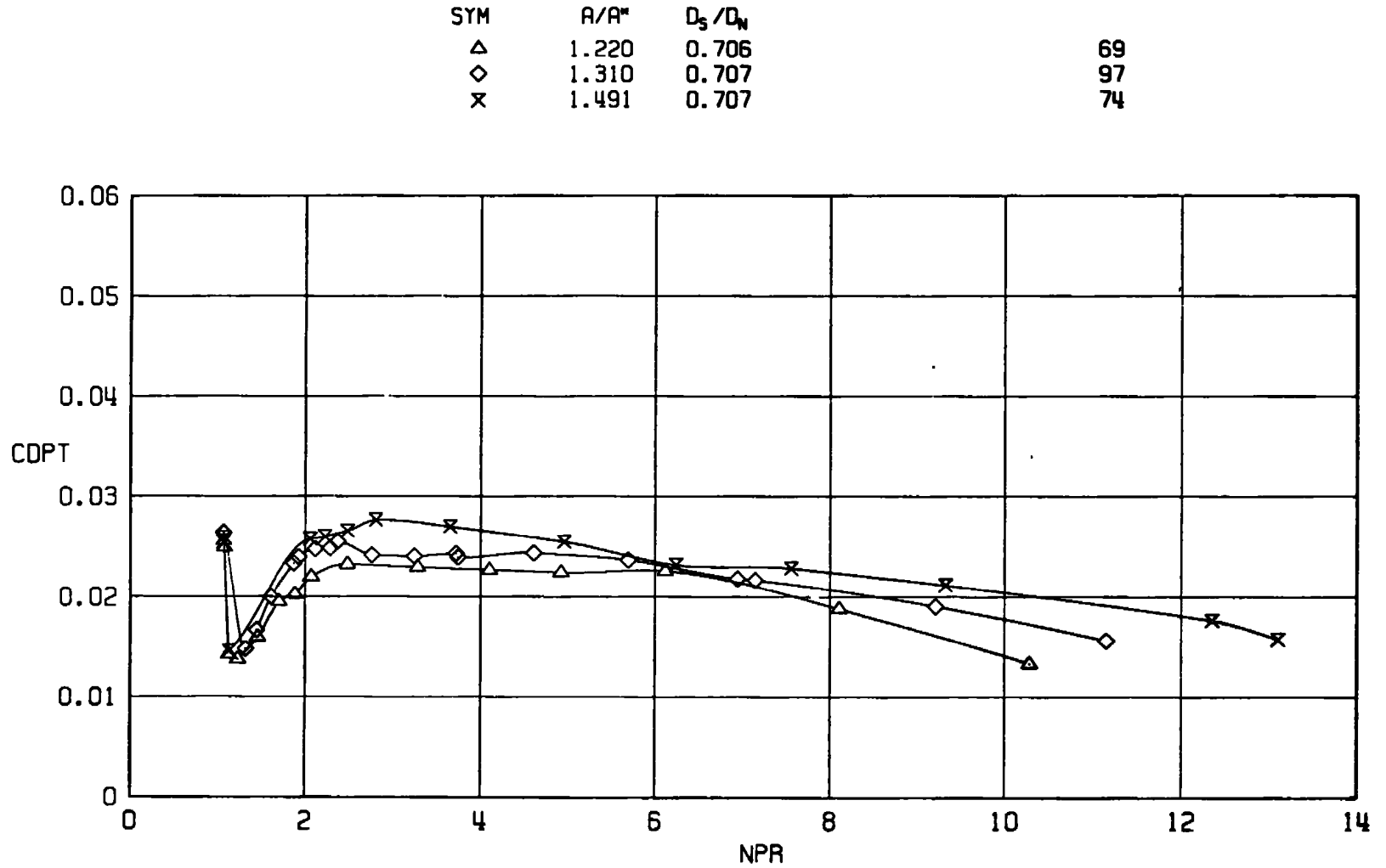
a. M_\infty = 0.6 Figure 20. Nozzle area ratio effects on afterbody drag, D_s/D_N = 0.707 .
