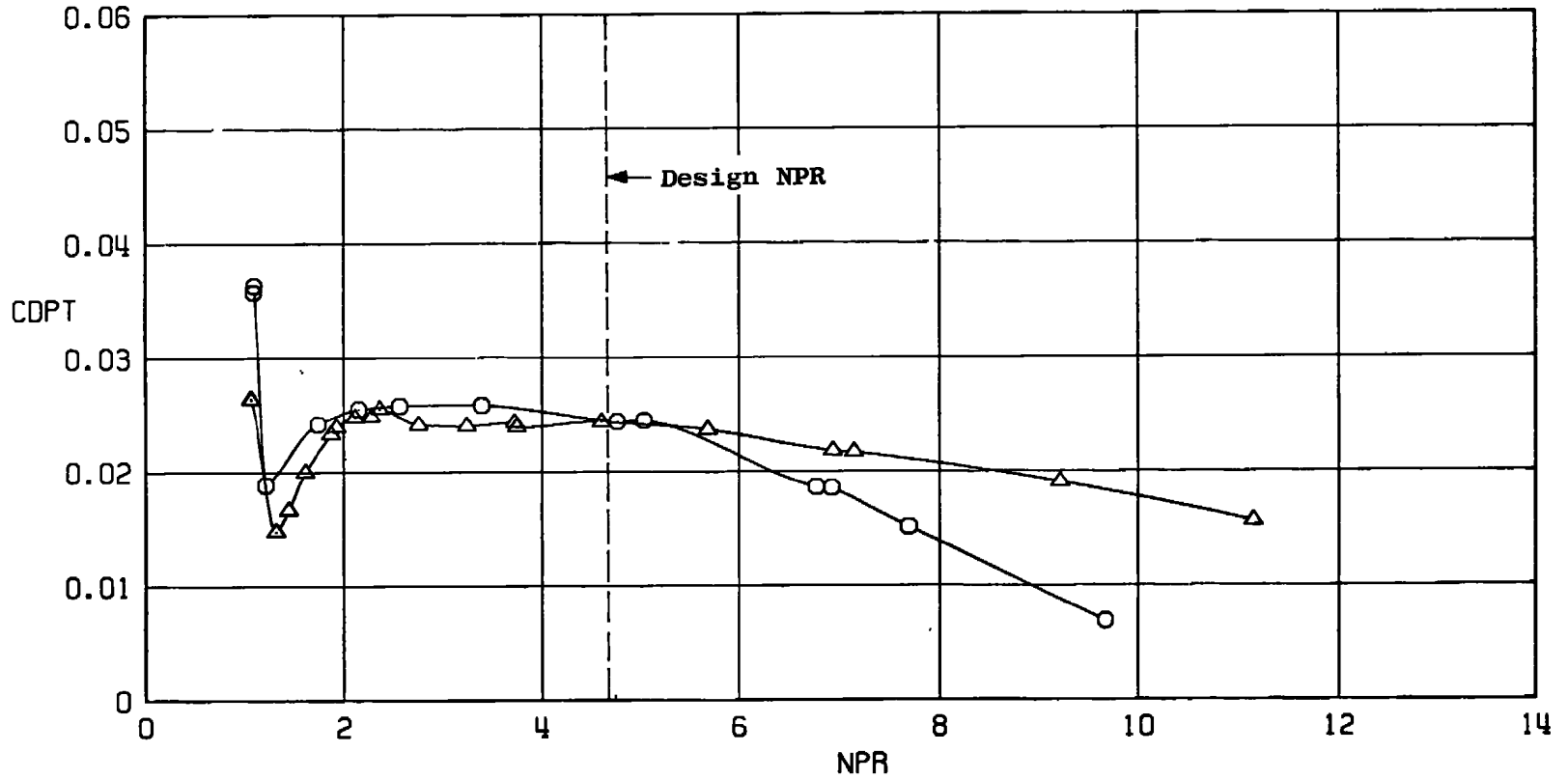
a. M_\infty = 0.6 Figure 15. Sting size effects on afterbody drag, A/A^* \approx 1.31 .
