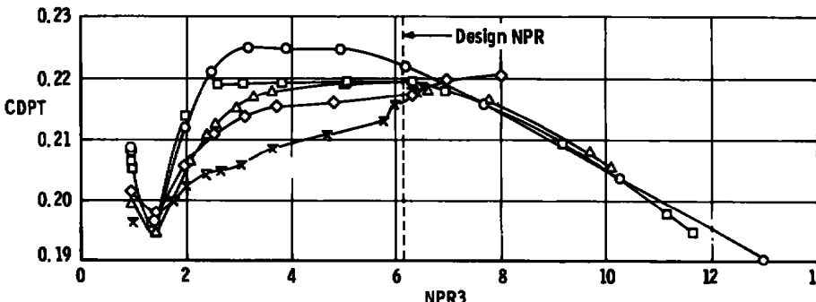
c. M_\infty = 1.2 Figure 35. Concluded.
