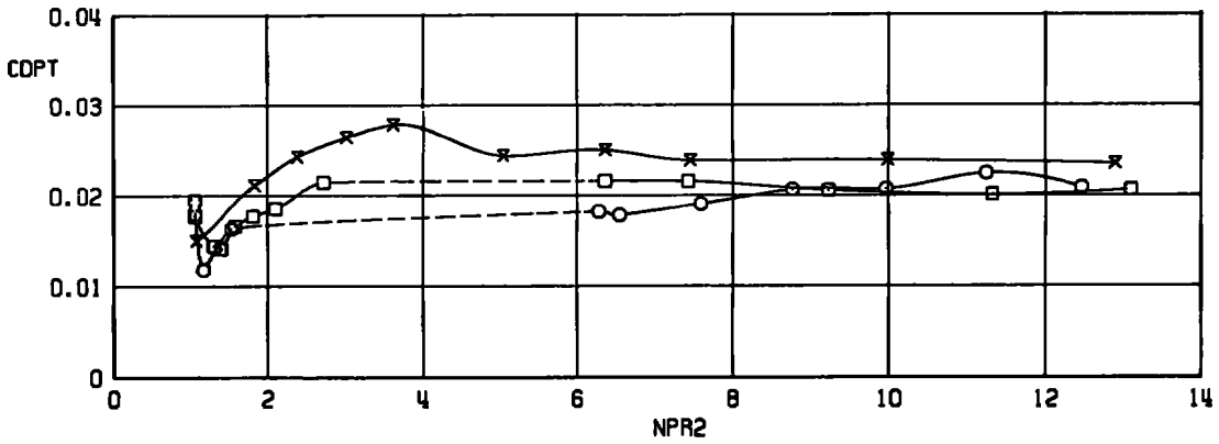
Figure 42. Correlation of nozzle area ratio effects on afterbody drag, D_s/D_N = 0.866 .
