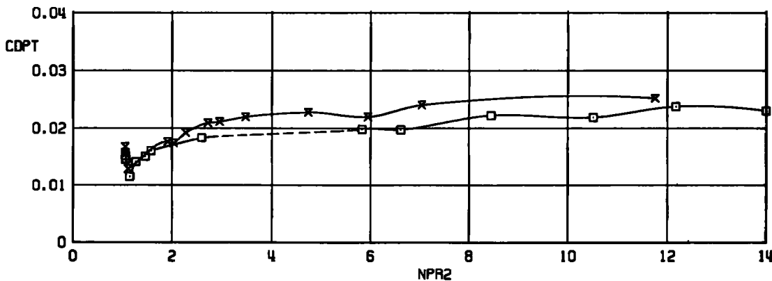
Figure 43. Correlation of nozzle area ratio effects on afterbody drag, D_3/D_N = 0.95 .
