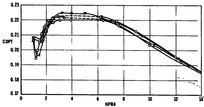
c. M_\infty = 1.2 Figure 39. Concluded.
