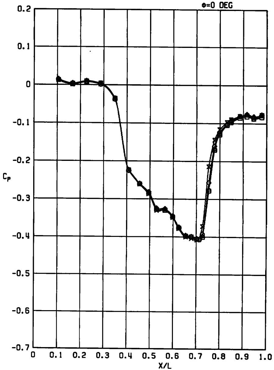
c. M_\infty = 1.2 Figure 10. Concluded.
