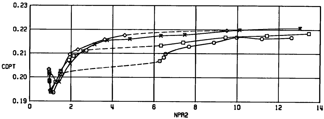
c. M_\infty = 1.2 Figure 42. Concluded.
