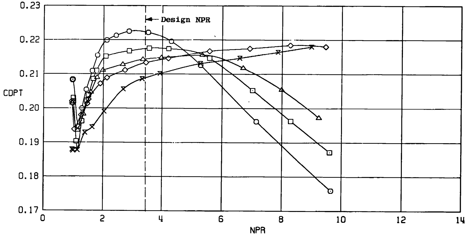
c. M_\infty = 1.2 Figure 13. Concluded.
