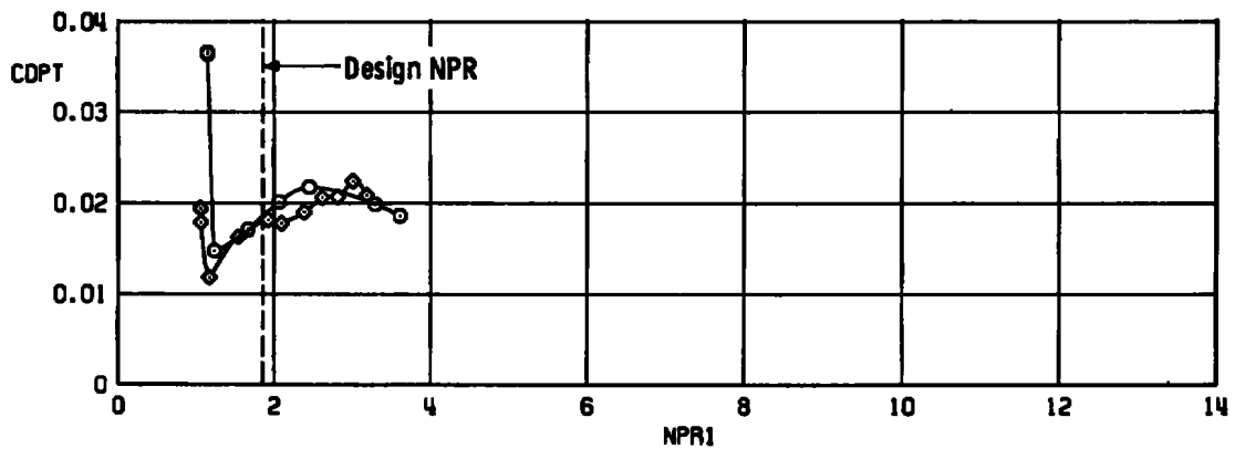
Figure 31. Correlation of sting size effects on afterbody drag, A/A^* = 1.0 .
