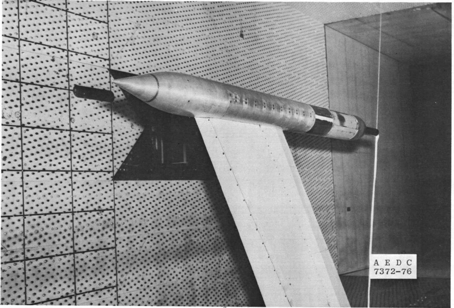
Figure 2. Model installation photograph.
