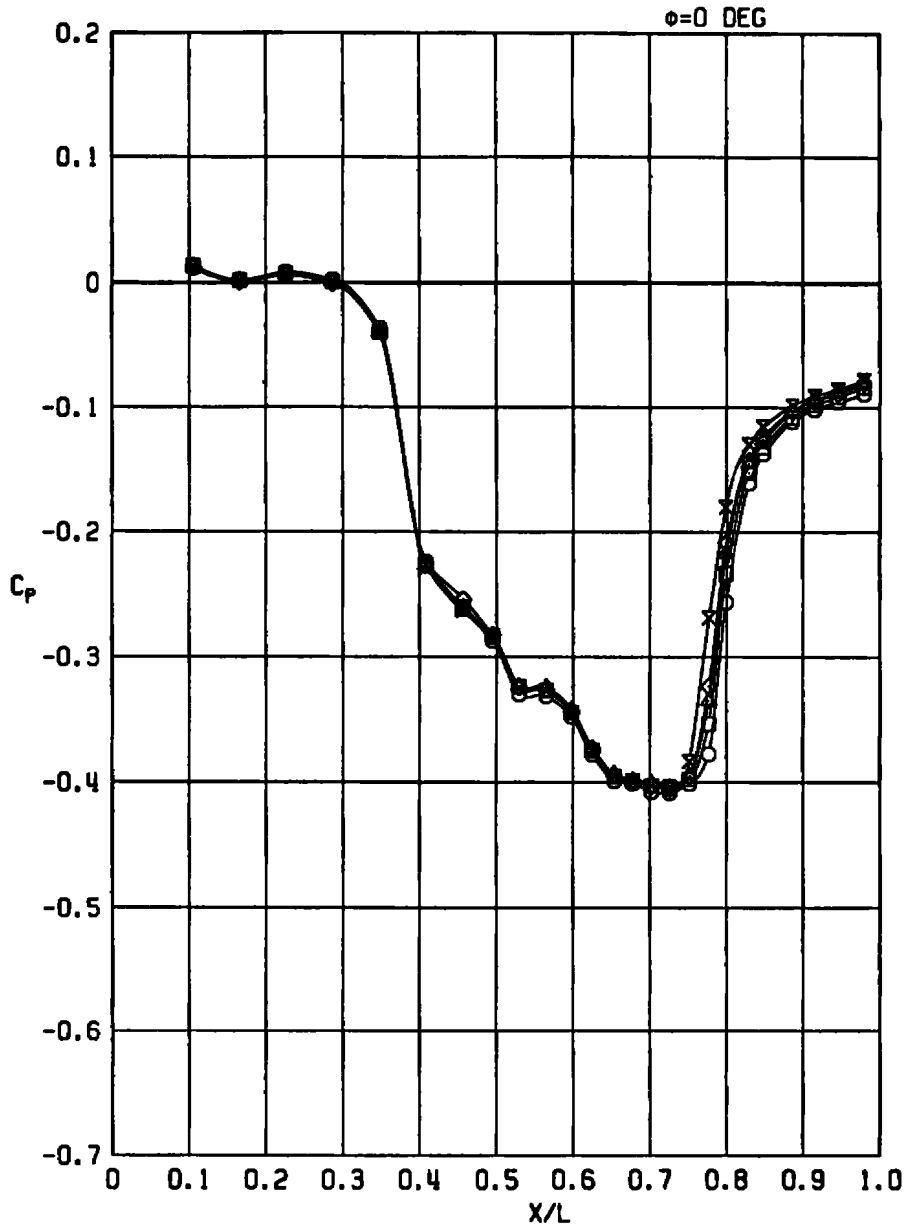
c. M_\infty = 1.2 Figure A-5. Concluded.
