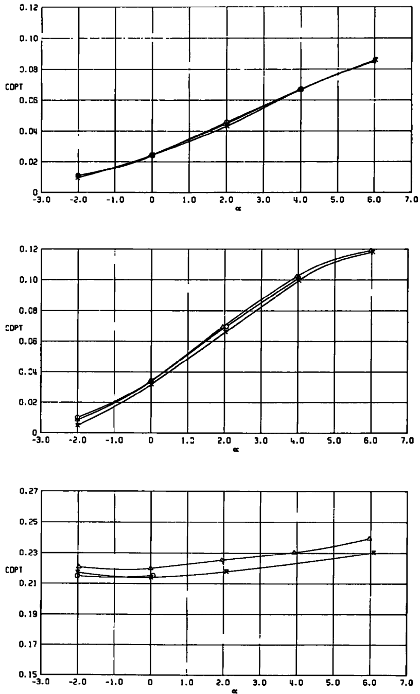
Figure 24. Influence of the annular jet on afterbody drag sensitivity to angle of attack, A/A^* \approx 1.49 .
