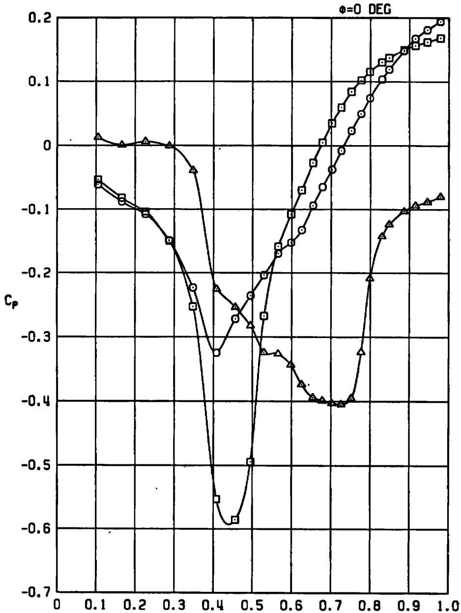
Figure A-15. Effects of Mach number, D_3/D_N = 0.866 , A/A^* = 1.142 , NSPR \approx 1.0 .
