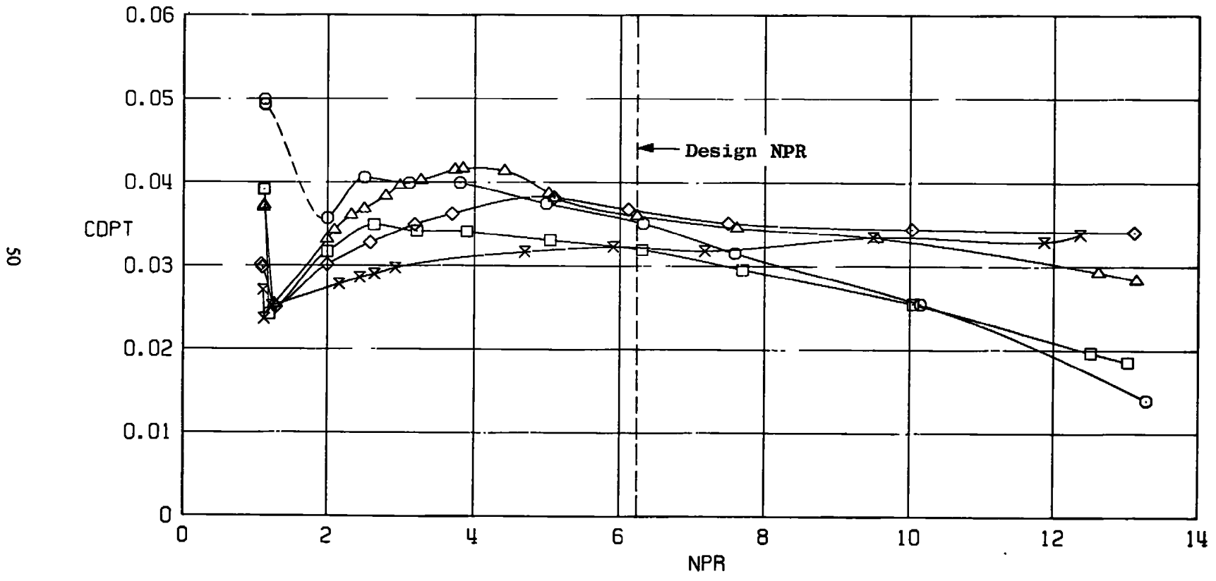
b. M_{\infty} = 0.9 Figure 16. Continued.
