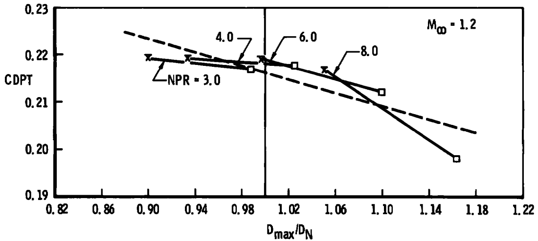
Figure 46. Variation of afterbody drag with exhaust plume maximum diameter, D_s/D_N = 0.543 .
