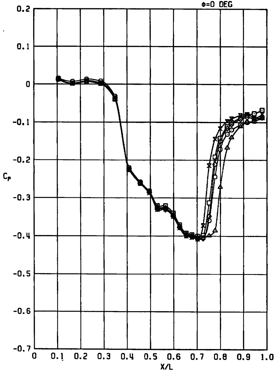
Figure A-2. Concluded.
