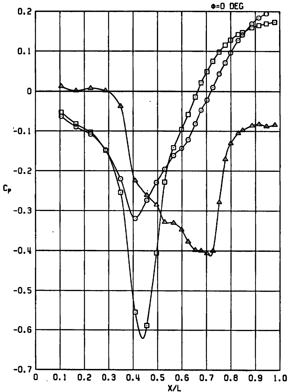
Figure A-14. Effects of Mach number, D_3/D_N = 0 , A/A^* = 1.134 , NSPR \approx 2.0 .
