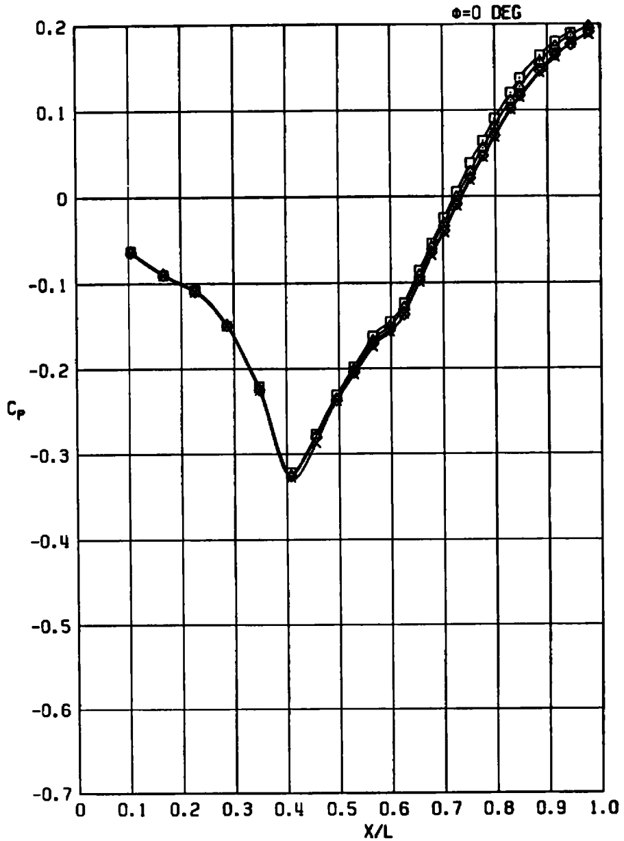
Figure A-8. Effects of sting to nozzle exit diameter ratio, A/A^* \approx 1.49 , NSPR \approx 2.0 .
