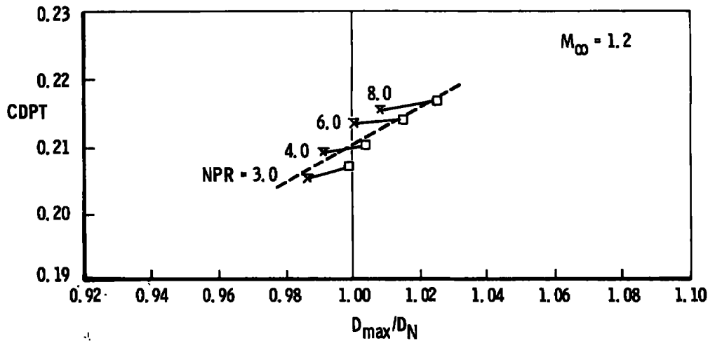
Figure 49. Variation of afterbody drag with exhaust plume maximum diameter, D_s/D_N = 0.95 .
