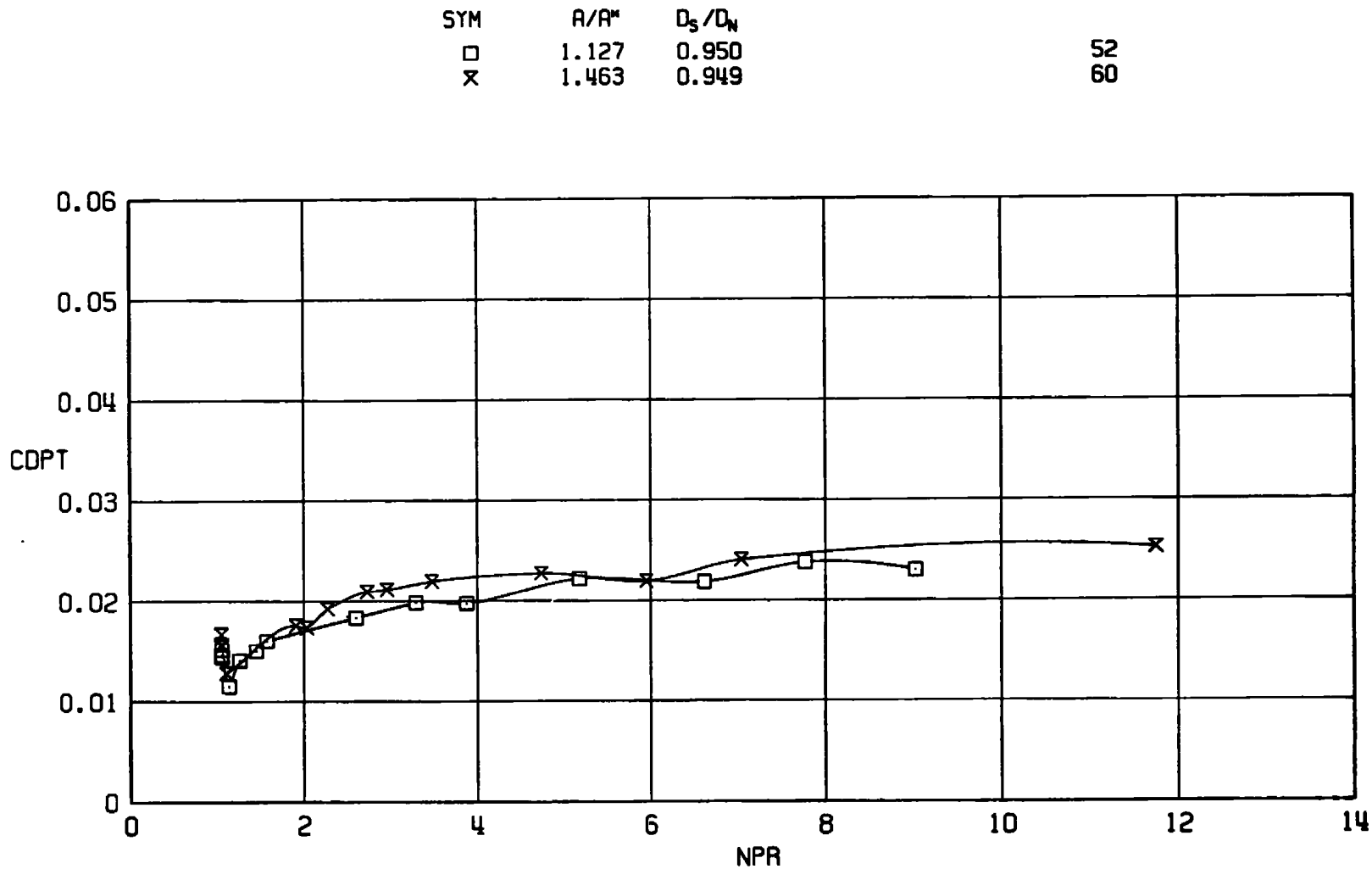
a. M_\infty = 0.6 Figure 22. Nozzle area ratio effects on afterbody drag, D_3/D_N = 0.95 .
