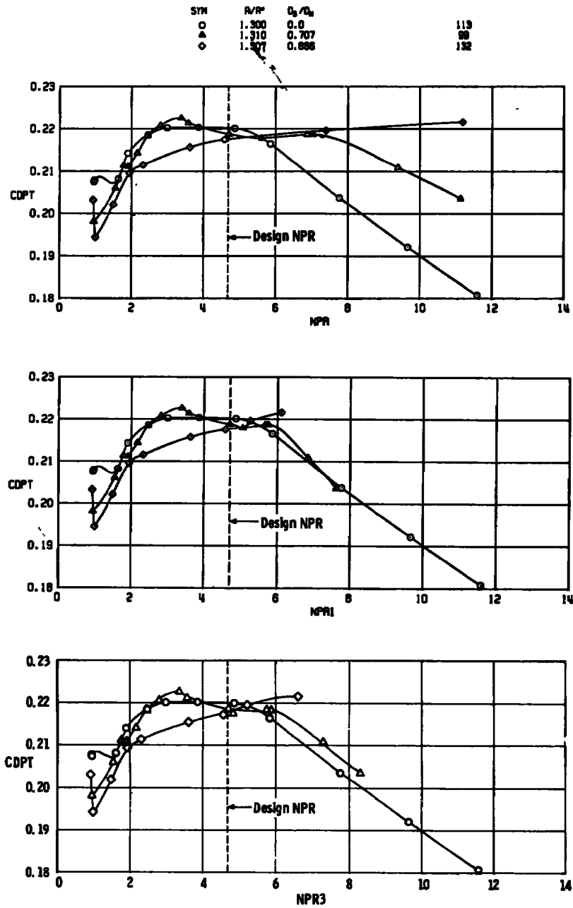
c. M_\infty = 1.2 Figure 34. Concluded.
