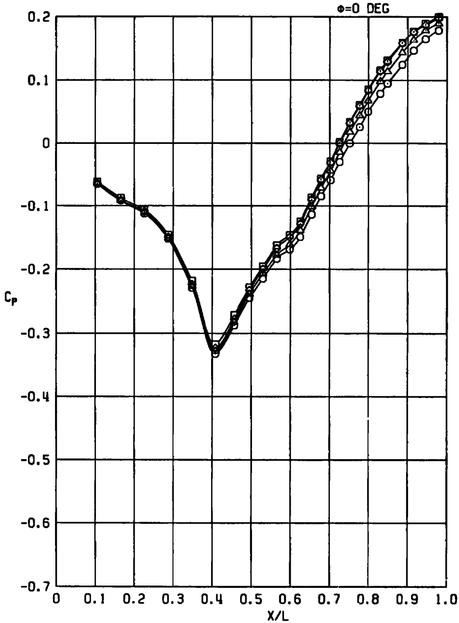
a. M_\infty = 0.6 Figure A-2. Effects of nozzle pressure ratio, D_s/D_N = 0, A/A^* = 1.490.
