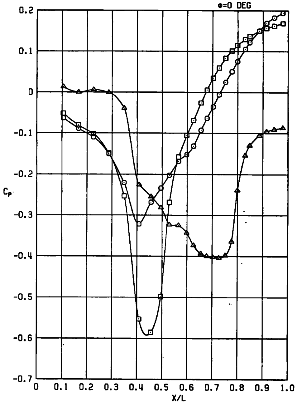
Figure A-16. Effects of Mach number, D_3/D_N = 0.866 , A/A^* = 1.142 , NSPR \approx 2.0 .
