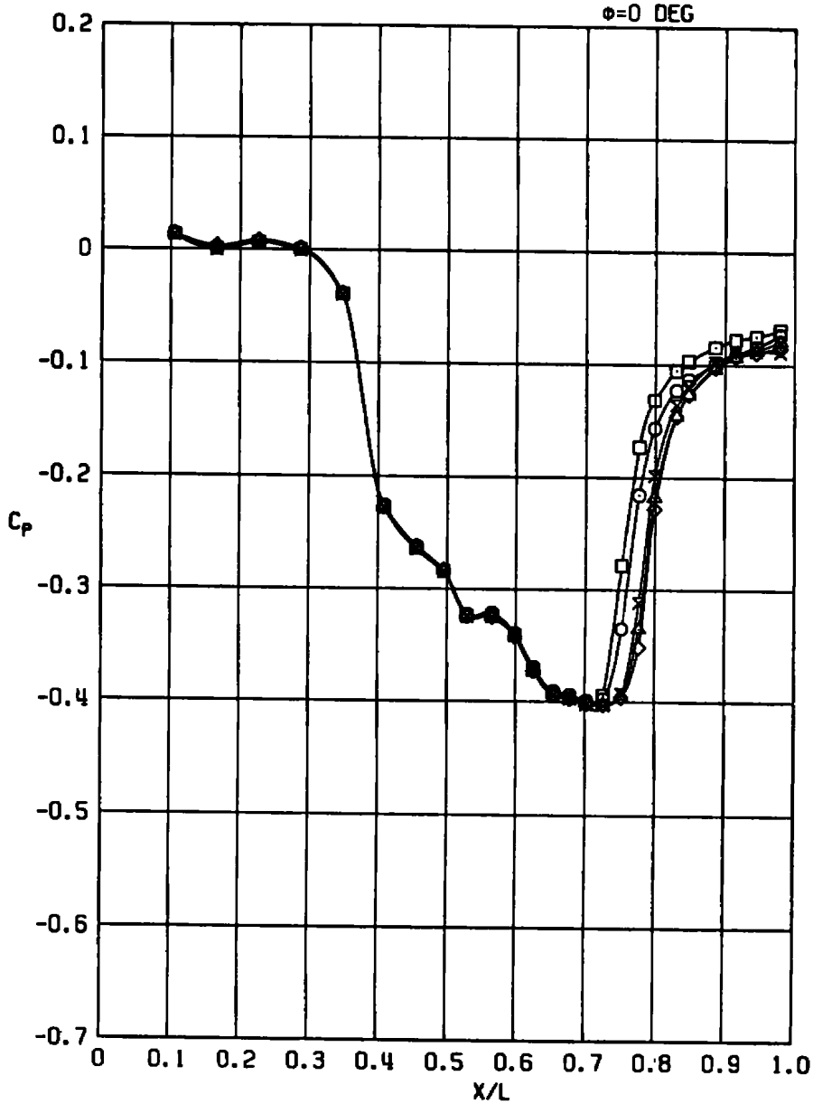
b. M_\infty = 1.2 Figure A-3. Concluded.
