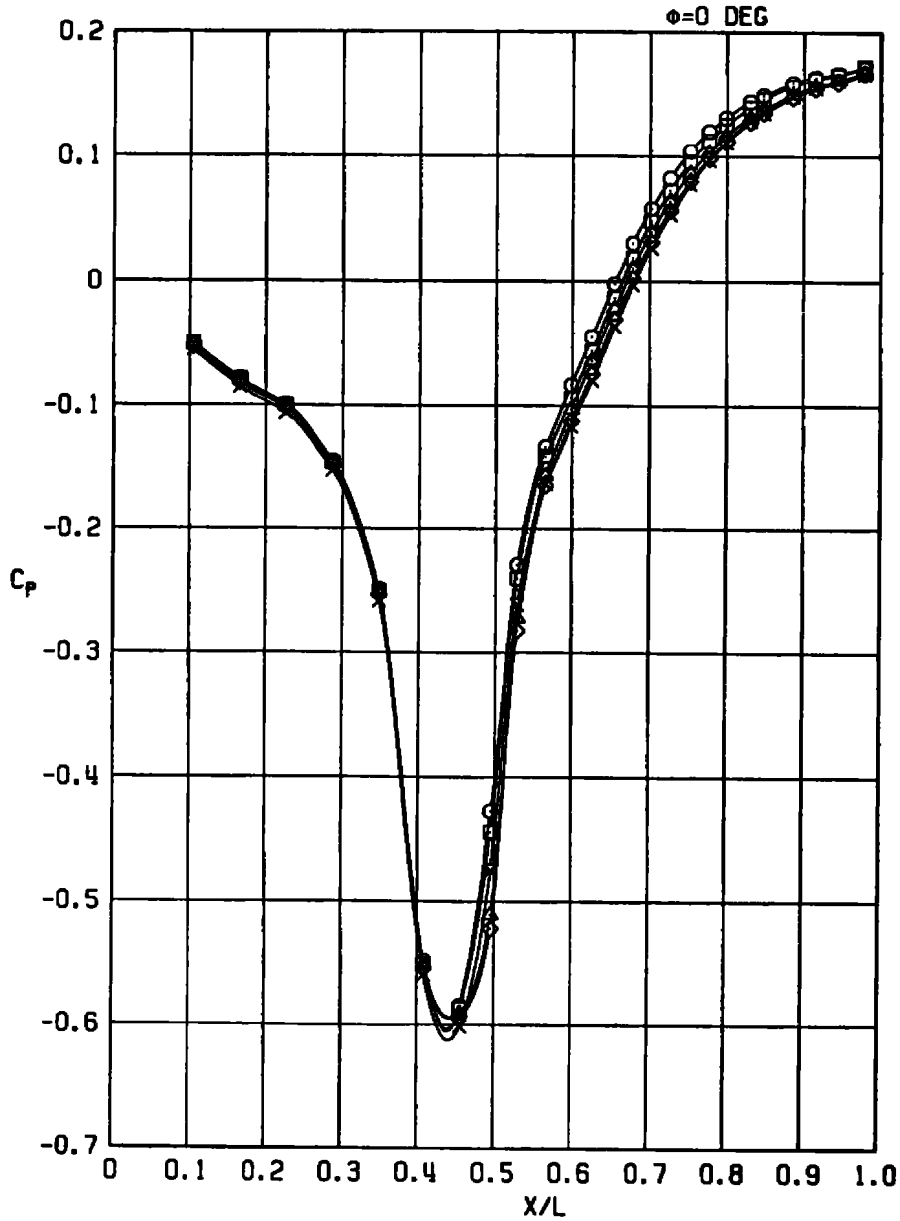
b. M_\infty = 0.9 Figure A-8. Continued.
