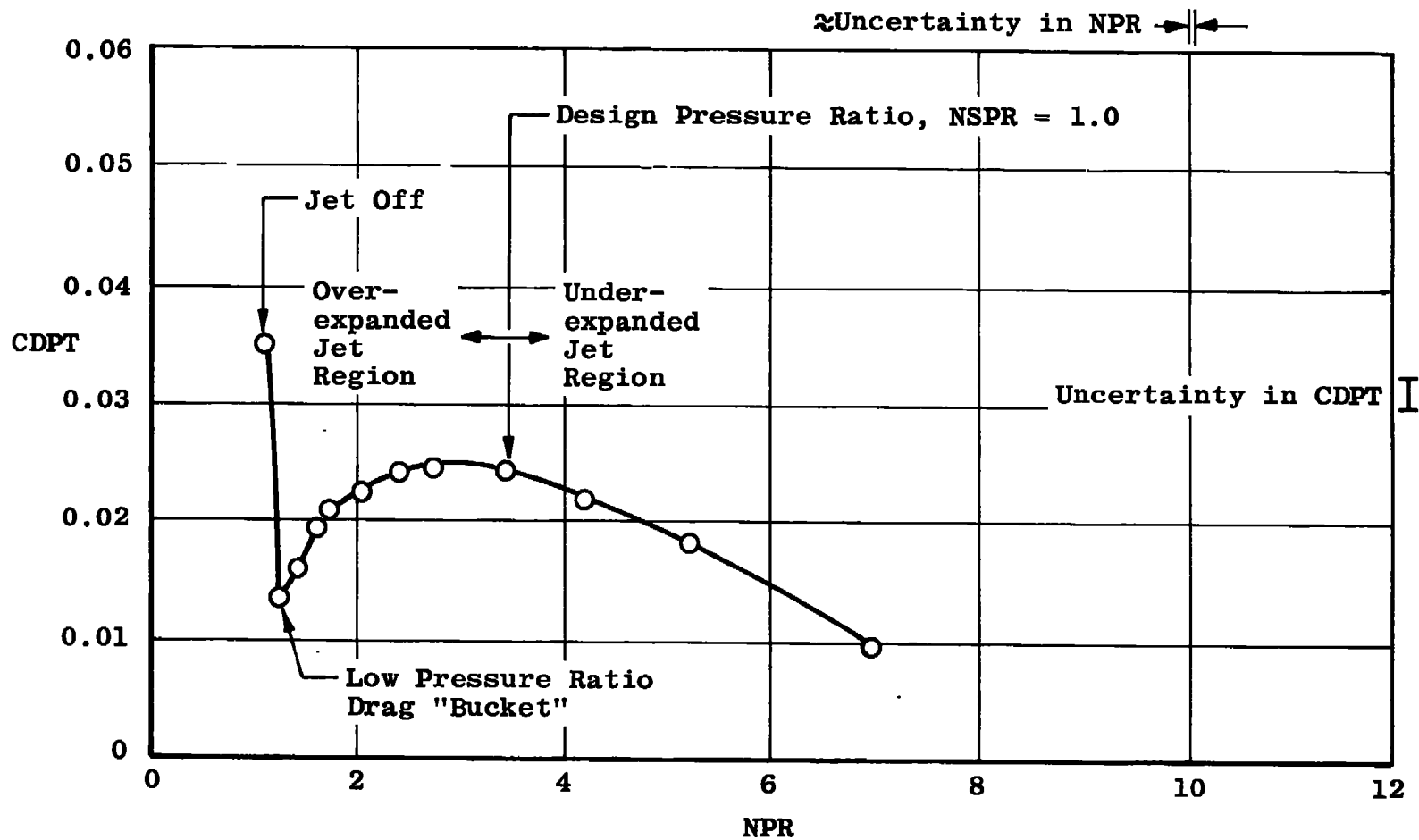
Figure 11. Typical variation of afterbody pressure drag with NPR.
