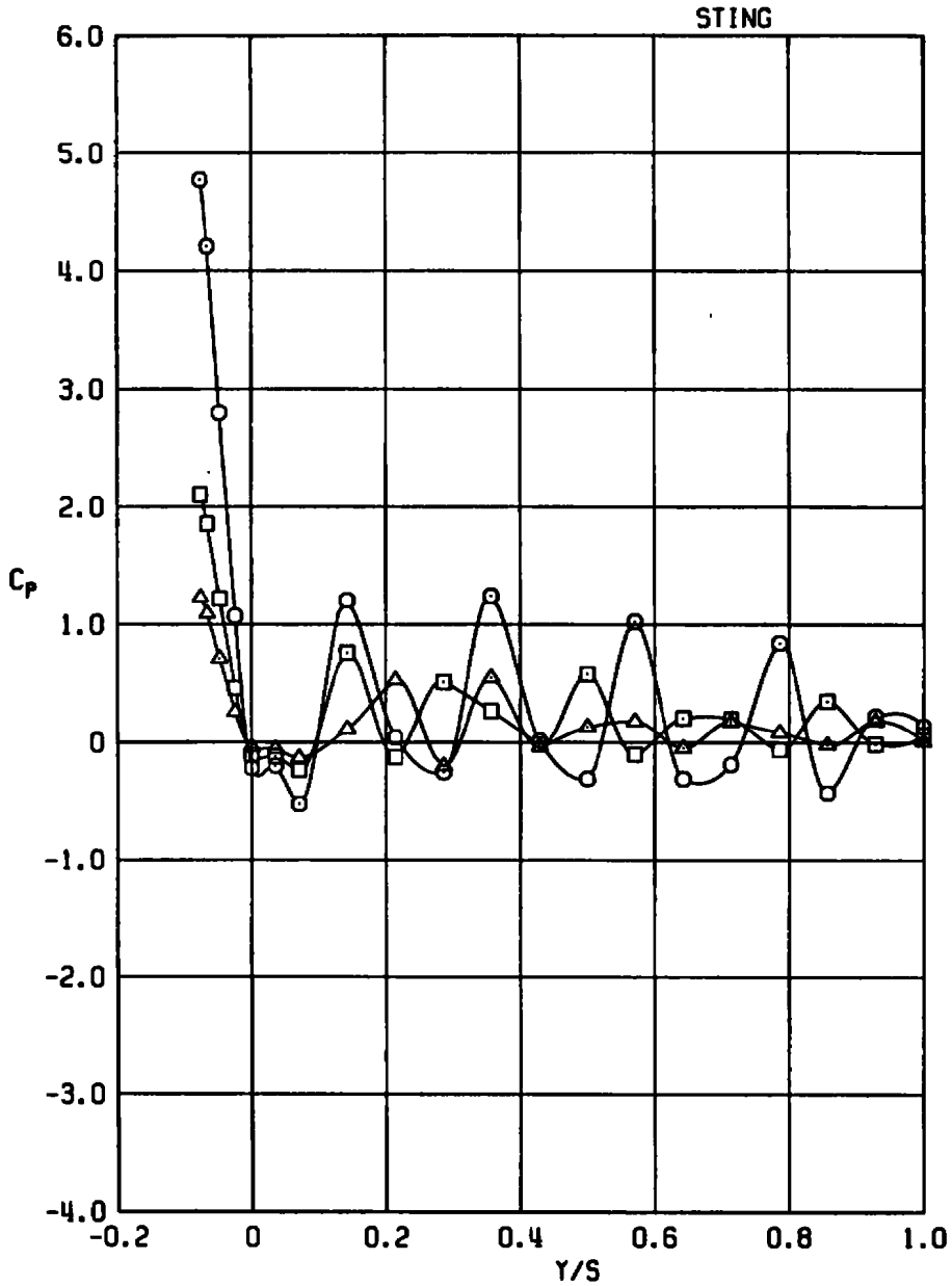
a. Sting pressure distributions, NSPR \approx 1.0 Figure 28. Free-stream Mach number effects on exhaust plume characteristics, D_g/D_N = 0.543 , A/A^* = 1.134 .
