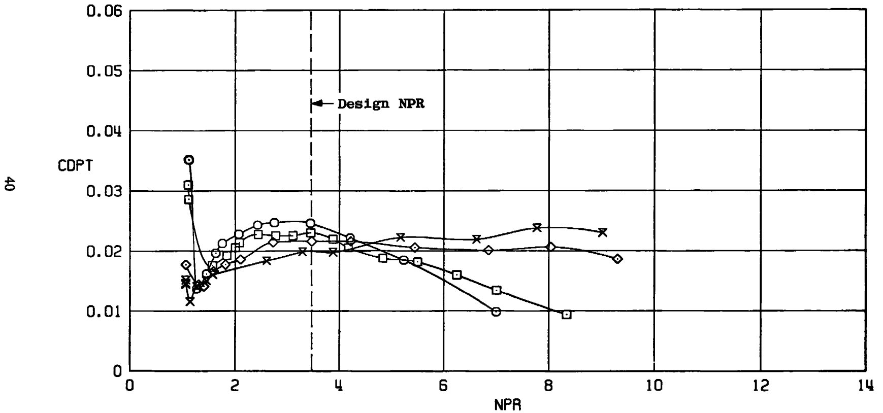
a. M_\infty = 0.6 Figure 13. Sting size effects on afterbody drag, A/A^* \approx 1.13 .
