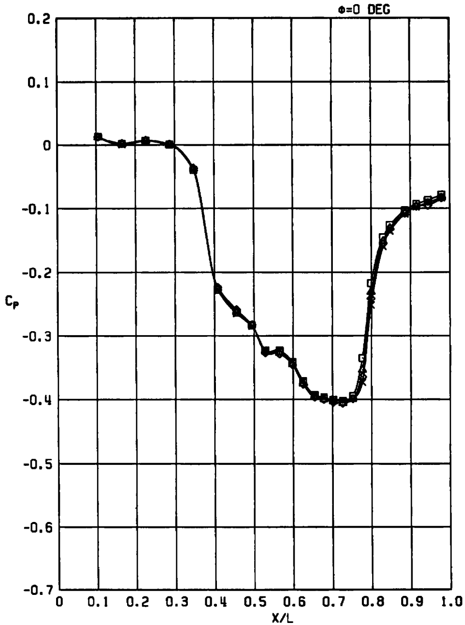
Figure A-11. Concluded.
