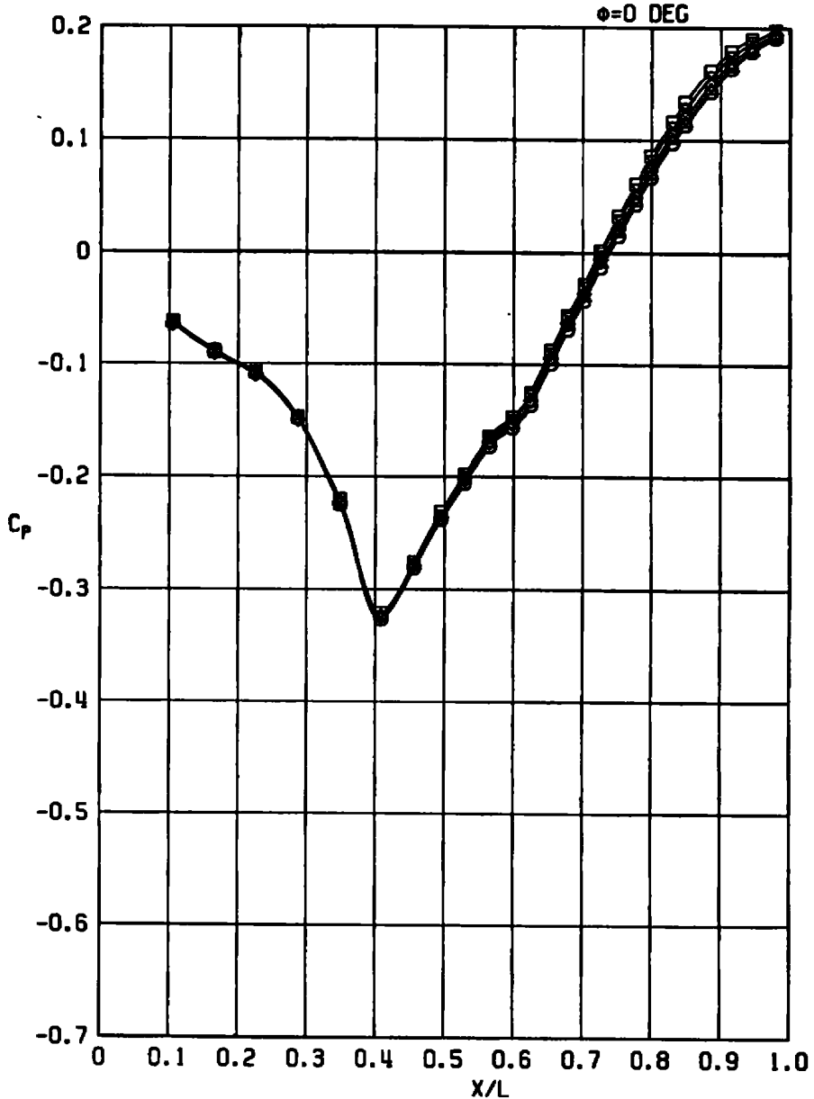
a. M_\infty = 0.6 Figure A-4. Effects of nozzle pressure ratio, D_s/D_N = 0.707, A/A^* = 1.491 .
