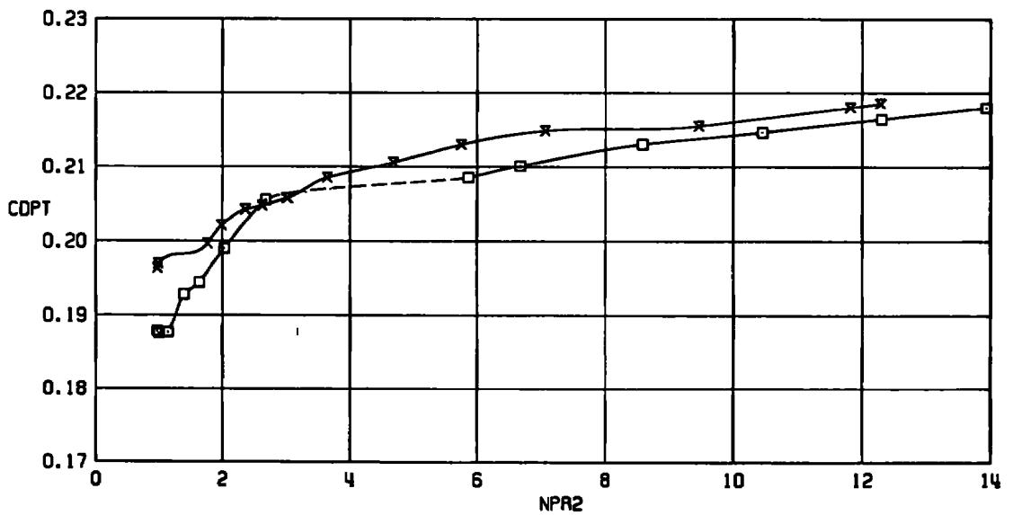
c. M_\infty = 1.2 Figure 43. Concluded.
