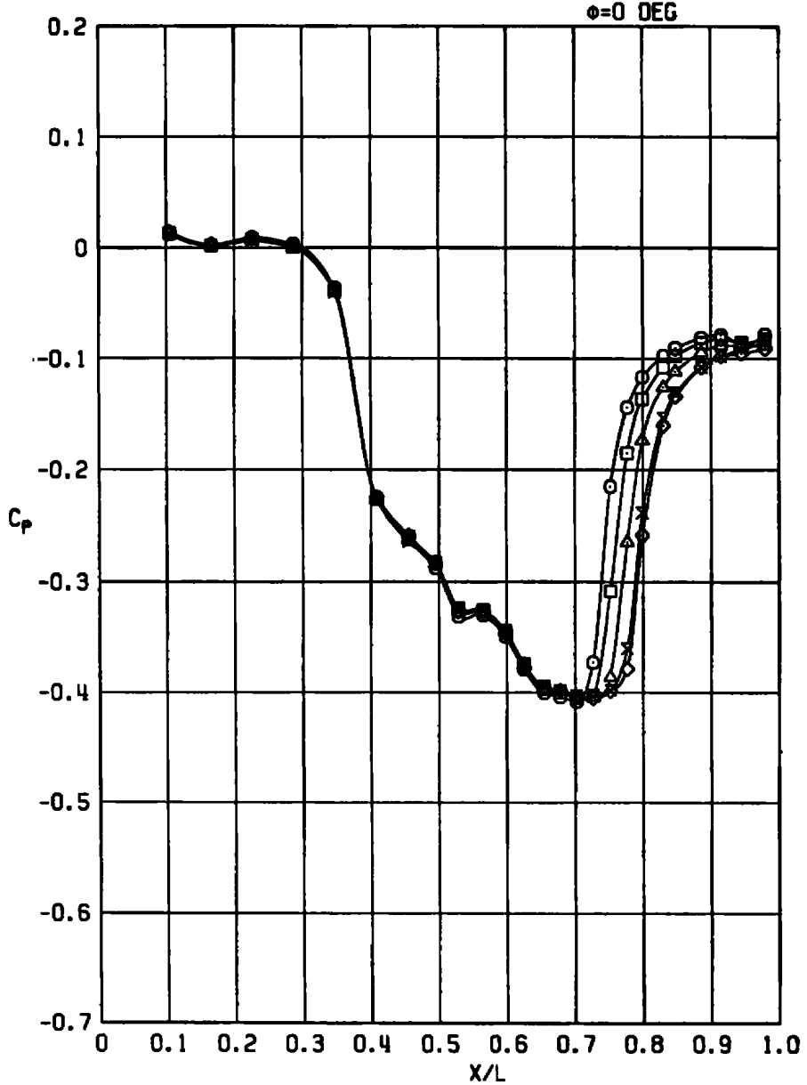
Figure A-8. Concluded.
