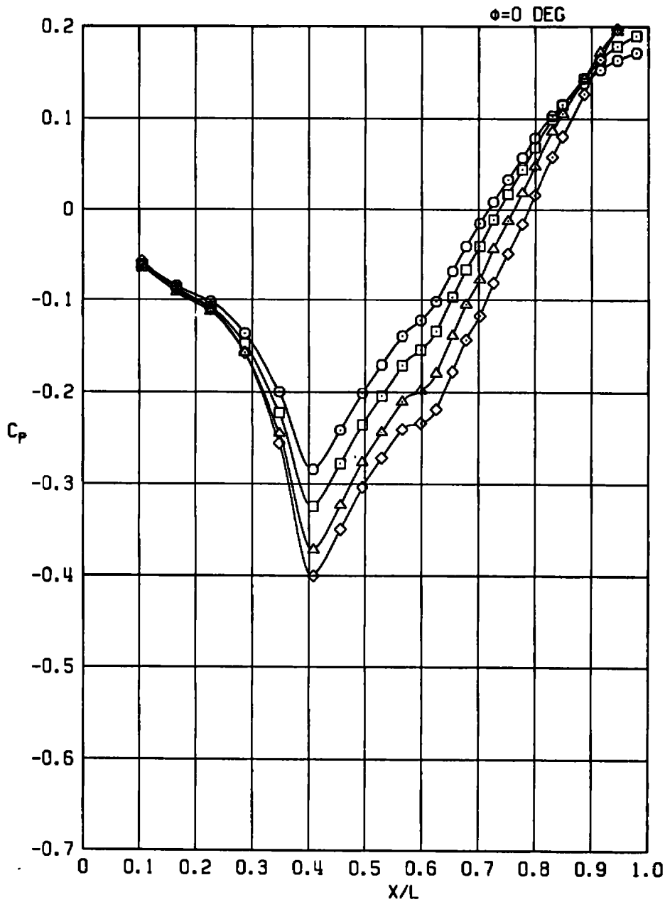
a. M_\infty = 0.6 Figure A-18. Effects of angle of attack, D_s/D_N = 0.707 , A/A^* = 1.491 , NSPR \approx 1.0 .
