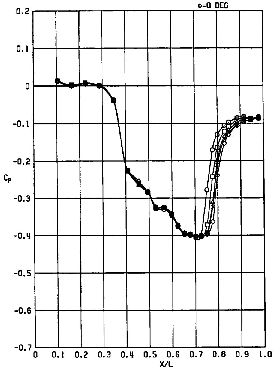
c. M_\infty = 1.2 Figure A-6. Concluded.
