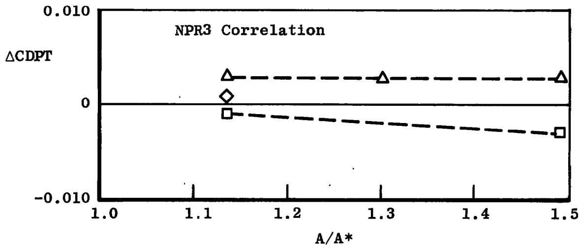
b. M_\infty = 0.9 Figure 37. Continued.
