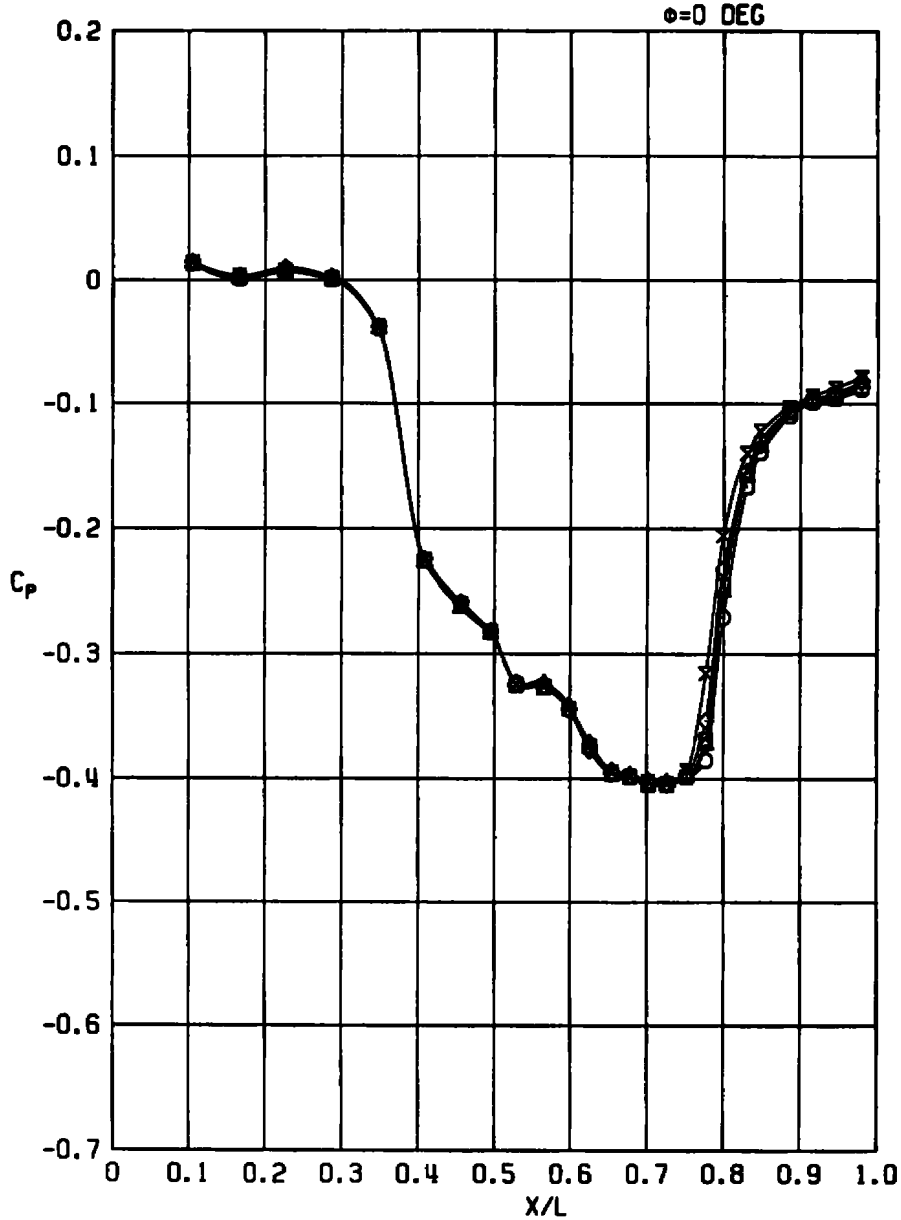
Figure A-7. Concluded.
