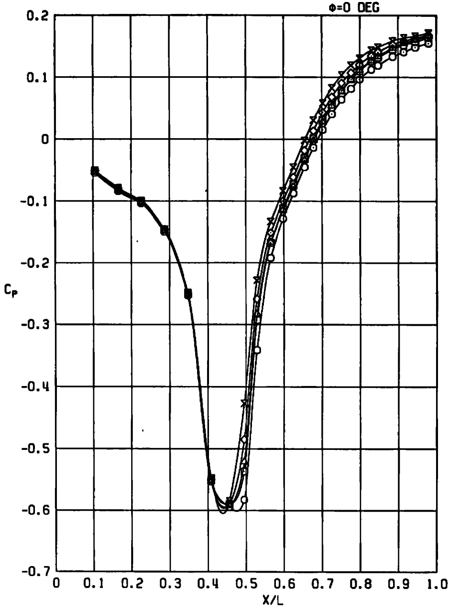
b. M_\infty = 0.9 Figure A-2. Continued.
