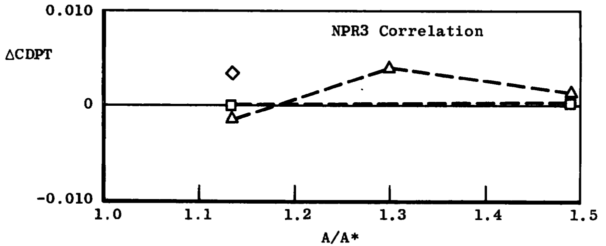
c. M ∞ = 1.2 Figure 37. Concluded.
