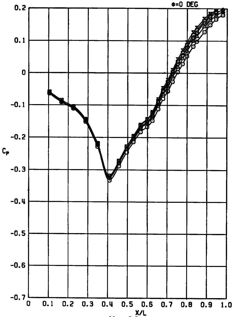
a. M_\infty = 0.6 Figure A-1. Effects of nozzle pressure ratio, D_s/D_N = 0, A/A^* = 1.134.
