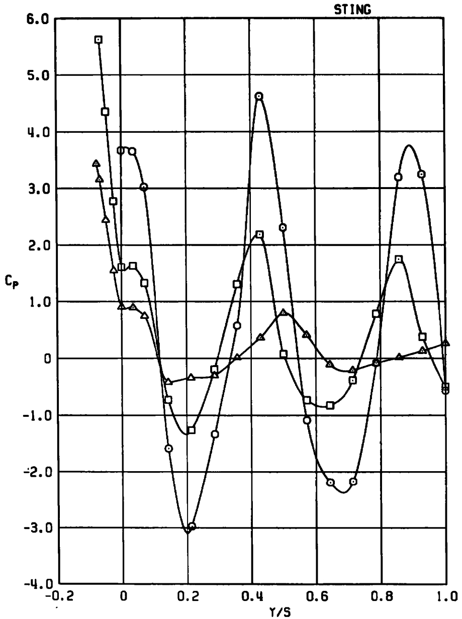
b. Sting pressure distributions, NSPR ≈ 2.0 Figure 28. Continued.
