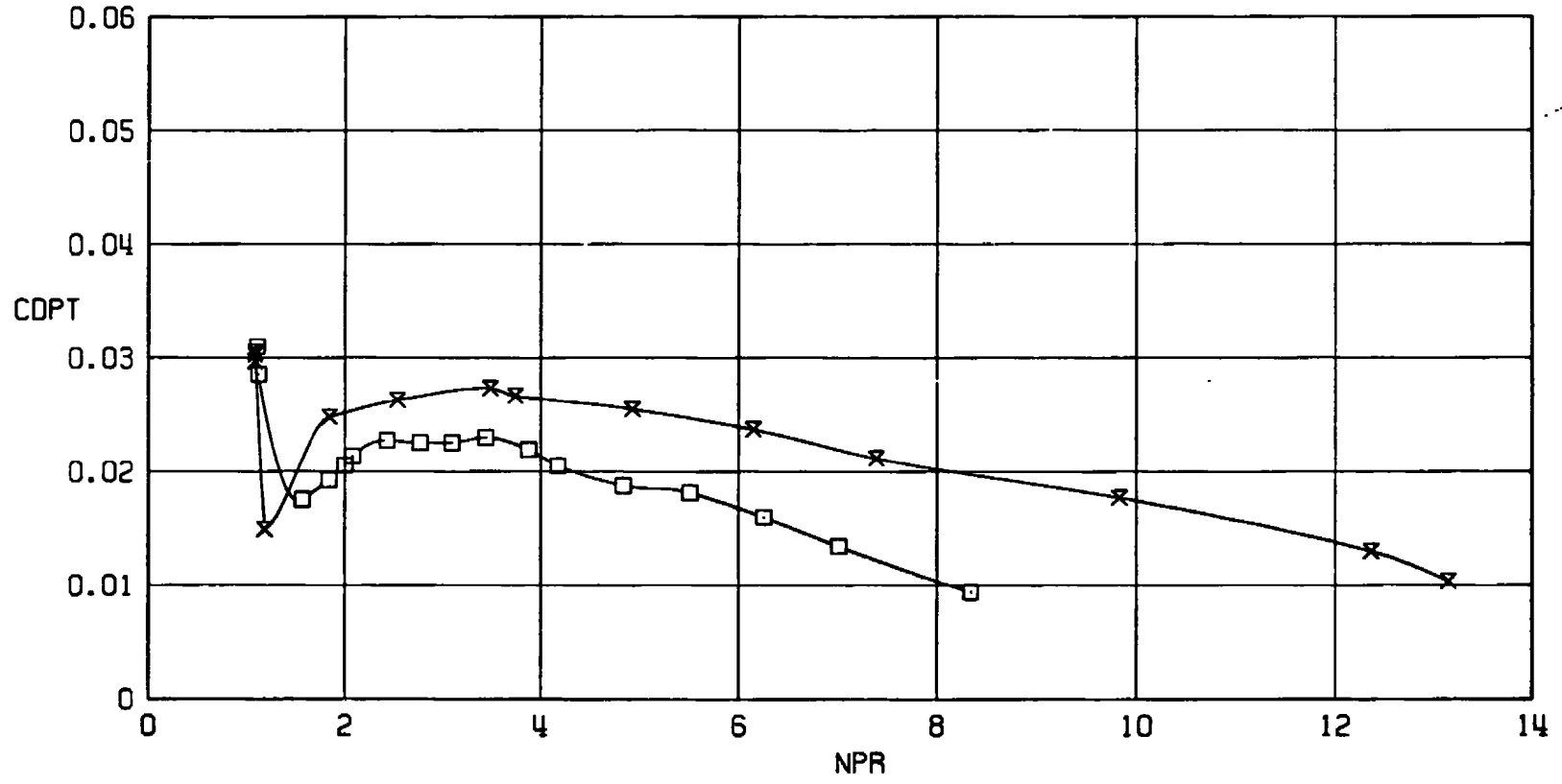
a. M_\infty = 0.6 Figure 19. Nozzle area ratio effects on afterbody drag, D_s/D_N = 0.543 .
