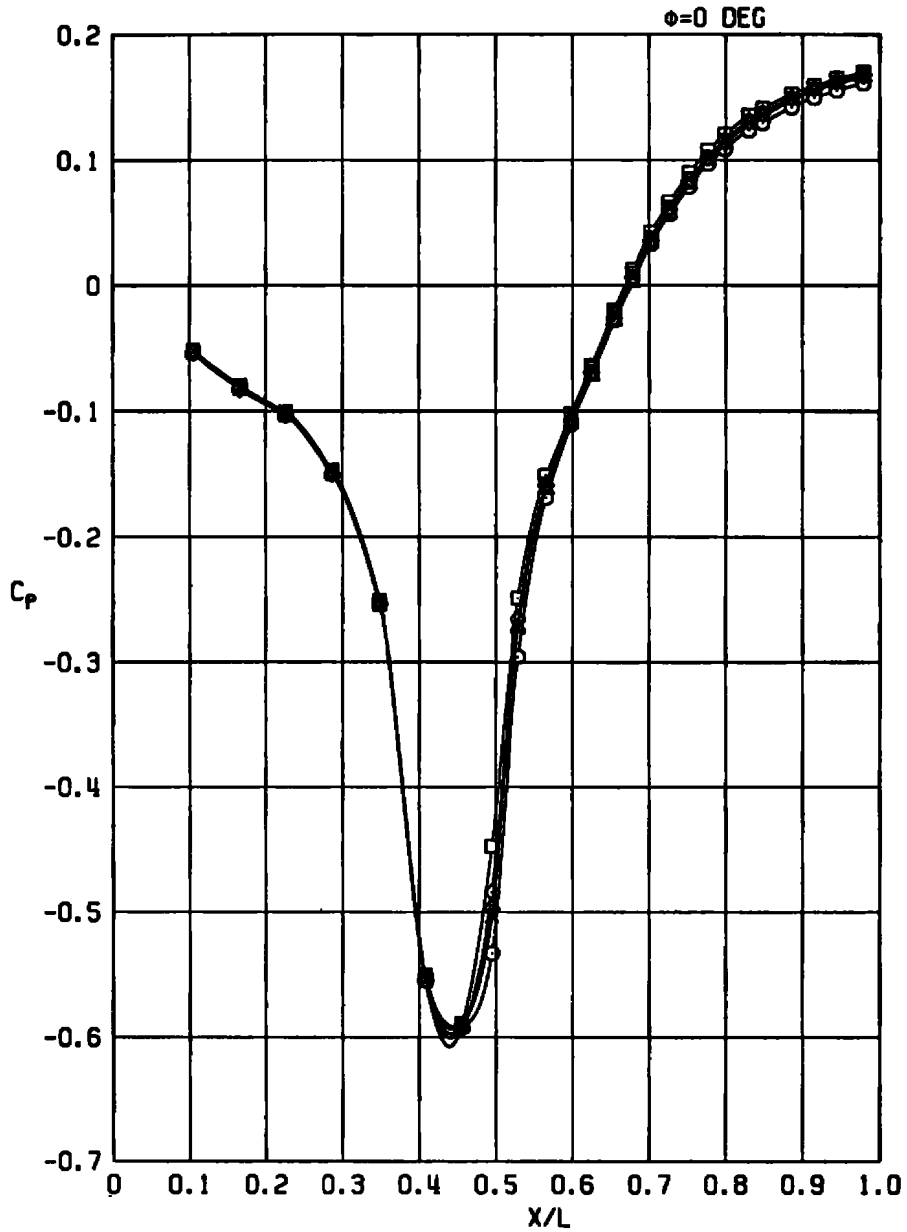
Figure A-3. Effects of nozzle pressure ratio, D_3/D_N = 0.707 , A/A^* = 1.133 .
