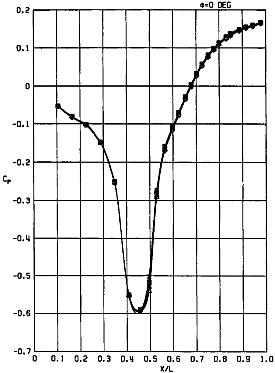
b. M_\infty = 0.9 Figure A-7. Continued.
