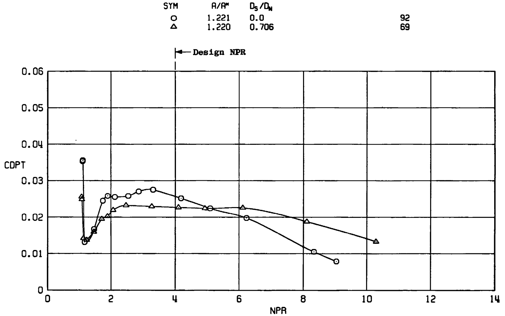
a. M_\infty = 0.6 Figure 14. Sting size effects on afterbody drag, A/A^* \approx 1.22 .
