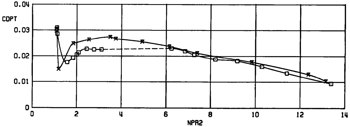
Figure 40. Correlation of nozzle area ratio effects on afterbody drag, D_s/D_N = 0.543 .
