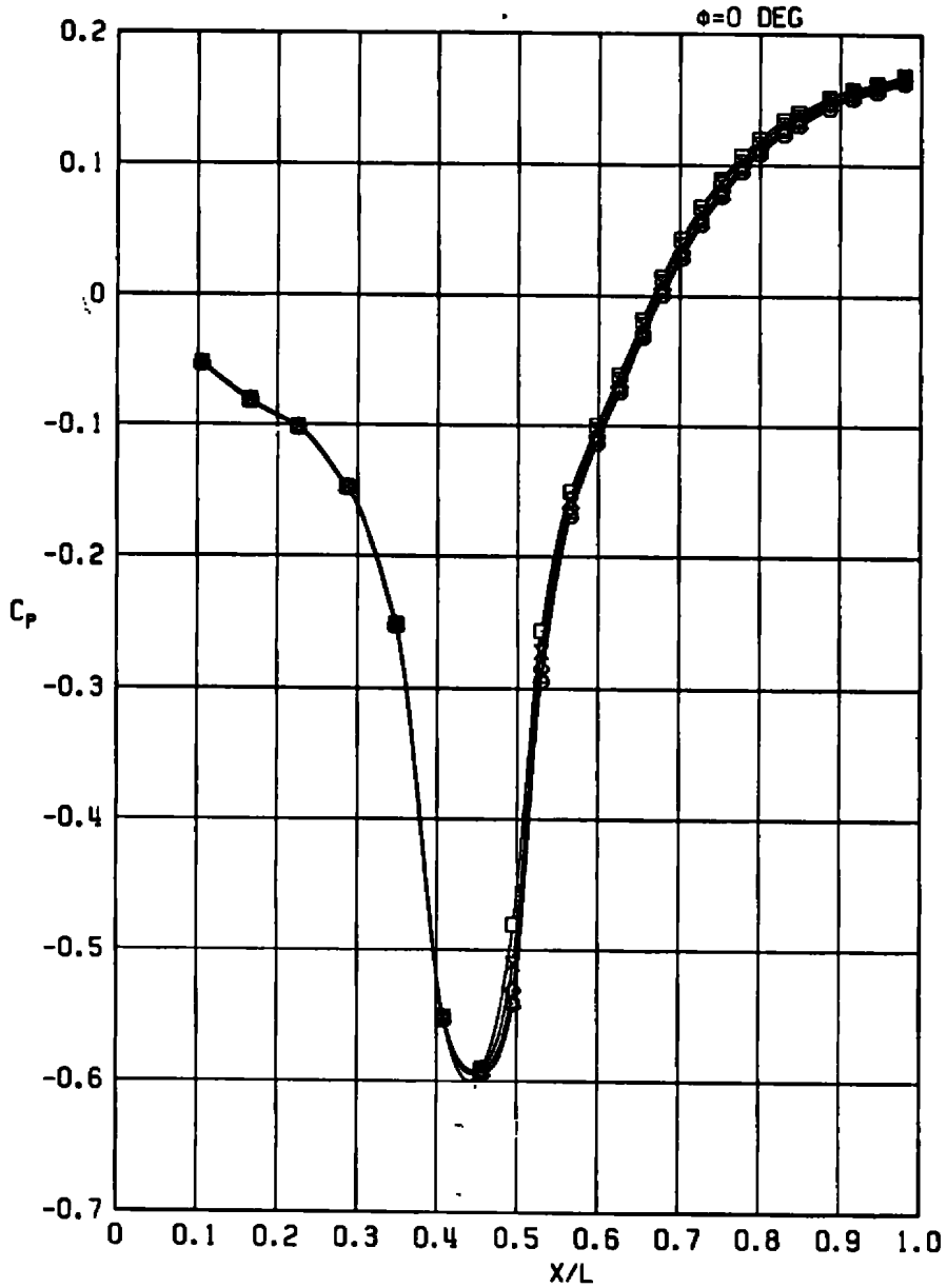
b. M_\infty = 0.9 Figure A-4. Continued.
