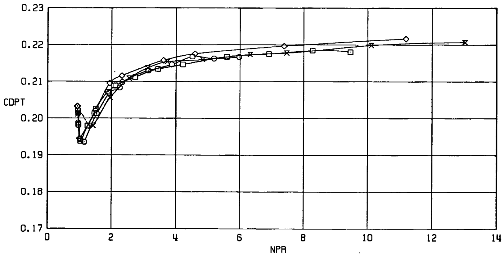
c. M_\infty = 1.2 Figure 21. Concluded.
