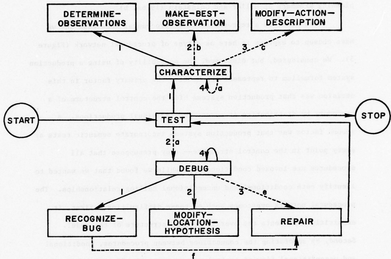
Figure 5. Procedural network for the top-level structure of a general strategy for troubleshooting/debugging.
