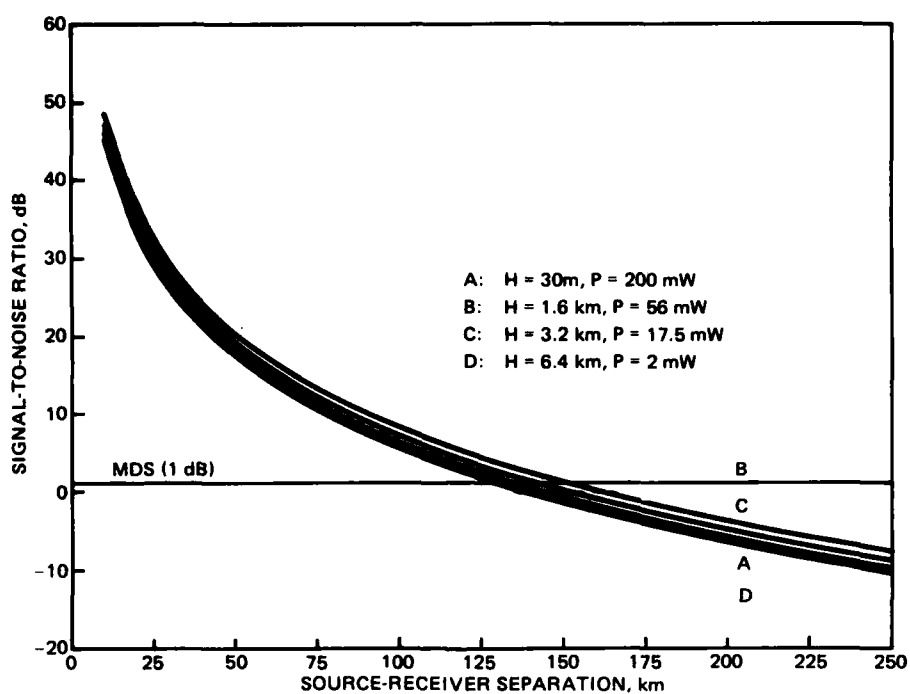
Figure 57. SNR vs range for a P-3 to enemy interception link. Receiver angular orientation (120^\circ, 0^\circ) .
