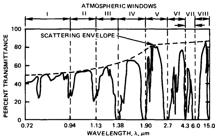
Figure 31. Transmissivity of the atmosphere. 16
