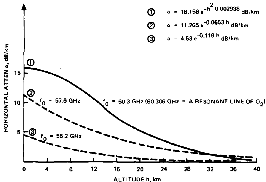
Figure 6. Horizontal attenuation vs altitude.
