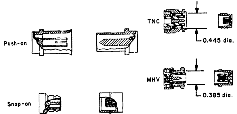
Figure 20. MHV-Type Connector
