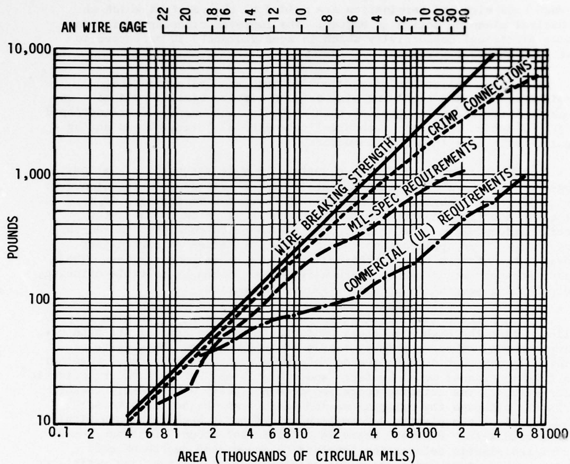
Figure 2. Tensile Strength of Wire and Wire Connections
