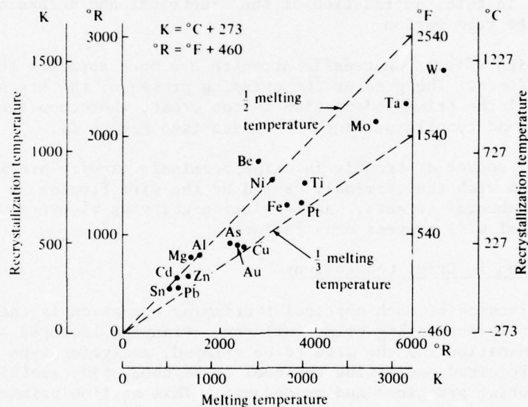
Figure 3. Metal Recrystallization Temperatures Compared with Melting Points
