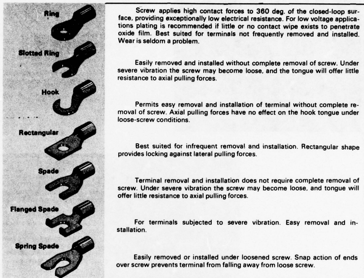
Figure 7. Common Terminal-Tongue Styles
