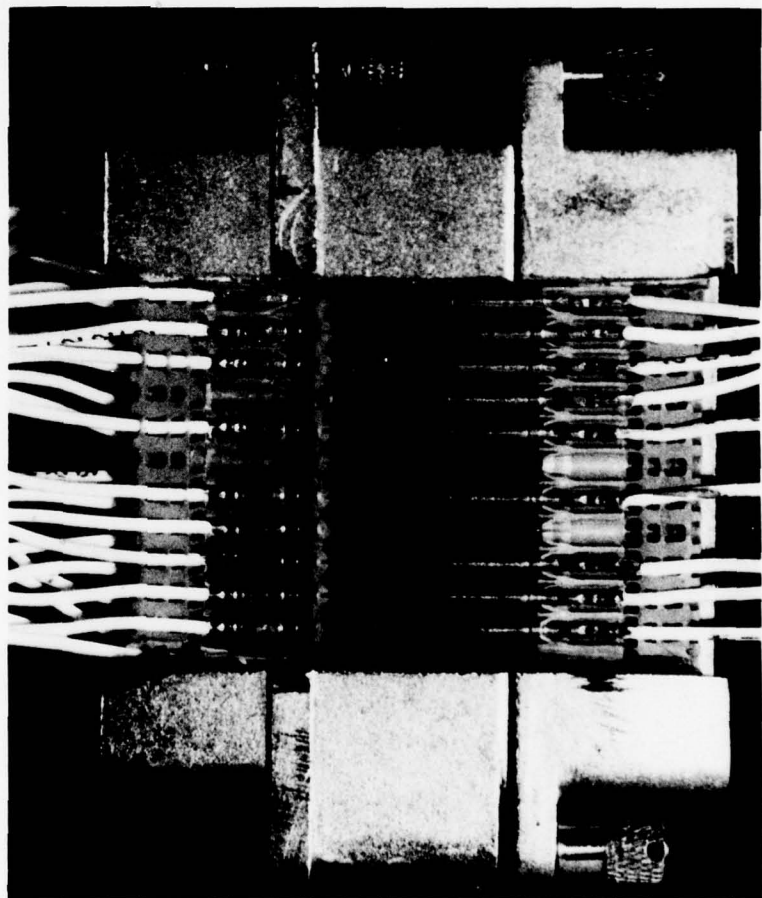
Figure 6. Cutaway View of Contacts Within a Connector
