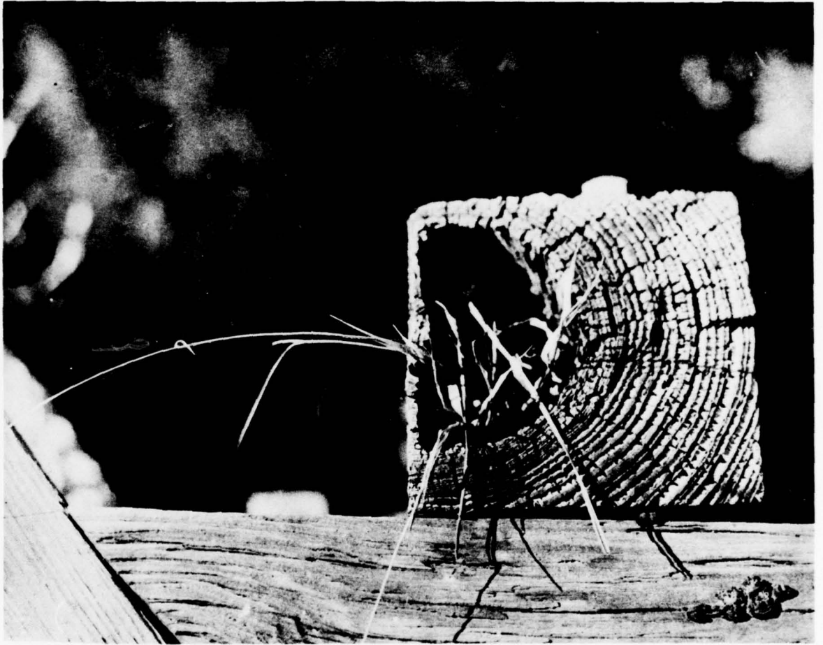
This southern pine bridge timber suffered heartwood decay. Because heartwood does not usually "treat" as easily as does the surrounding sapwood, the wide treated sapwood band on the right and the thin treated border of heartwood on the left have outlasted the untreated exposed heartwood core.
