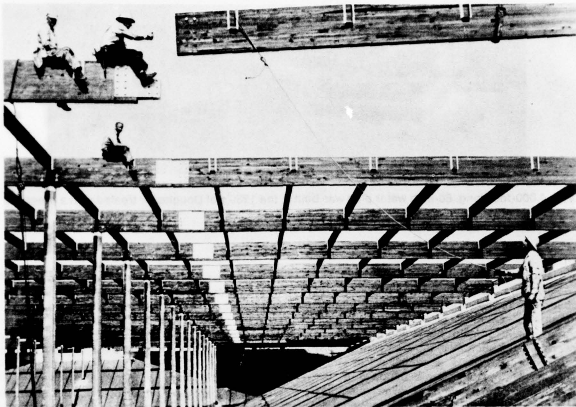
These pressure-treated laminated wood beams provide the supports for a roof over a 22-million-gallon reservoir near Pinole, Calif. Treatments vary for special uses, such as this one in contact with a supply of drinking water.
