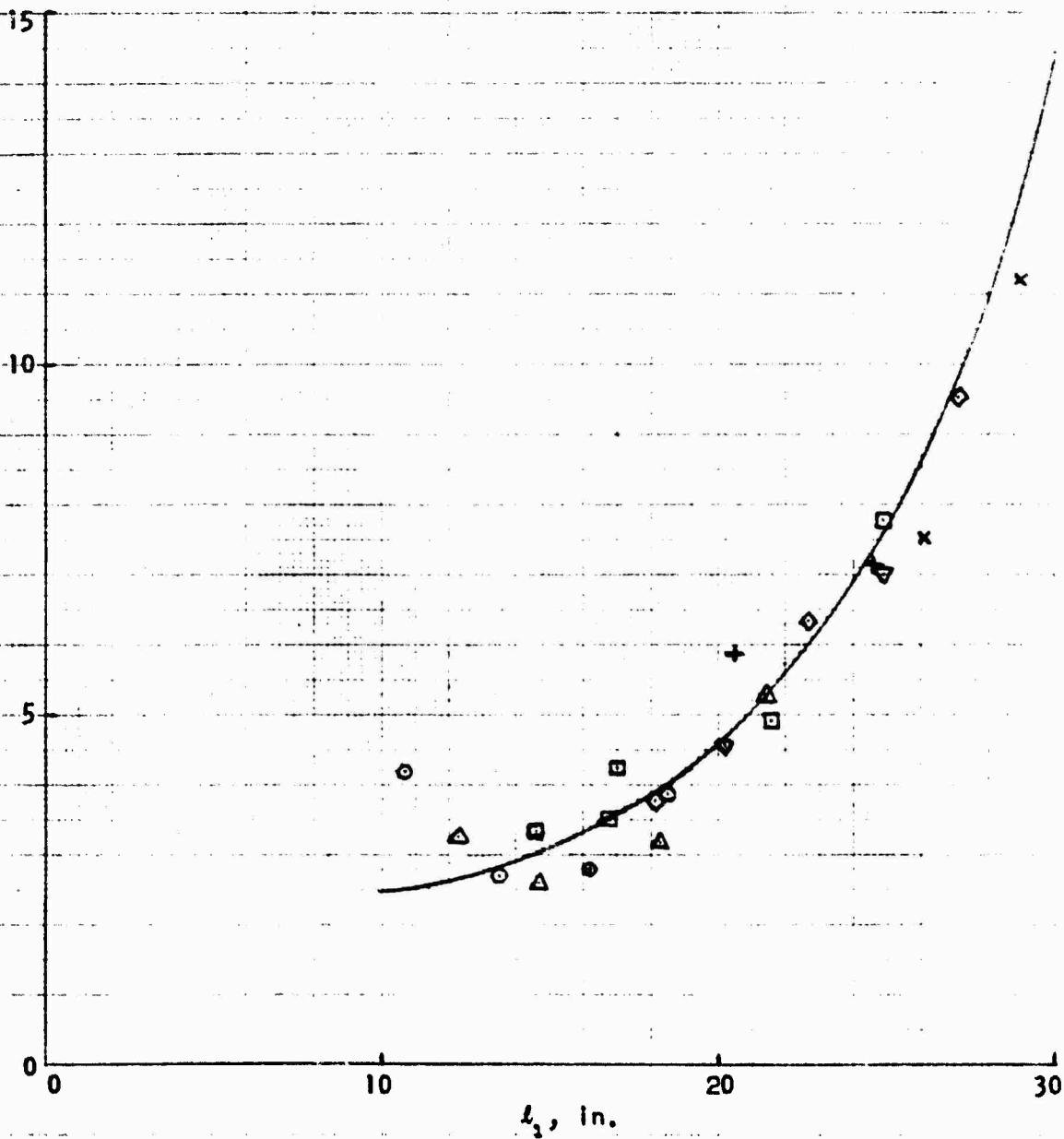
FIGURE A11 PARASITE DRAG LESS SKIN FRICTION DRAG AT 14.82 FPS
