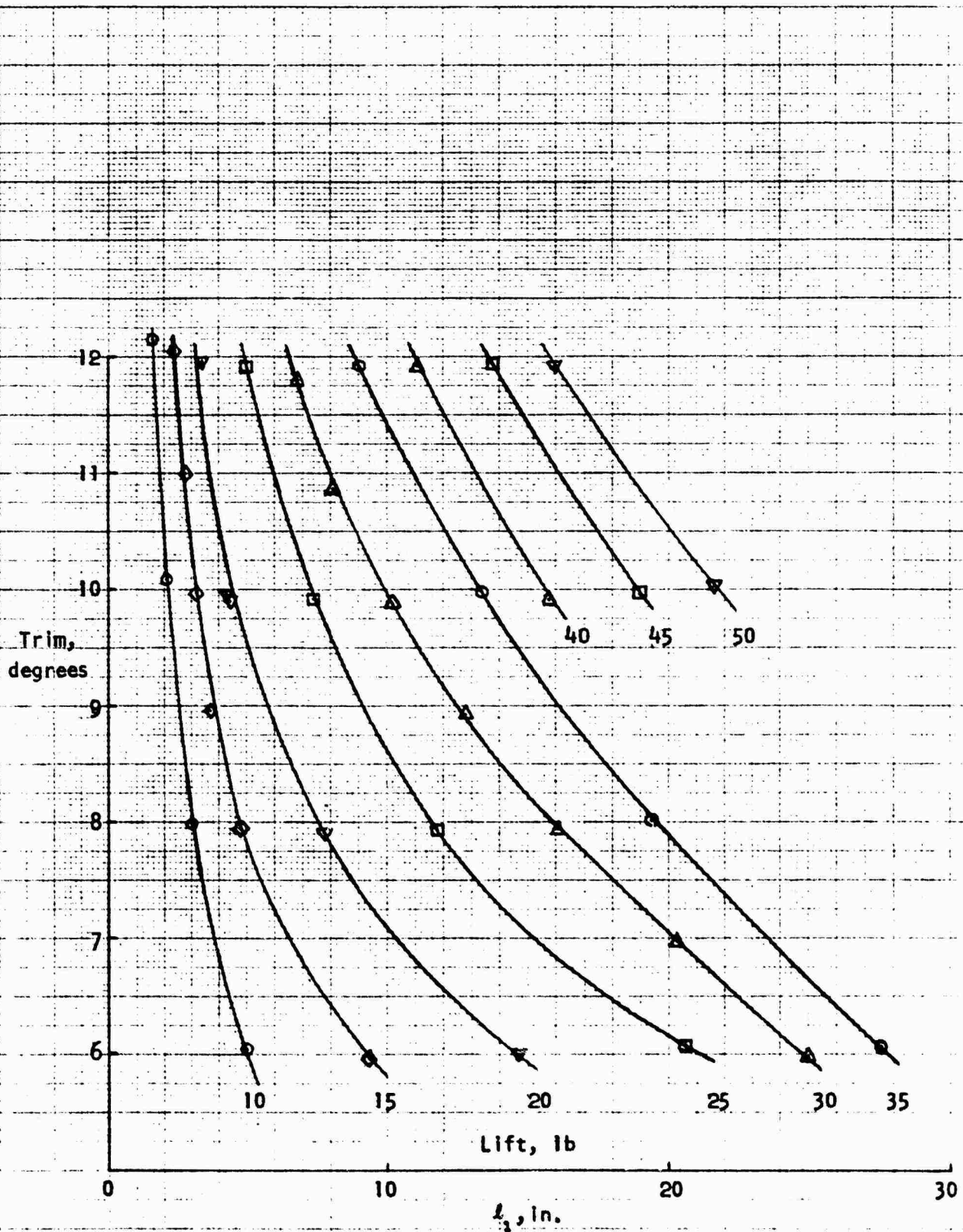
FIGURE A2 MODEL LIFT CHARACTERISTICS AT 14.82 FPS (35 mph)
