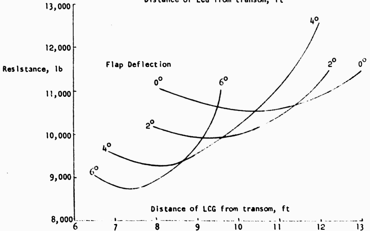
FIGURE 9 SEA STATE 2 ACCELERATION AND RESISTANCE CHARACTERISTICS AT 35 mph, 55,000 lb
