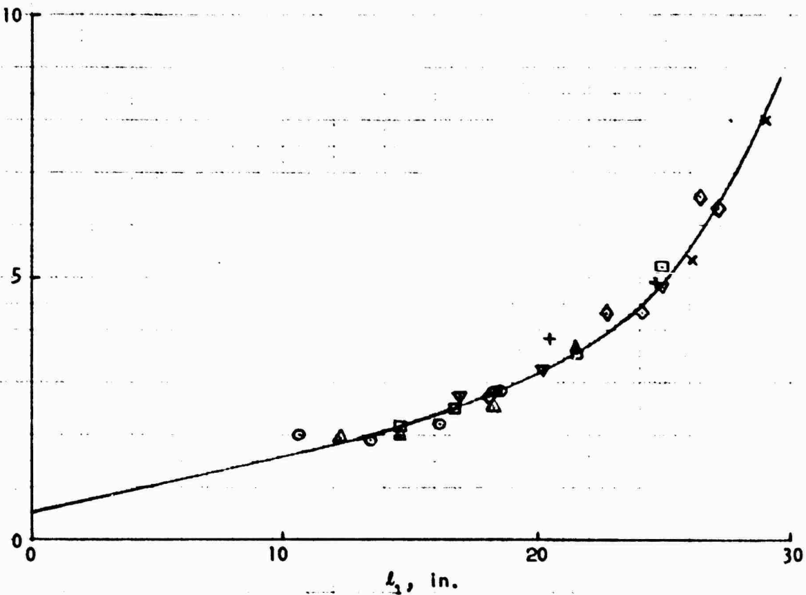
FIGURE A7 REMOVAL OF FLAP DRAG FROM TOTAL MODEL ROUGH WATER PARASITE DRAG AT 14.82 FPS
