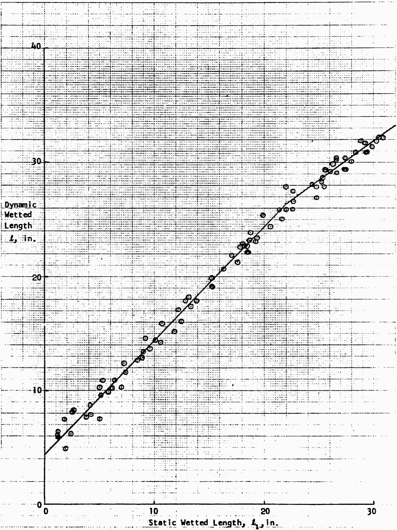
FIGURE A1 WETTED LENGTH CHARACTERISTICS
