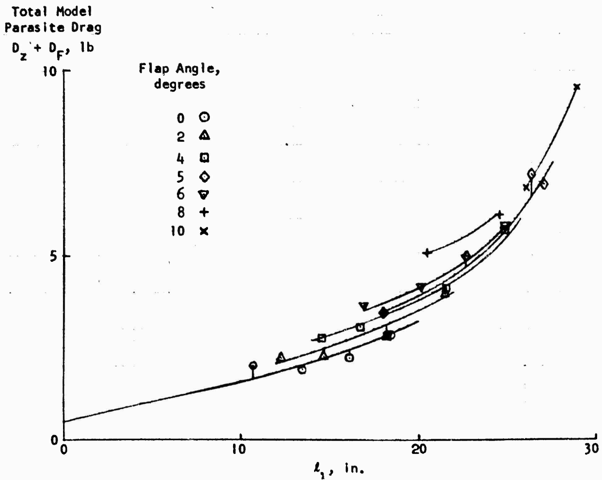
FIGURE A6 VARIATION OF PARASITE DRAG WITH WETTED LENGTH AND FLAP ANGLE AT 14.82 FPS
