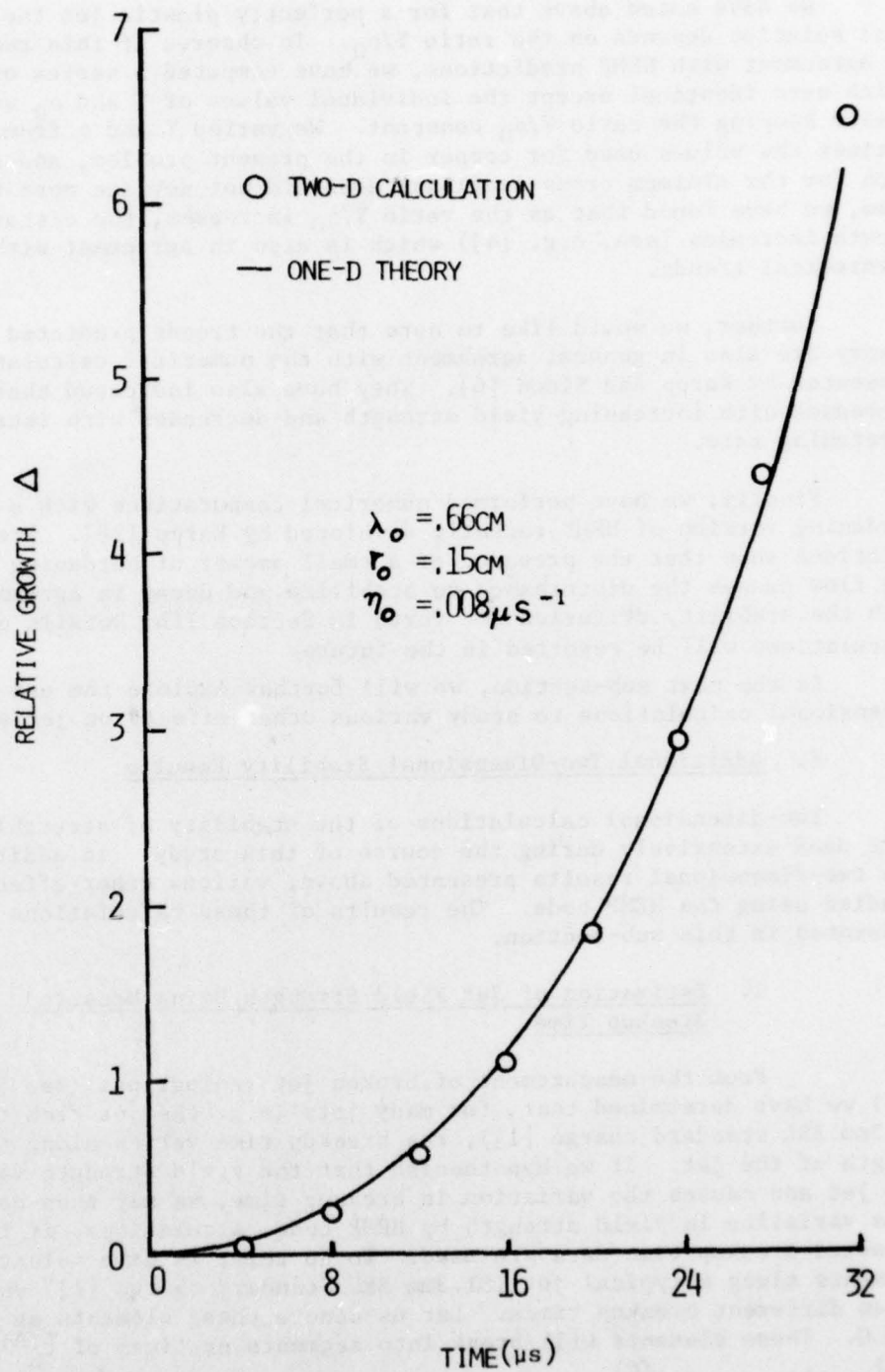
Figure 4. Comparison of relative growth versus time for one-dimensional theory and two-dimensional calculations with \eta_o = .008 \mu s^{-1} .
