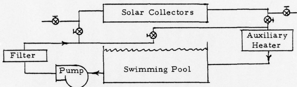
Fig. 13. Solar Swimming Pool Heater Schematic
