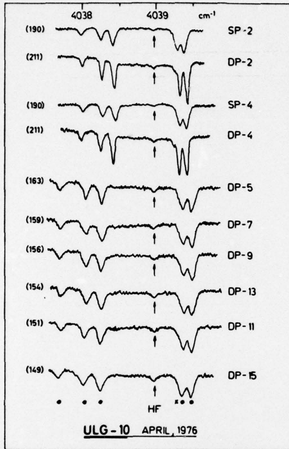
Fig. 1. Solar spectra near 4039 \text{ cm}^{-1} , taken from 27.9 km altitude, at various solar zenith angles (linear ordinate deflections).
