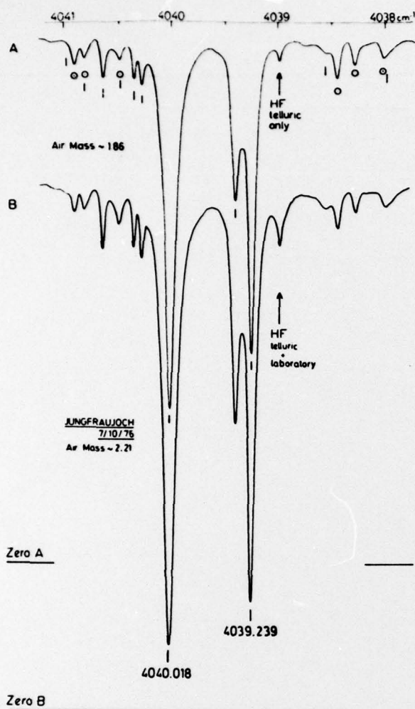
Fig. 2. Two solar spectra ranging from 4041 to 4038 \text{cm}^{-1} , as observed at the Jungfrauoch Station (linear ordinate deflections).
