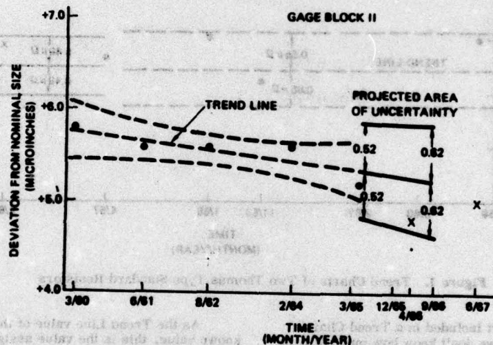
Figure 2. Trend Charts of Two Gage Blocks
