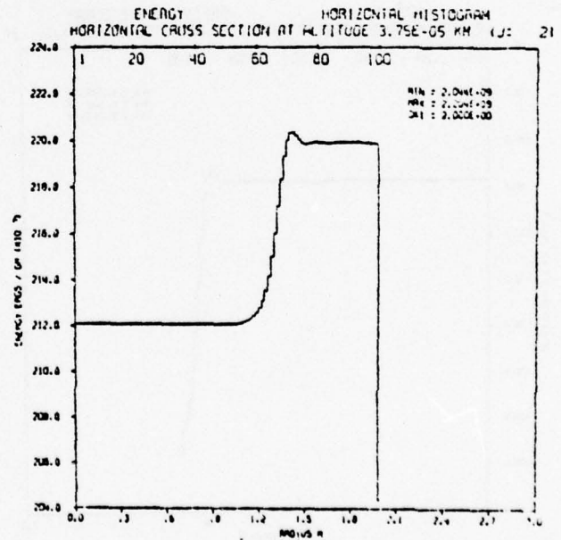
Figure 8. AFWL - 2 psi Square Wave on Wall - Large Quadratic Viscosity Time - 4.8 msec, Problem 19.8011A.
