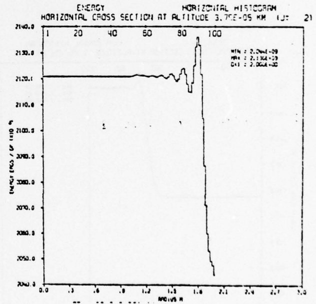
Figure 3. AFWL - 2 psi Square Wave on Wall - STABF = 0.05 Time - 2.5 msec, Problem 19.8011.
