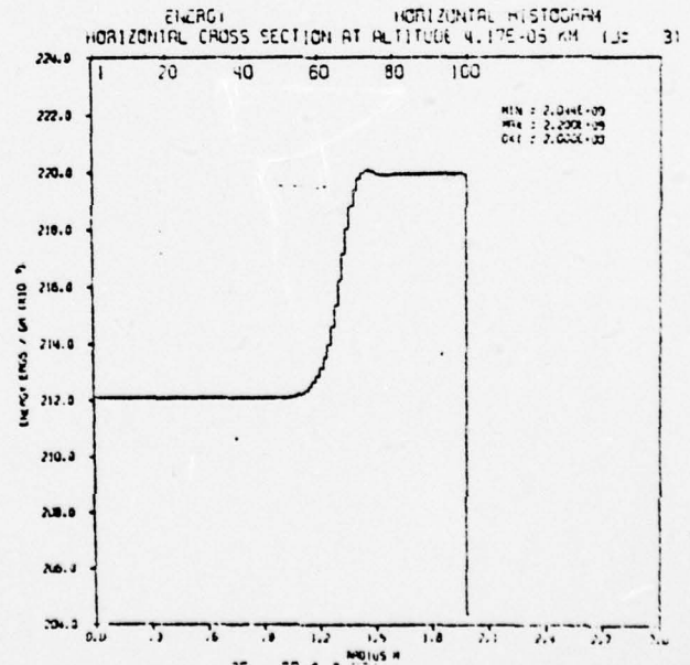
Figure 14. AFWL - 2 psi Square Wave on Wall - Viscosity Function Time - 4.8 msec, Problem 19.8012B.
