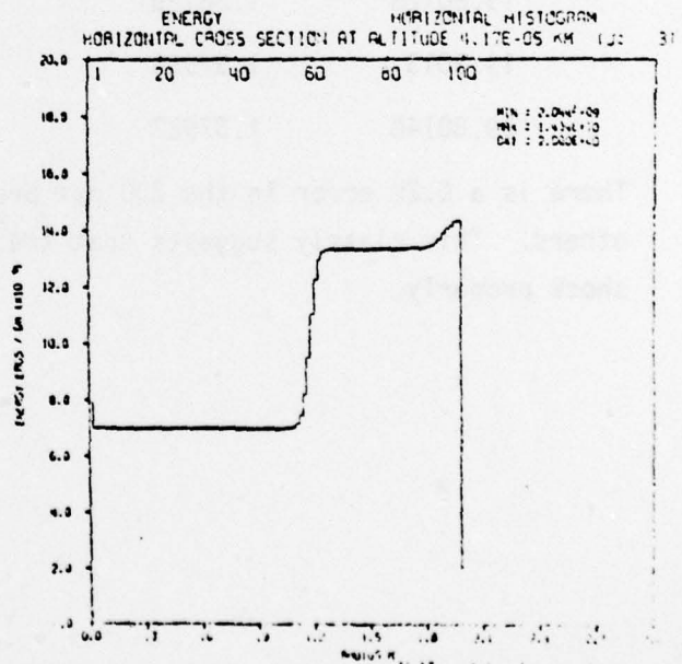
Figure 22. AFWL - 200 psi Square Wave on Wall - Viscosity Function Time - 2.5 msec, Problem 19.80148.
