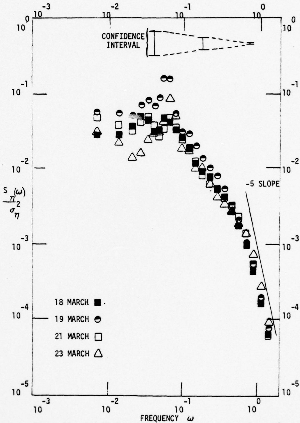
Figure 11. Sea Surface Elevation spectra at Wave Gauge #3
