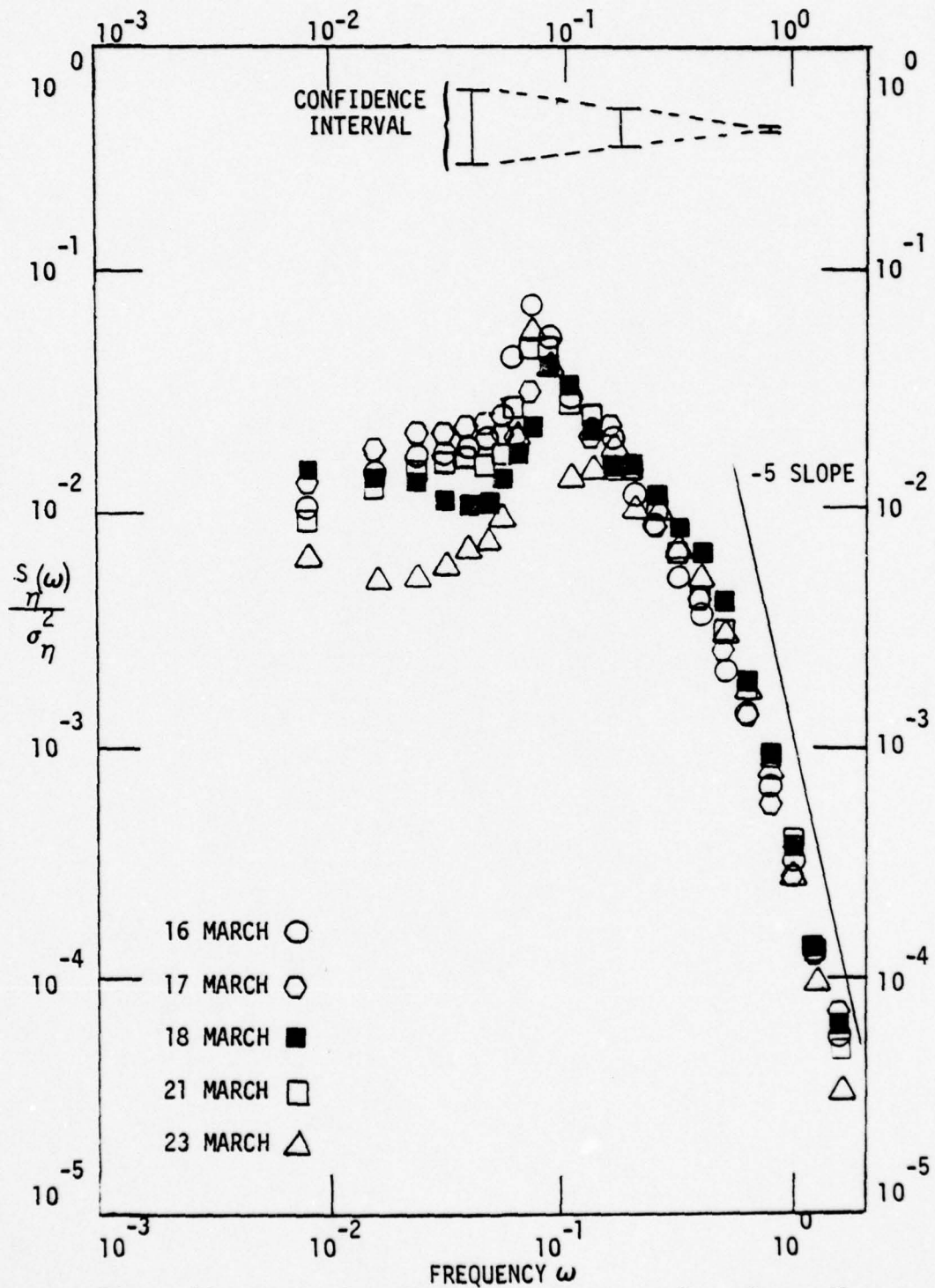
Figure 10. Sea Surface Elevation spectra at Wave Gauge #1.
