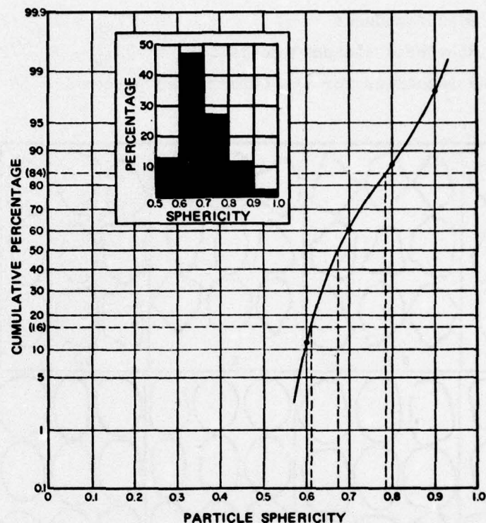
Figure A3. Histogram and cumulative curve of sphericity distribution of river pebbles. The dashed lines show the 16th, 50th, and 84th percentiles on the cumulative probability graph (after Krumbein and Sloss 45 )
