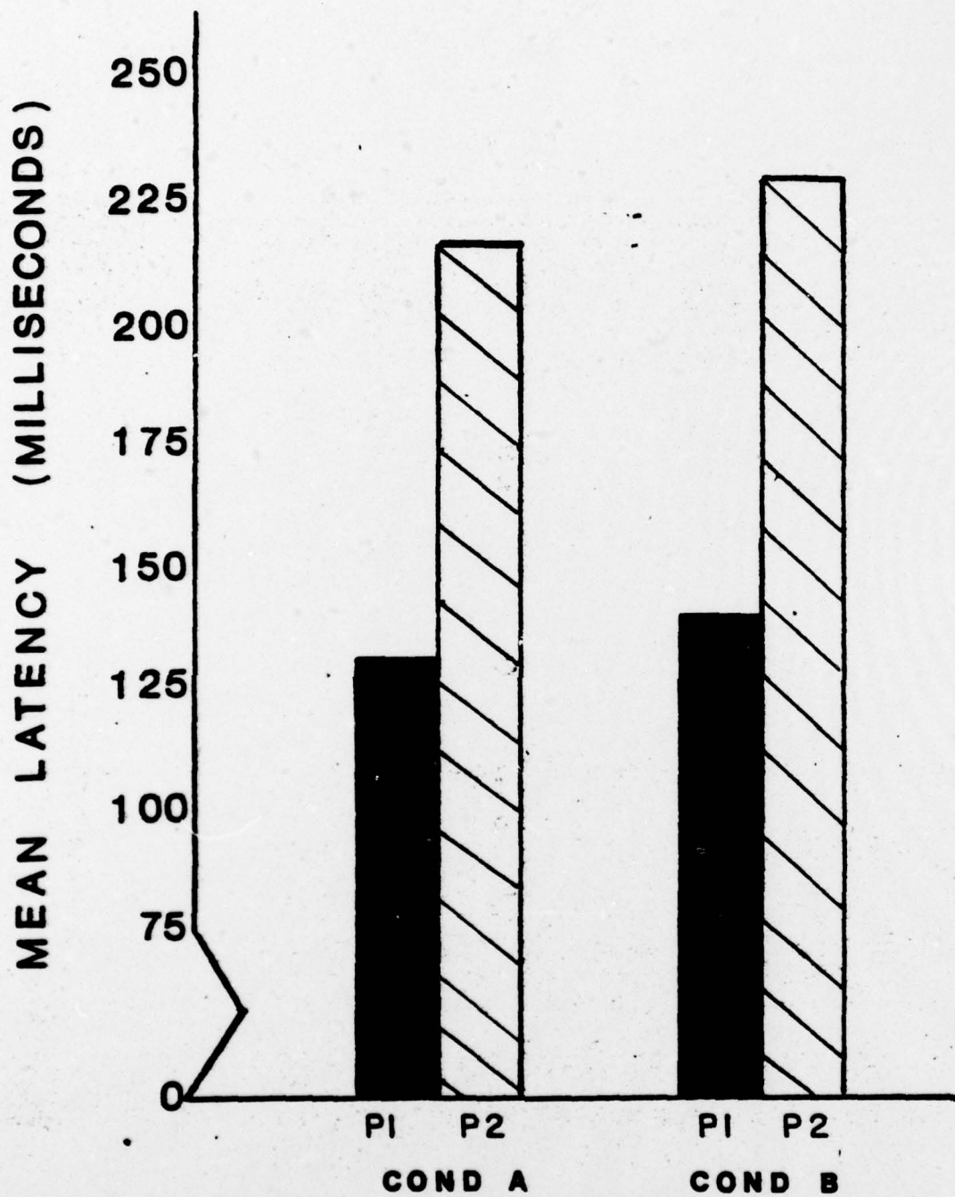
Figure 4- Mean latency for VEP components P1 and P2 under conditions A and B at O_2 (10 Sa).
