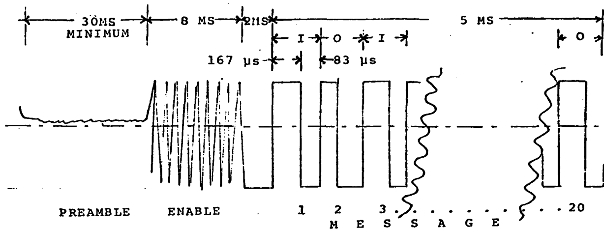
FIGURE C.1.1.4. Input to decoder, output from portable command transmitter (PCT).
