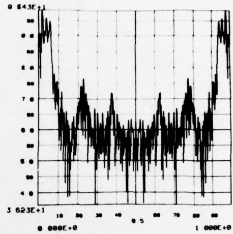
(b) Spectrum of input speech
