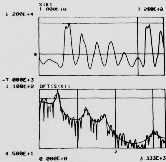
Figure 1: Example frame used as s(k) a) 128 samples of the vowel /ə/, sampled at 6667. Hz. b) Spectrum of /ə/ and a 10 pole LPC fit to that spectrum.
