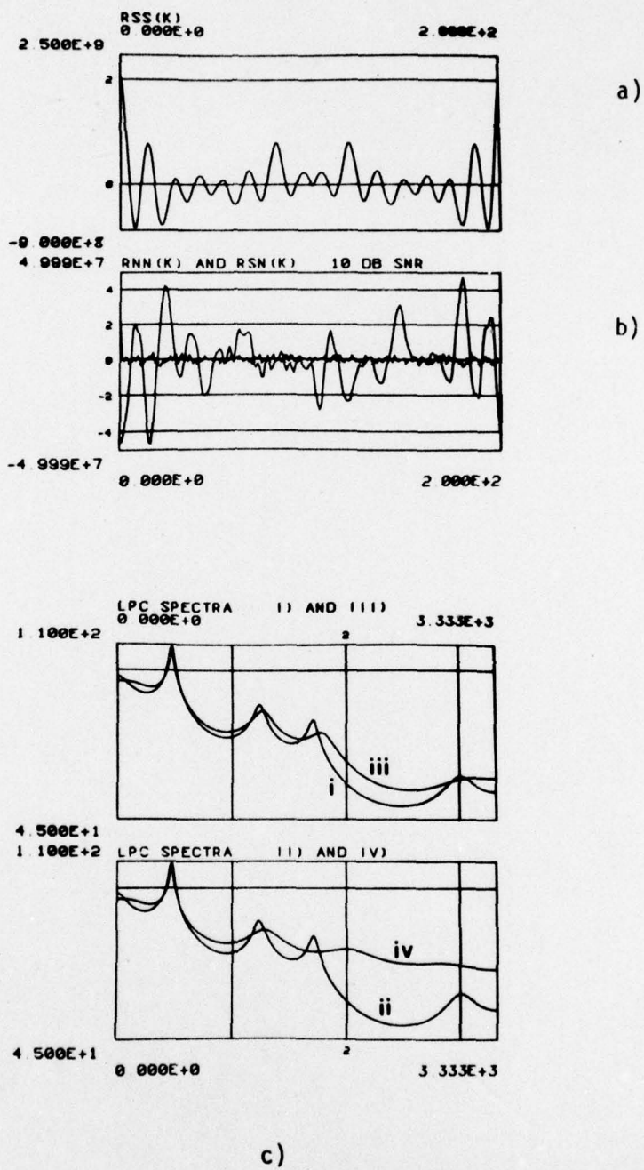
Figure 3: Comparison of autocorrelation and crosscorrelation sequences for the sample frame with a 10 dB SNR. a) R_{ss}(k) b) R_{nn}(k) and R_{sn}(k) c) 10 pole LPC spectra based on autocorrelations i-iv discussed in text.
