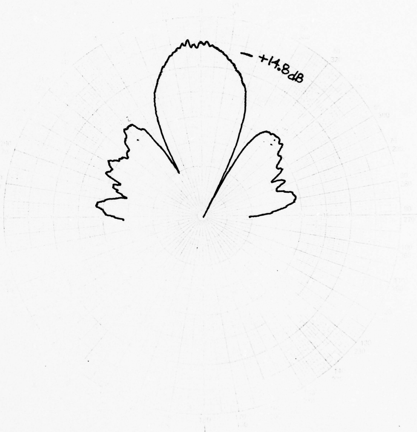
Figure 4-3 E-Plane Radiation Pattern (36.6 GHz) Coax Fed
