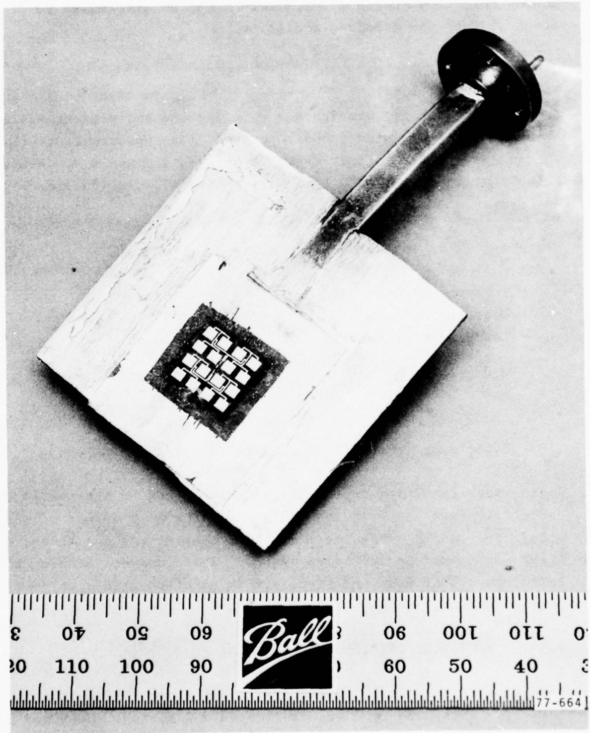
Figure 4-7 Waveguide Probe Fed Array (Front View)
