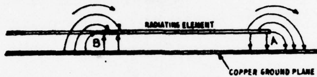
Figure 1-2 Electric Field in Vicinity of Microstrip Element
