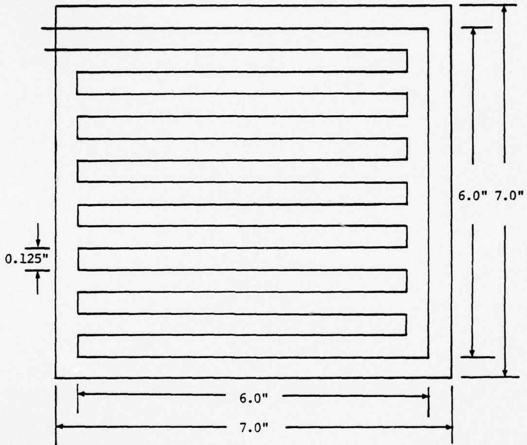
FIGURE 4. Heater Element
