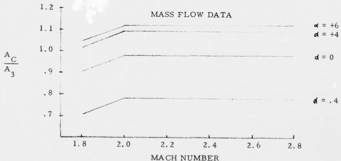
Figure 5 Pressure Recovery and Mass Flow Data
