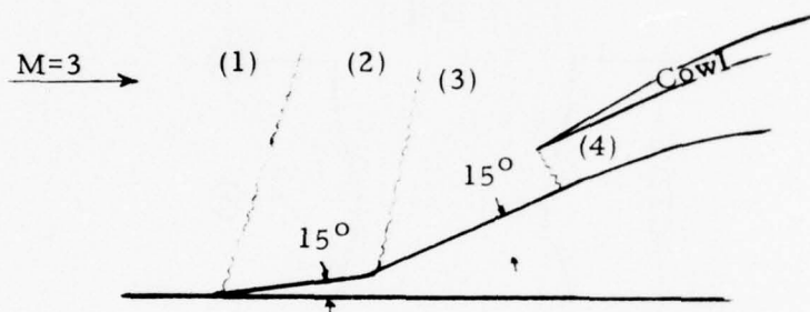
FIG. 2 Two-dimensional diffuser
