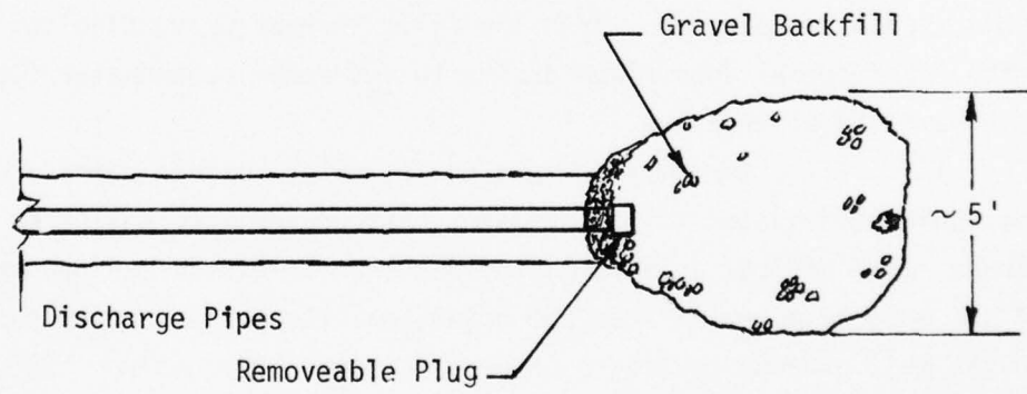
Figure 8. Leachate collection sump
