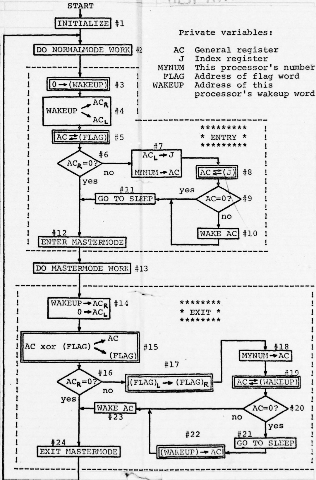
Figure 9. Flowchart of Solution Algorithm
