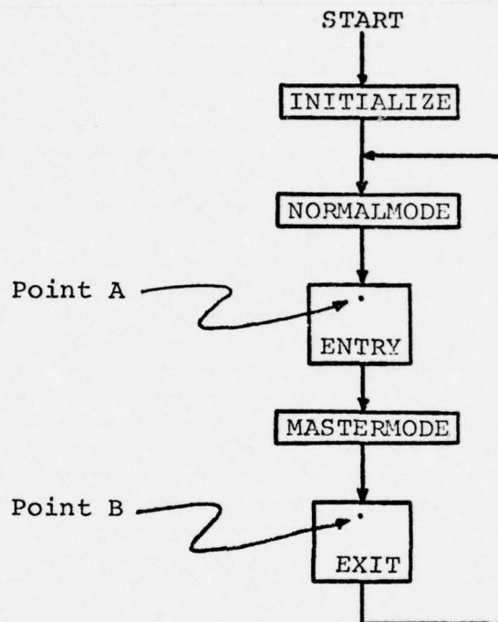
Figure 6. Cyclic Mastermode/Normalmode Program
