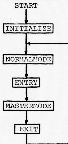
Figure 5. Cyclic Mastermode/Normalmode Program
