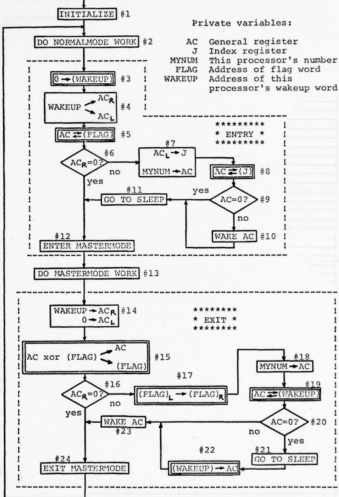
Figure 7. Flowchart of Solution Algorithm
