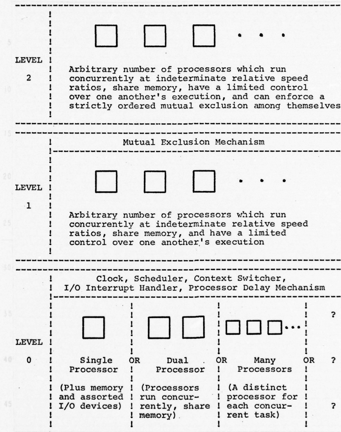
Figure 1. Development of Level-Structured System
