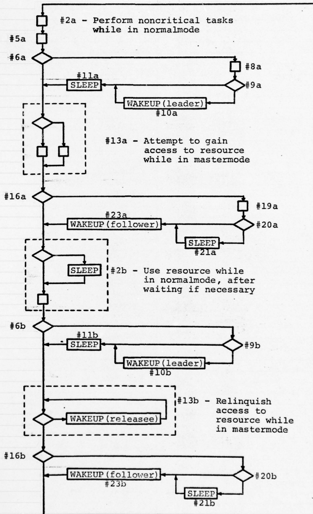
Figure 8. Cyclic Use of a Shared Resource
