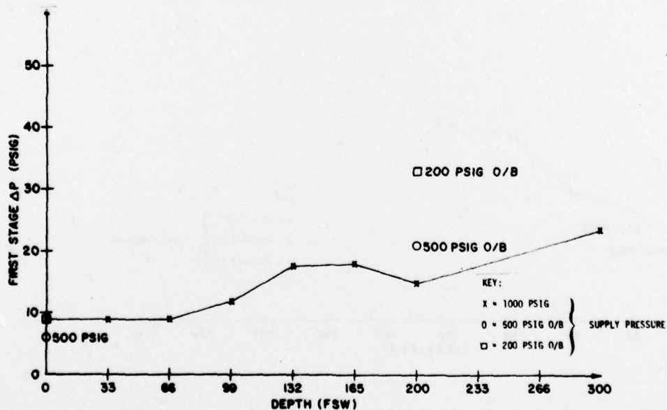
FIGURE 5. FIRST STAGE ΔP VS. DEPTH FOR MR12-II REGULATOR AT 15 BPM, 1.5 TIDAL VOLUME, AND 22.5 RMV
