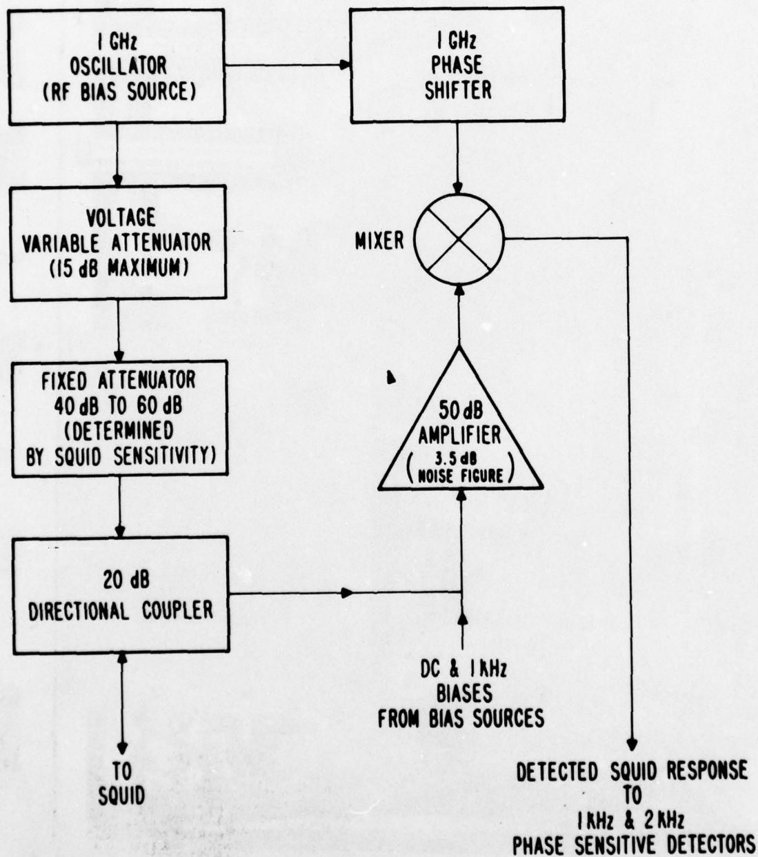
Figure 1.8. Block diagram of microwave bias (1 GHz) circuits.
