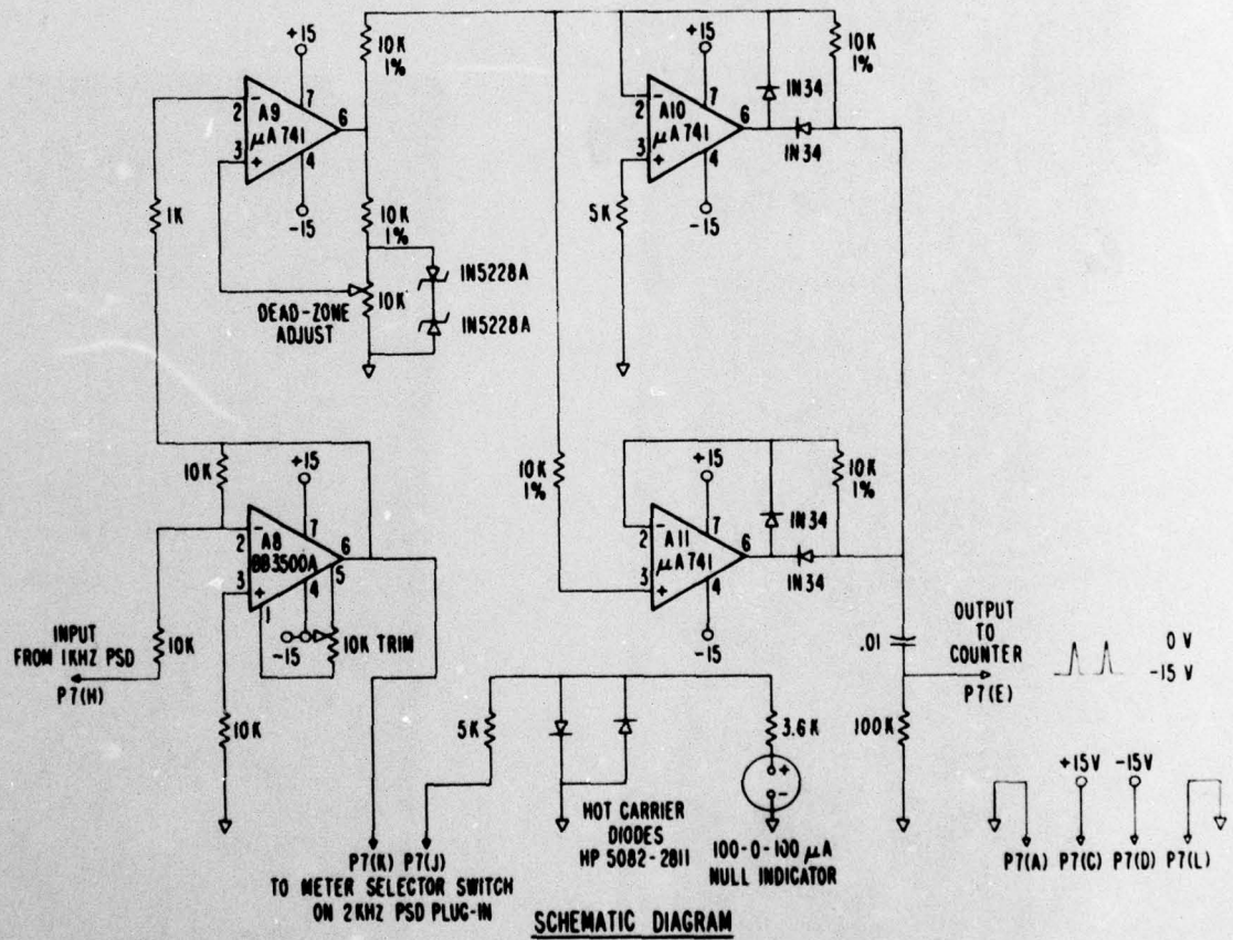
Figure 1.24. Schematic diagram of null indicator and null counting trigger circuits.
