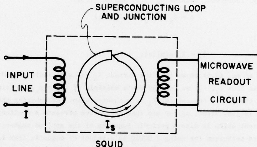
Figure 2.1. Basic SQUID system configuration.
