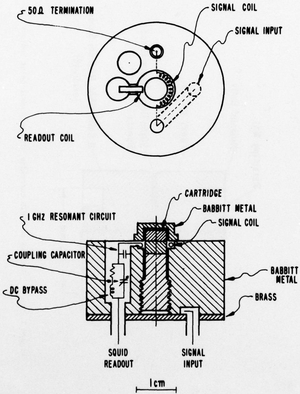
Figure 1.29(b). Diagram of SQUID body containing cartridge.
