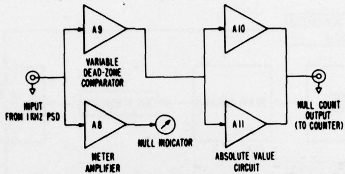
BLOCK DIAGRAM
