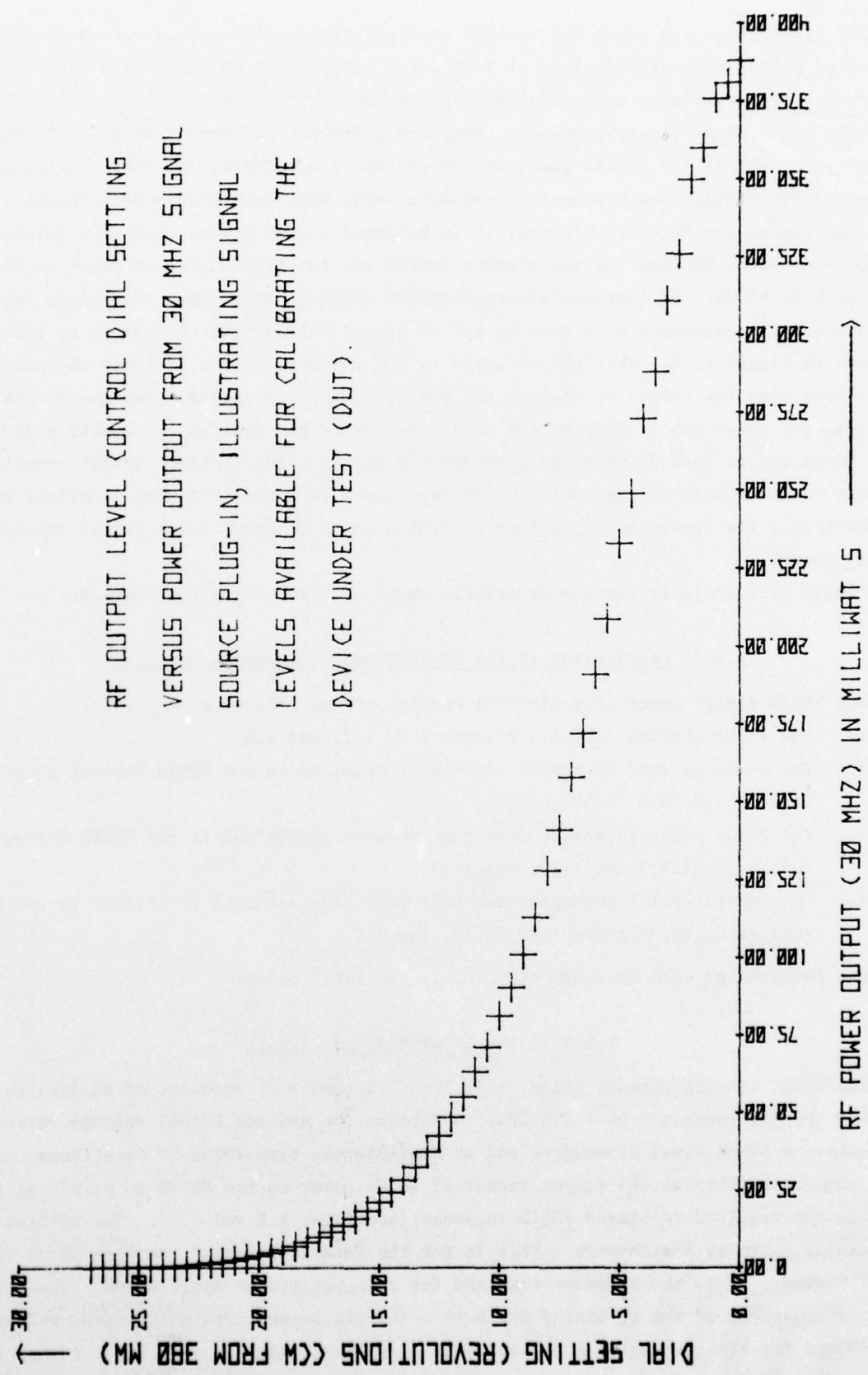
Figure 1.13. RF output level control characteristic curve.
