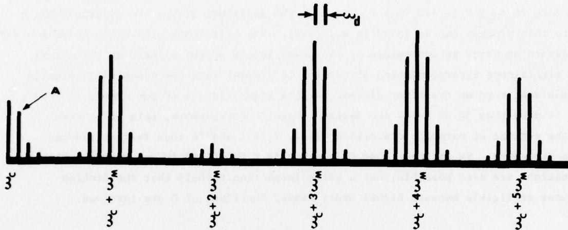
Figure 2.5. Relative sideband amplitudes of the SQUID response.
