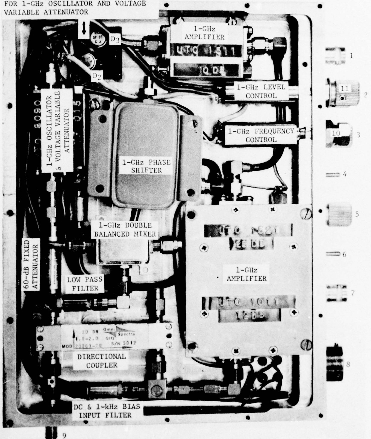
Figure 3.6. Descriptive view of microwave bias (1 GHz) components contained in SQUID control unit.
