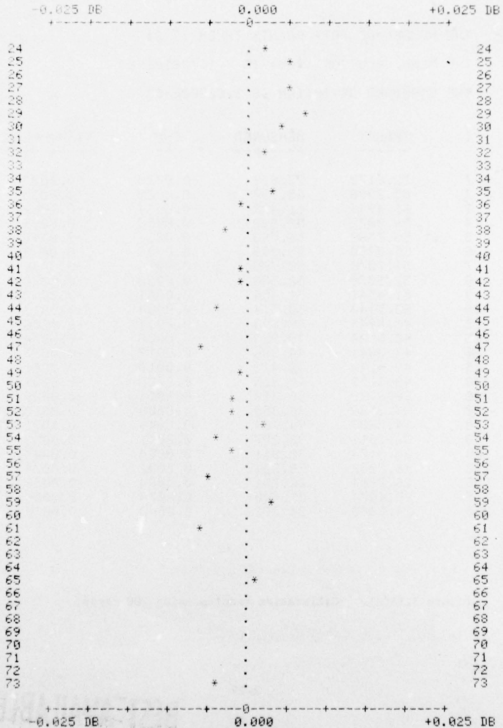
Figure 3.15(b). Calibration curve for attenuation measurements using 200 zeros.
