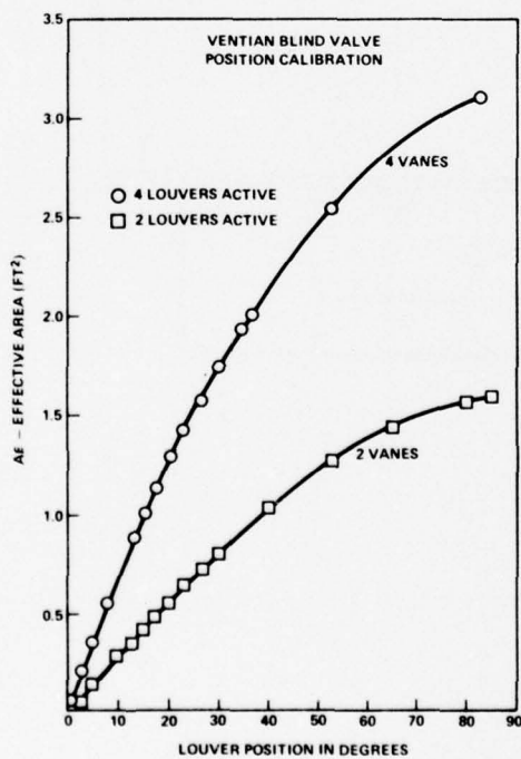
Figure 8 – Flow Control Valve Admittance Characteristics
