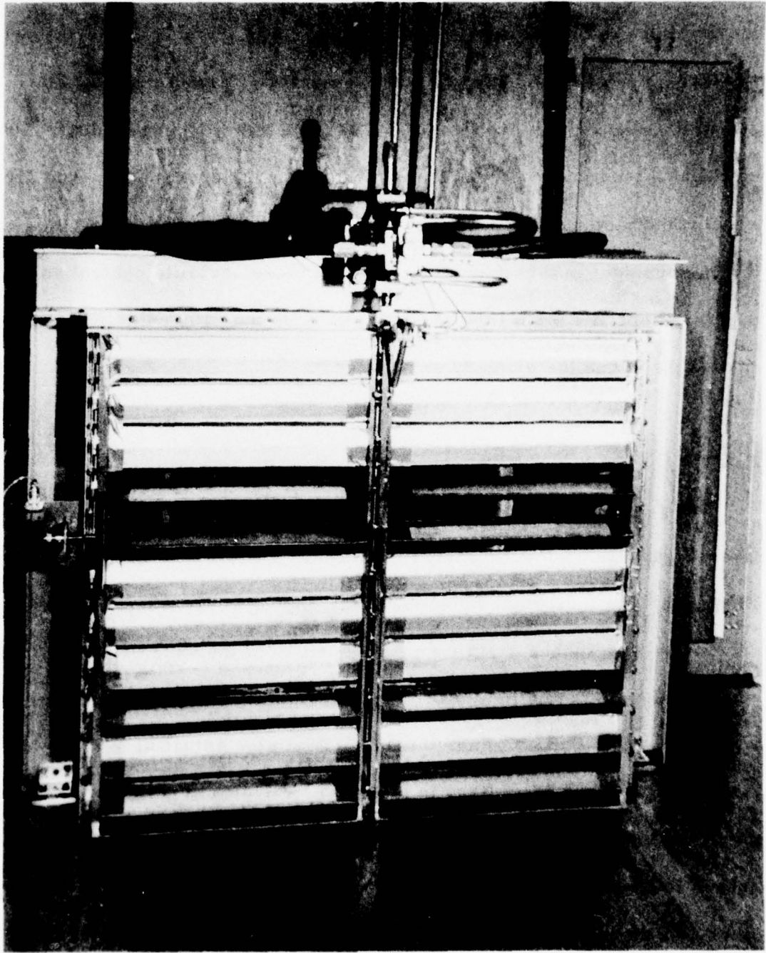
Figure 6 – Louver-Type Flow Control Valve
