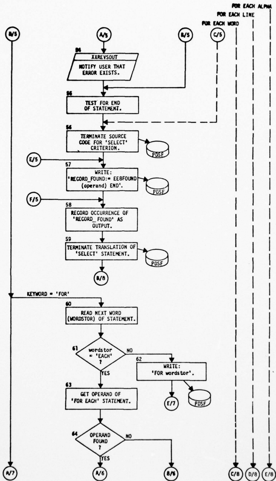
Figure 3-55 Alpha Translation (GGTRALFA) (Continued)
