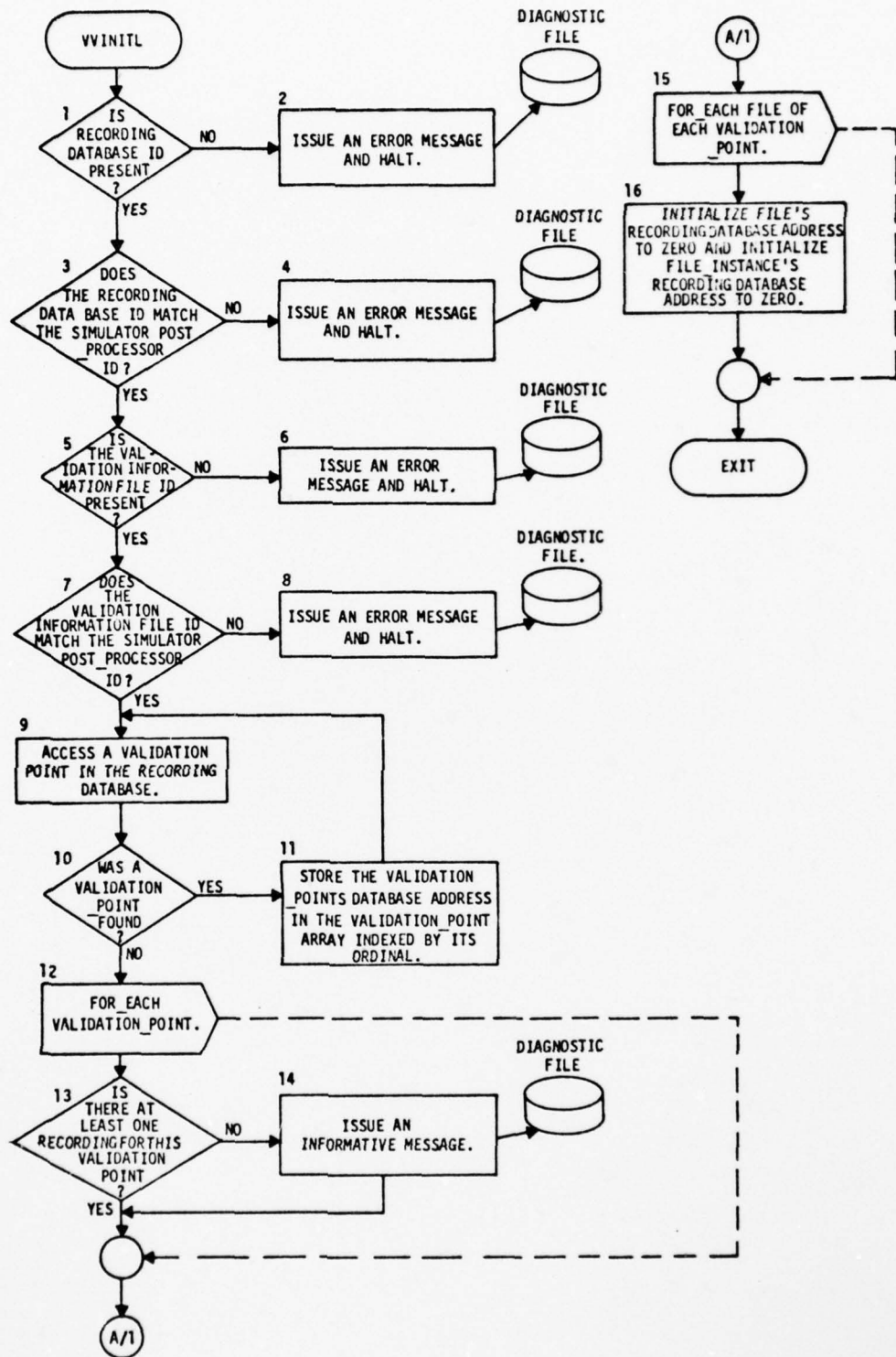
Figure 5-3 Simulator Post-Processor Initialization (VWINITL)
