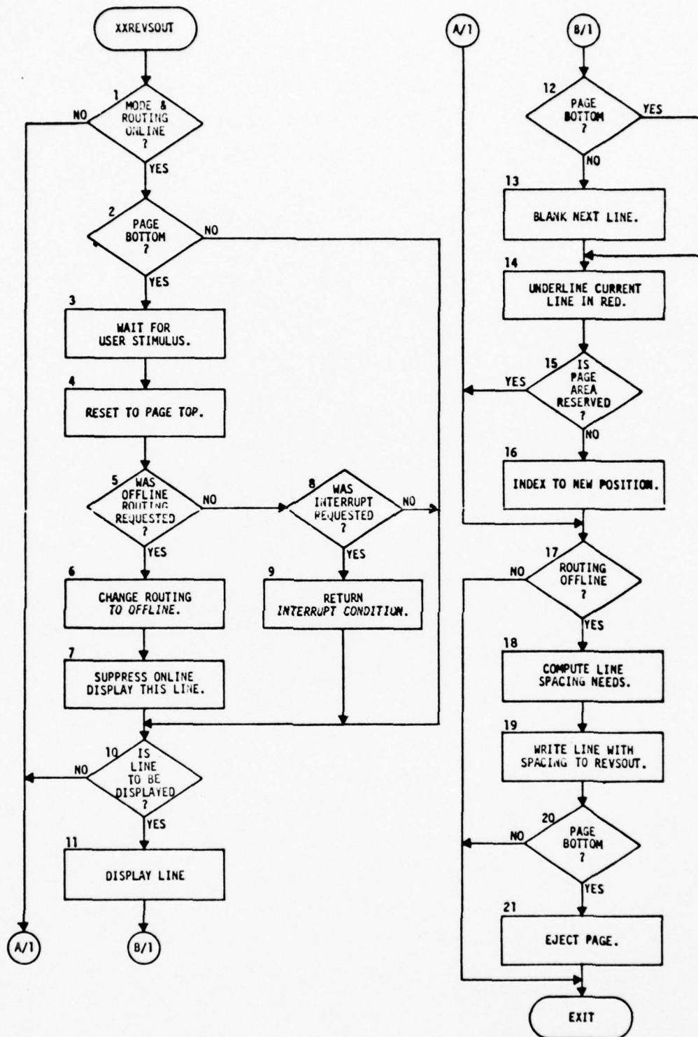
Figure 3-3 REVS Output (XXREVSOUT)
