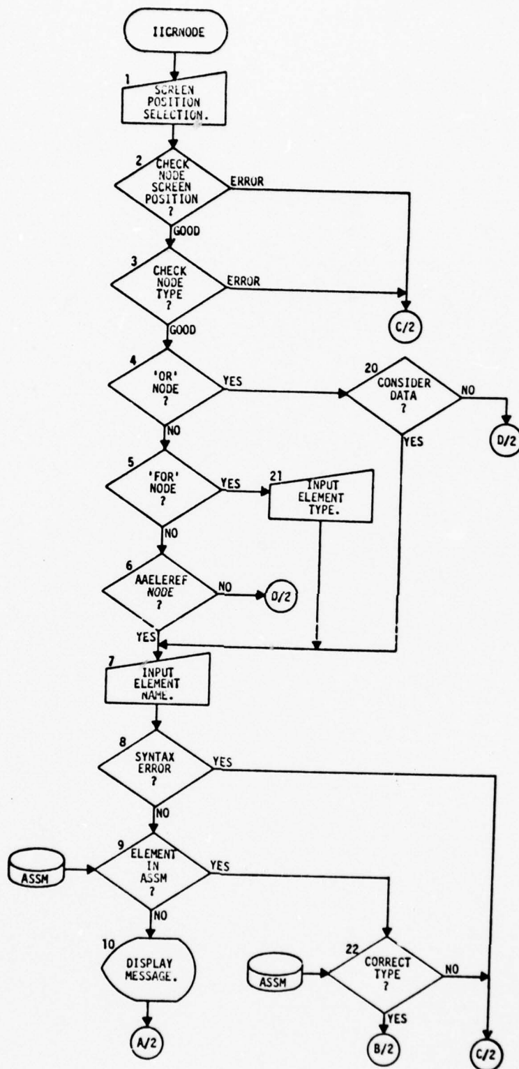
Figure 3-8 Create Node (IICRNODE)
