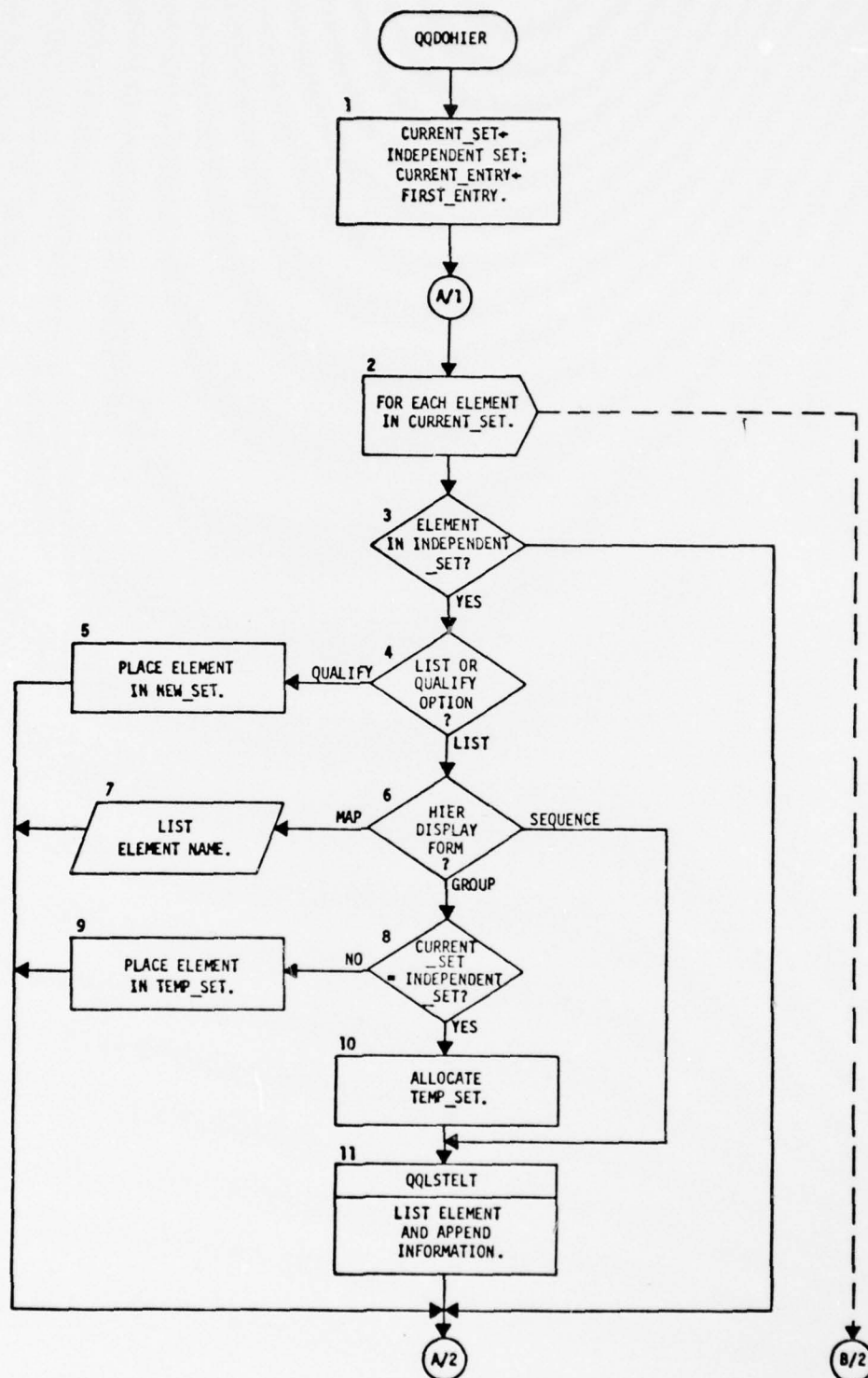
Figure 3-33 List or Qualify Set by Hierarchy (QDOHIER)
