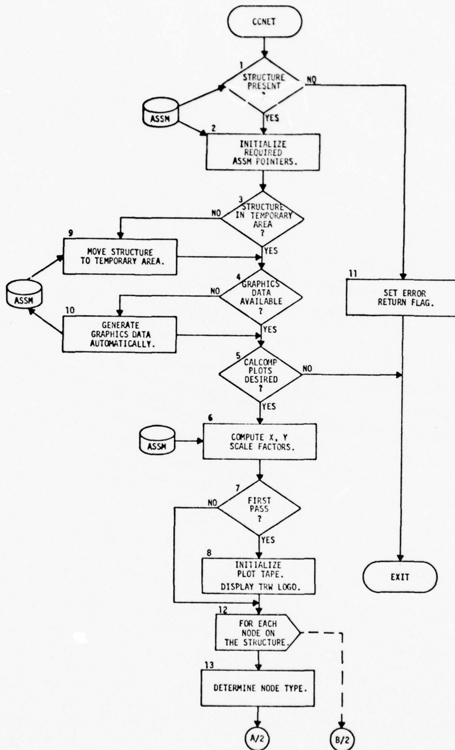
Figure 3-26 CALCOMP Net Display (CCNET)
