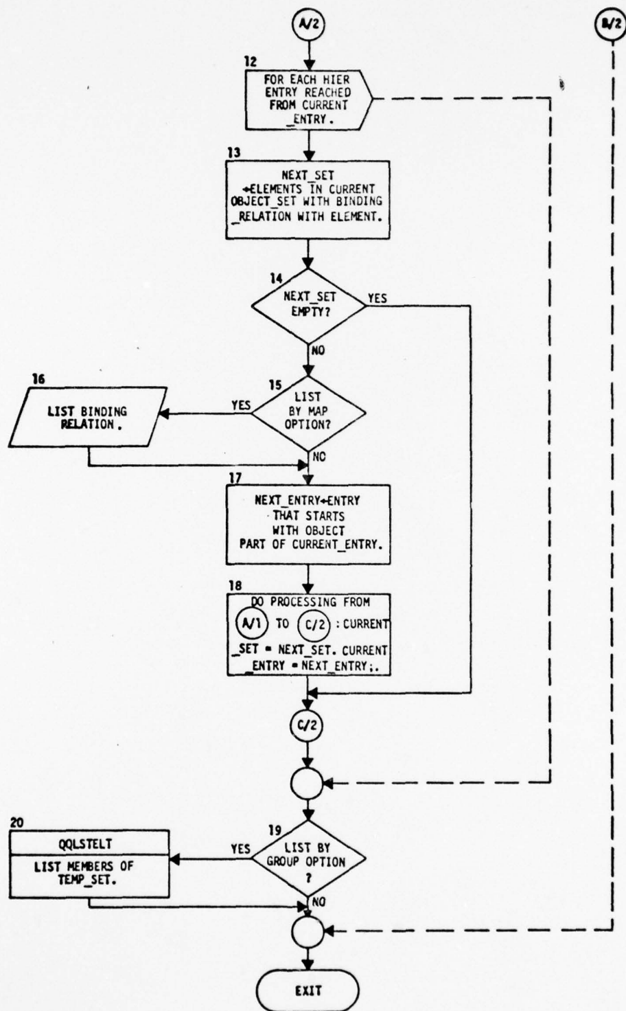
Figure 3-33 List or Qualify Set by Hierarchy (QQDOHIER) (Continued)
