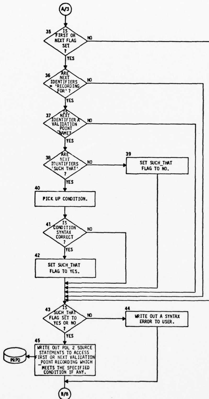
Figure 3-58.2 Performance-Requirement Translation (GGTRPR) (Continued)
