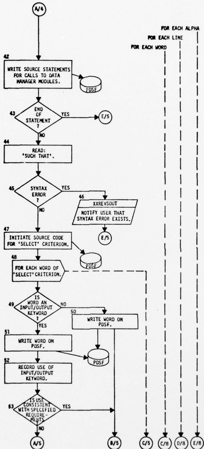
Figure 3-55 Alpha Translation (GGTRALFA) (Continued)
