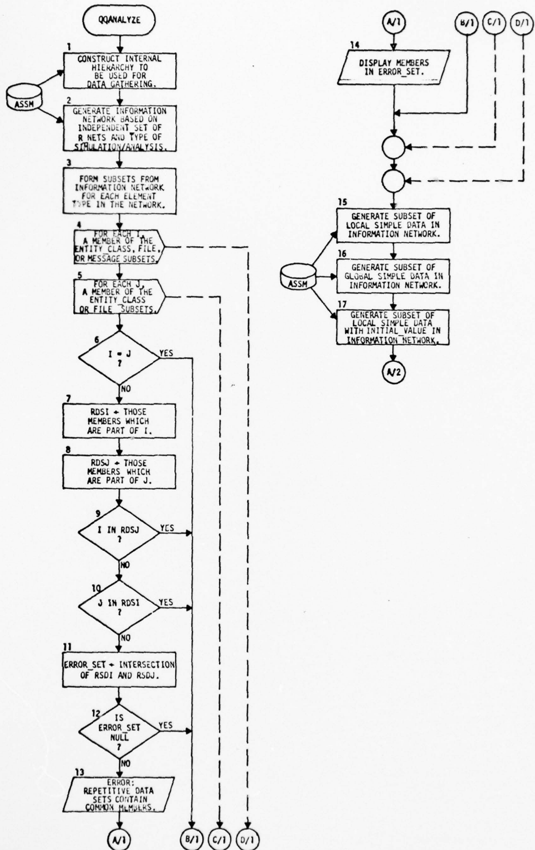
Figure 3-38 Requirements Analysis (QQANALYZE)
