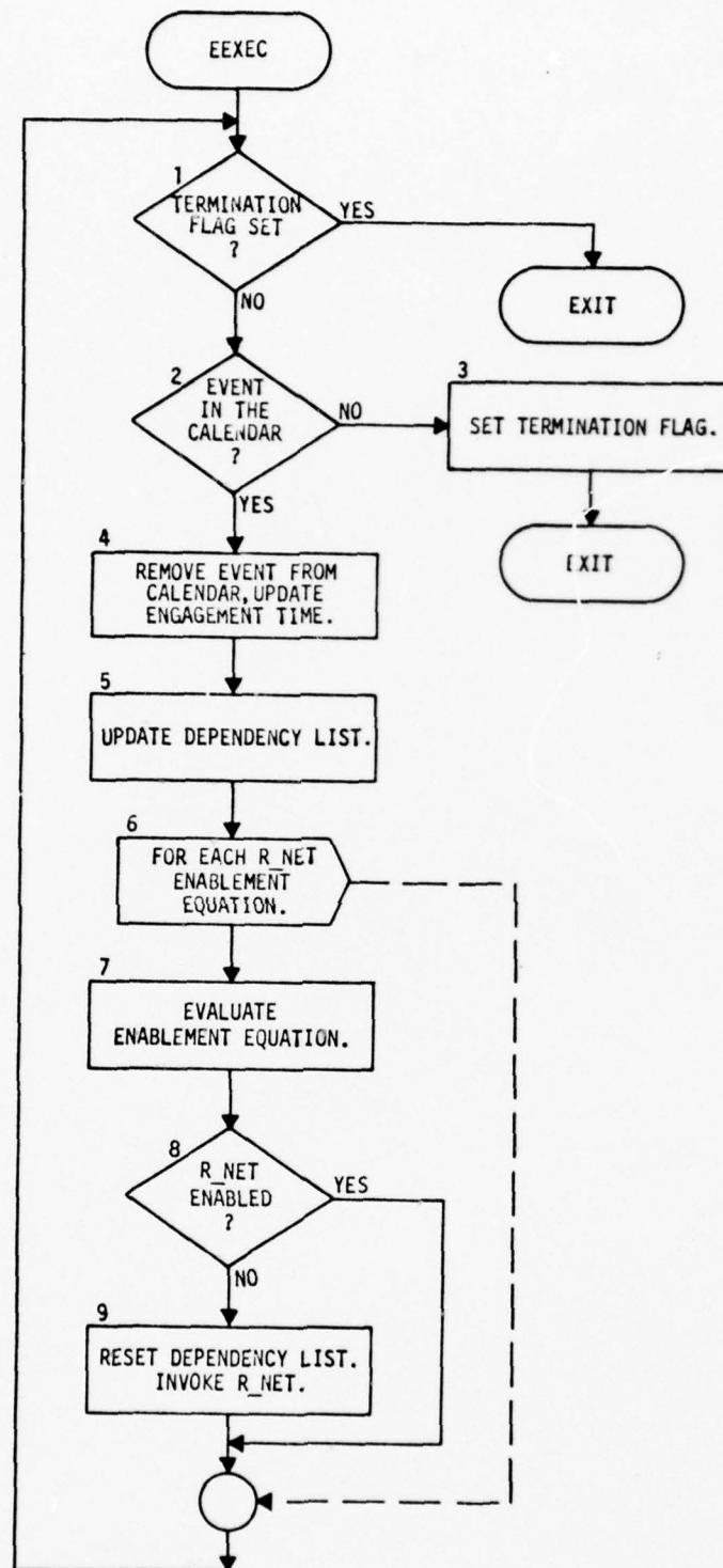
Figure 4-4 Simulator Executive (EEXEC)
