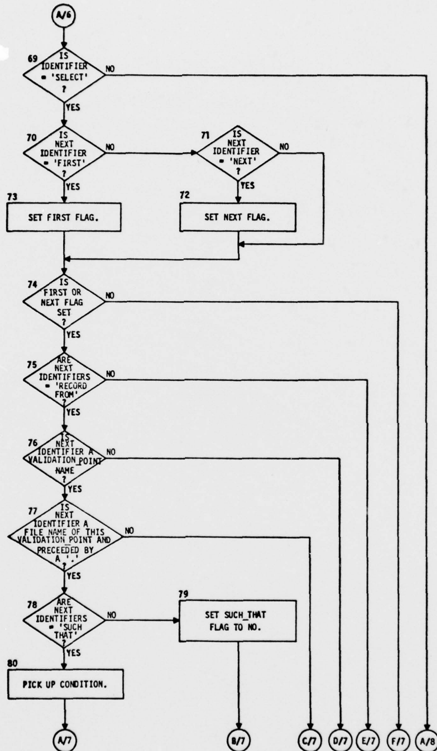
Figure 3-58.2 Performance-Requirement Translation (GGTRPR) (Continued)
