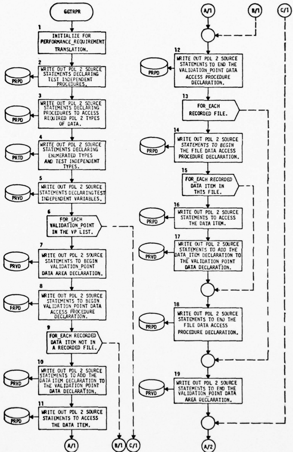
Figure 3-58.2 Performance-Requirement Translation (GGTRPR)
