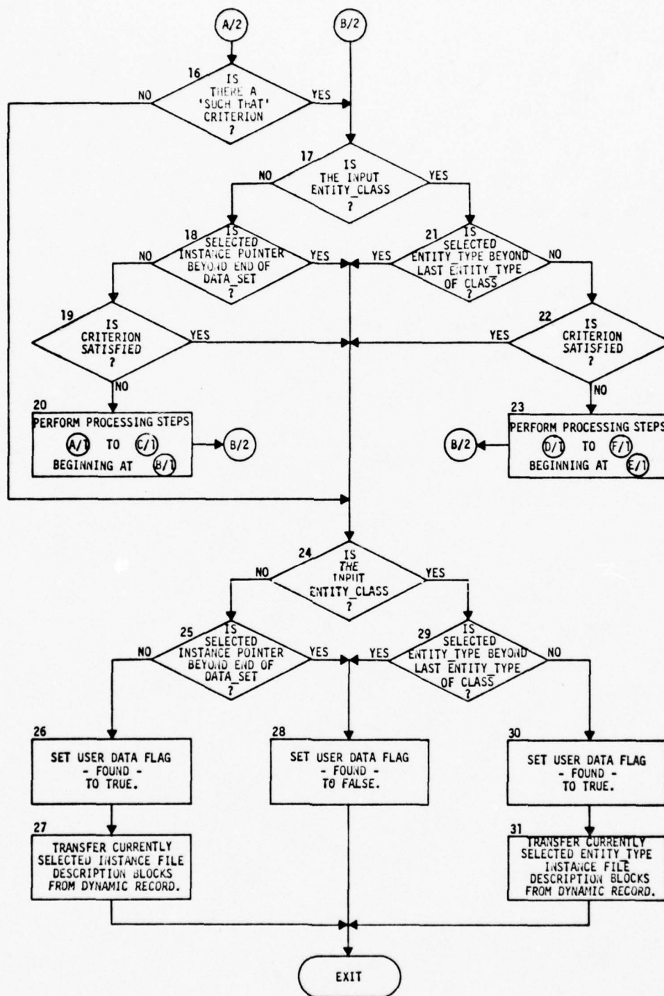
Figure 4-12 SELECT FIRST (Continued)
