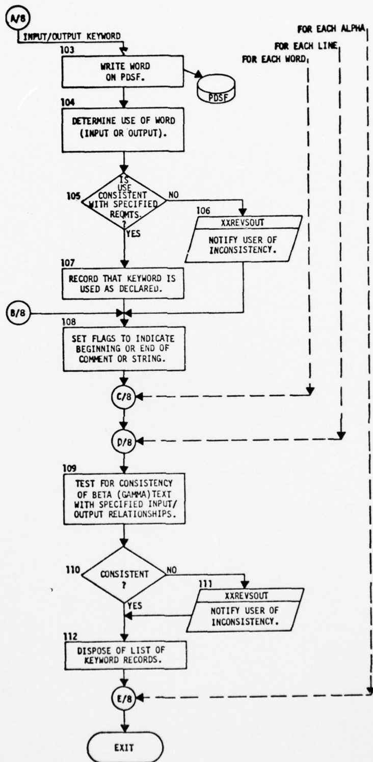
Figure 3-55 Alpha Translation (GGTRALFA) (Continued)
