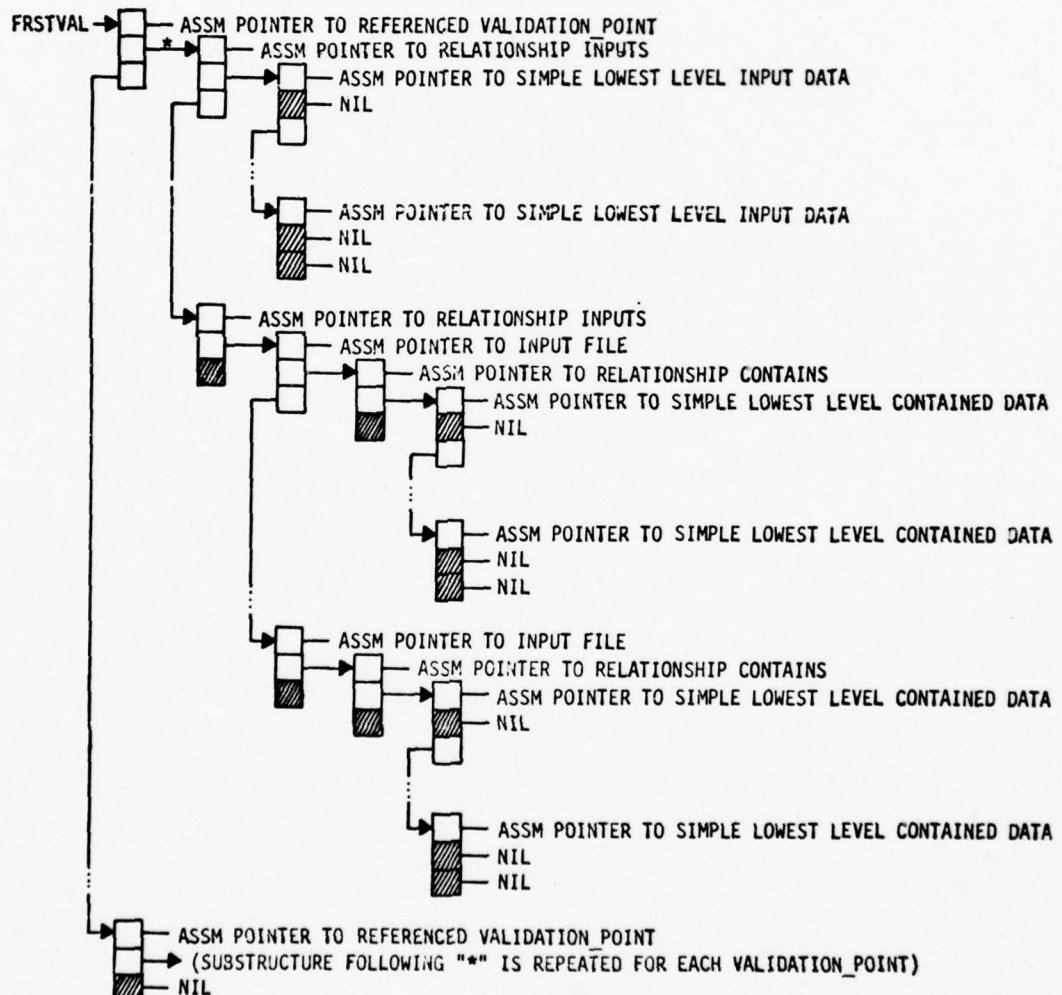
Figure 3-47 VALIDATION_POINT List (VALLIST)
