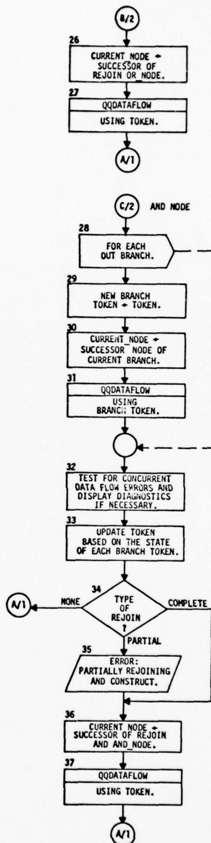
Figure 3-39 Data Flow Analysis (QDATAFLOW) (Continued)
