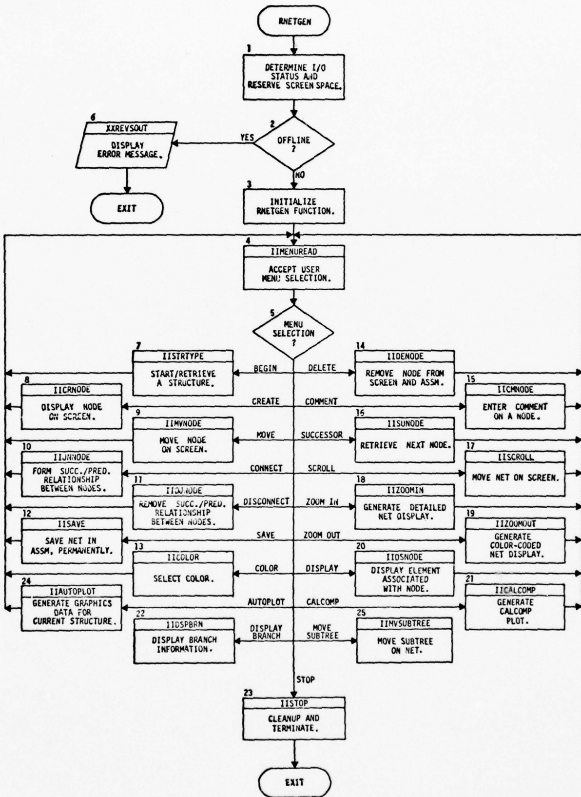
Figure 3-6 R-Net Generation (RNETGEN)
