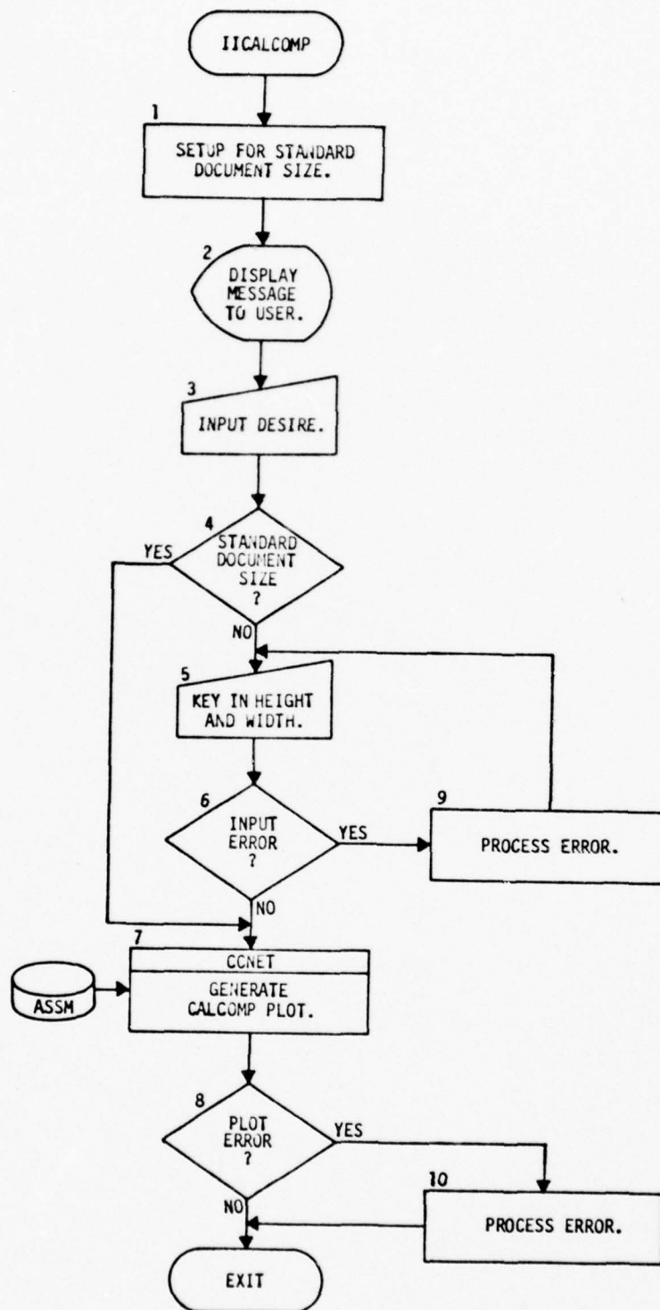
Figure 3-19 Generate CALCOMP Plot (IICALCOMP)
