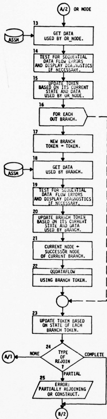
Figure 3-39 Data Flow Analysis (QDATAFLOW) (Continued)
