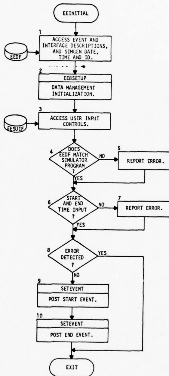
Figure 4-3 Simulator Initialization (EEINITIAL)
