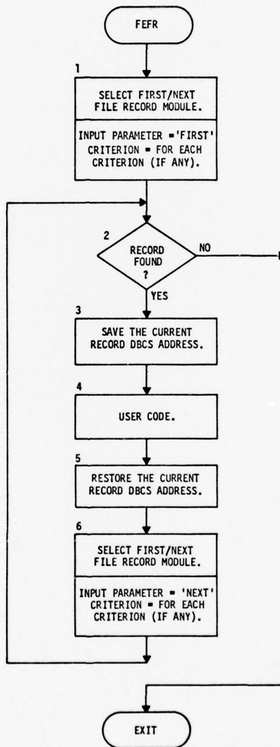
Figure 5-9 For Each File Record (FEFR)
