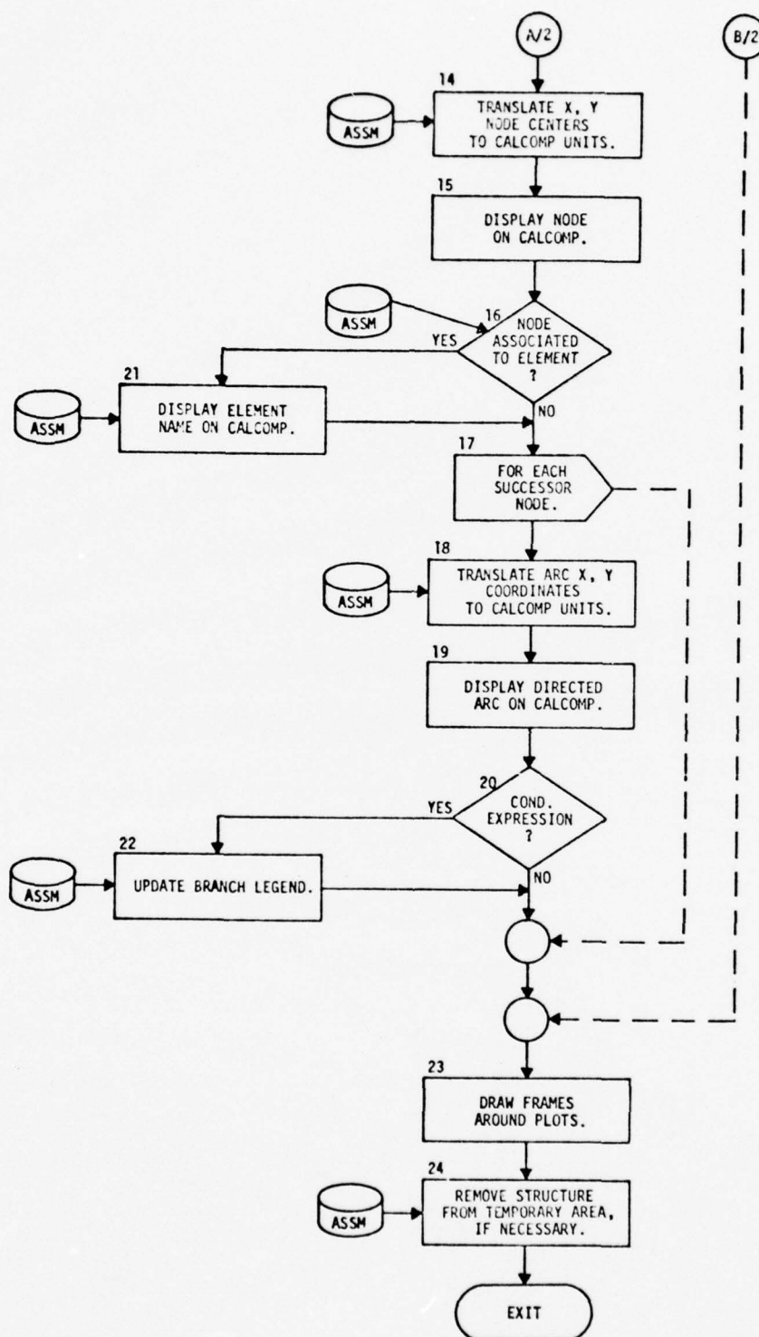
Figure 3-26 CALCOMP Net Display (CCNET) (Continued)
