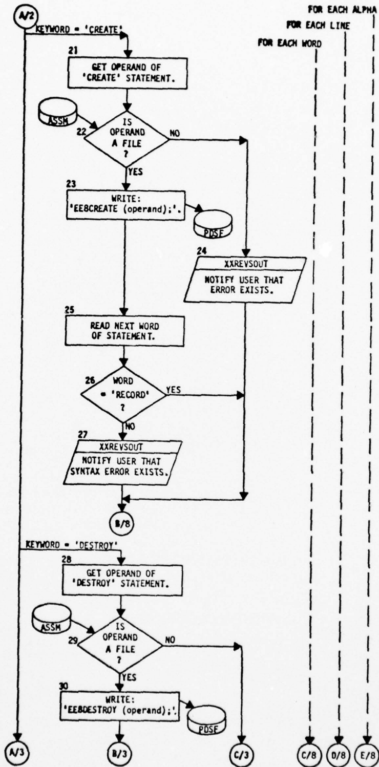
Figure 3-55 Alpha Translation (GGTRALFA) (Continued)
