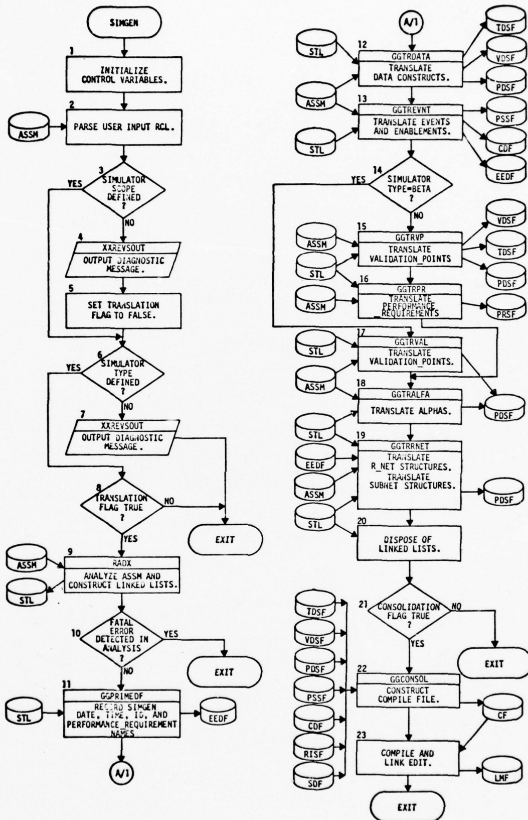
Figure 3-48 Simulator Generation (SIMGEN)
