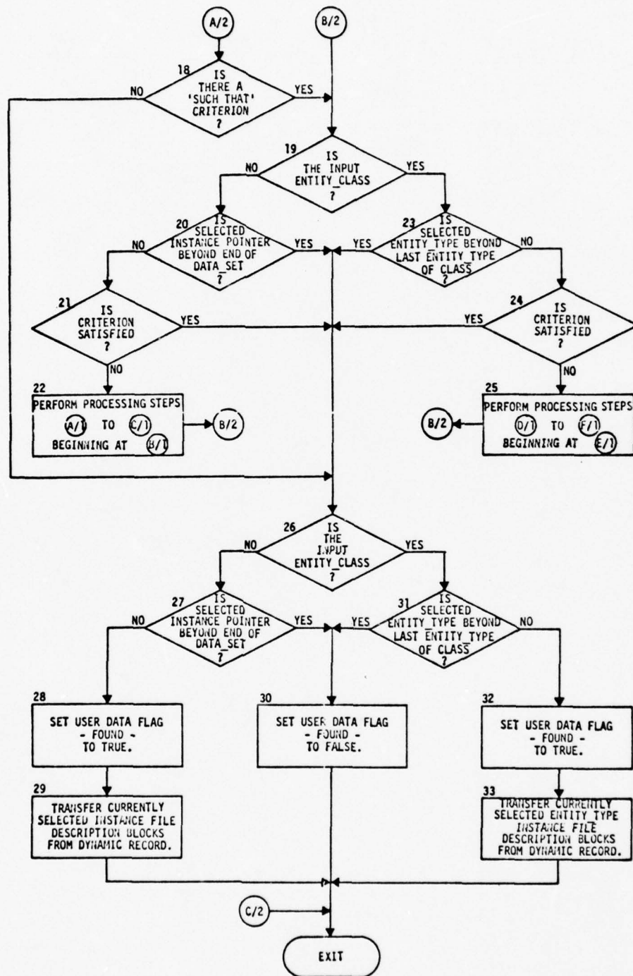
Figure 4-13 SELECT NEXT (Continued)
