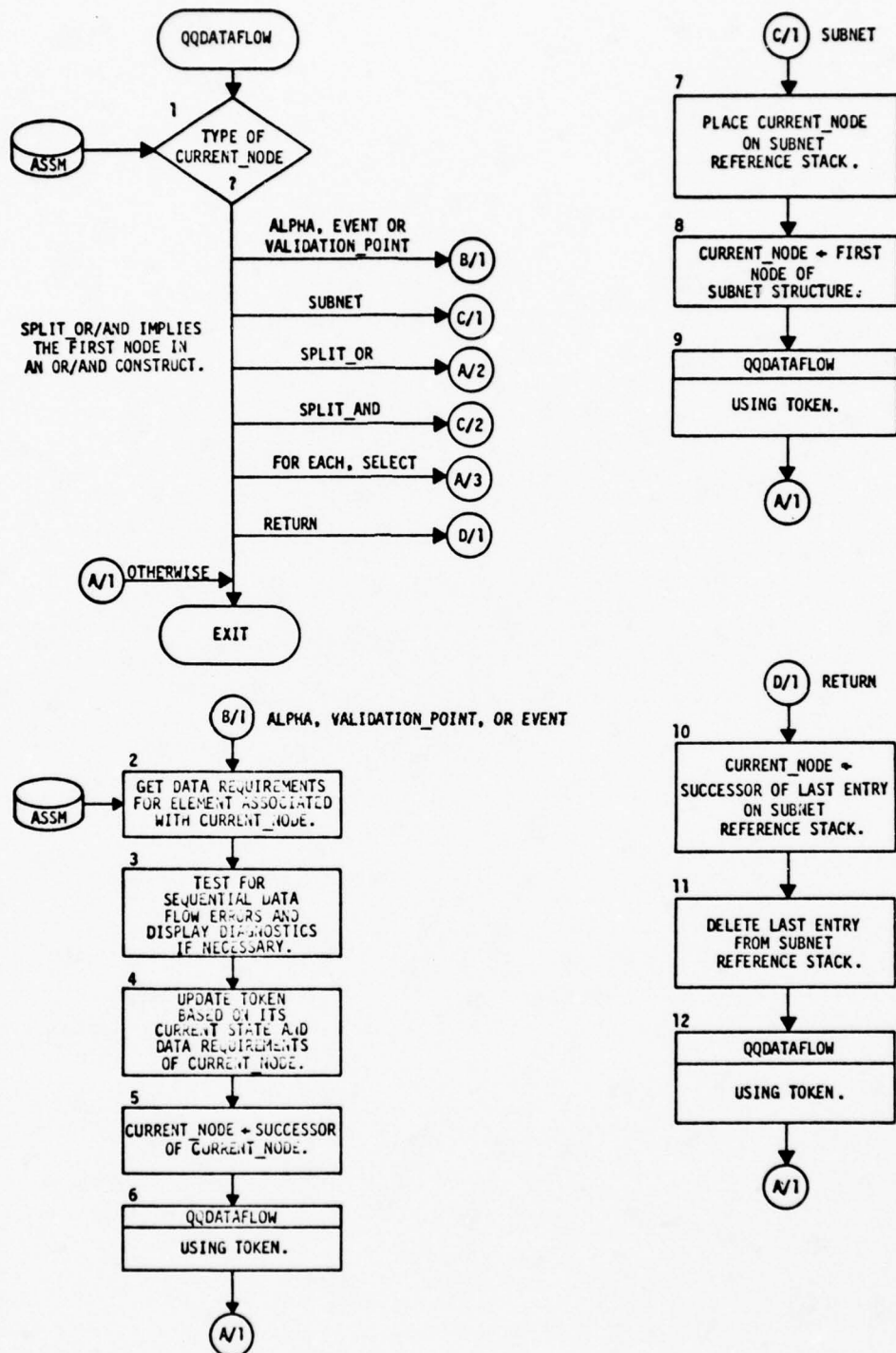
Figure 3-39 Data Flow Analysis (QQDATAFLOW)
