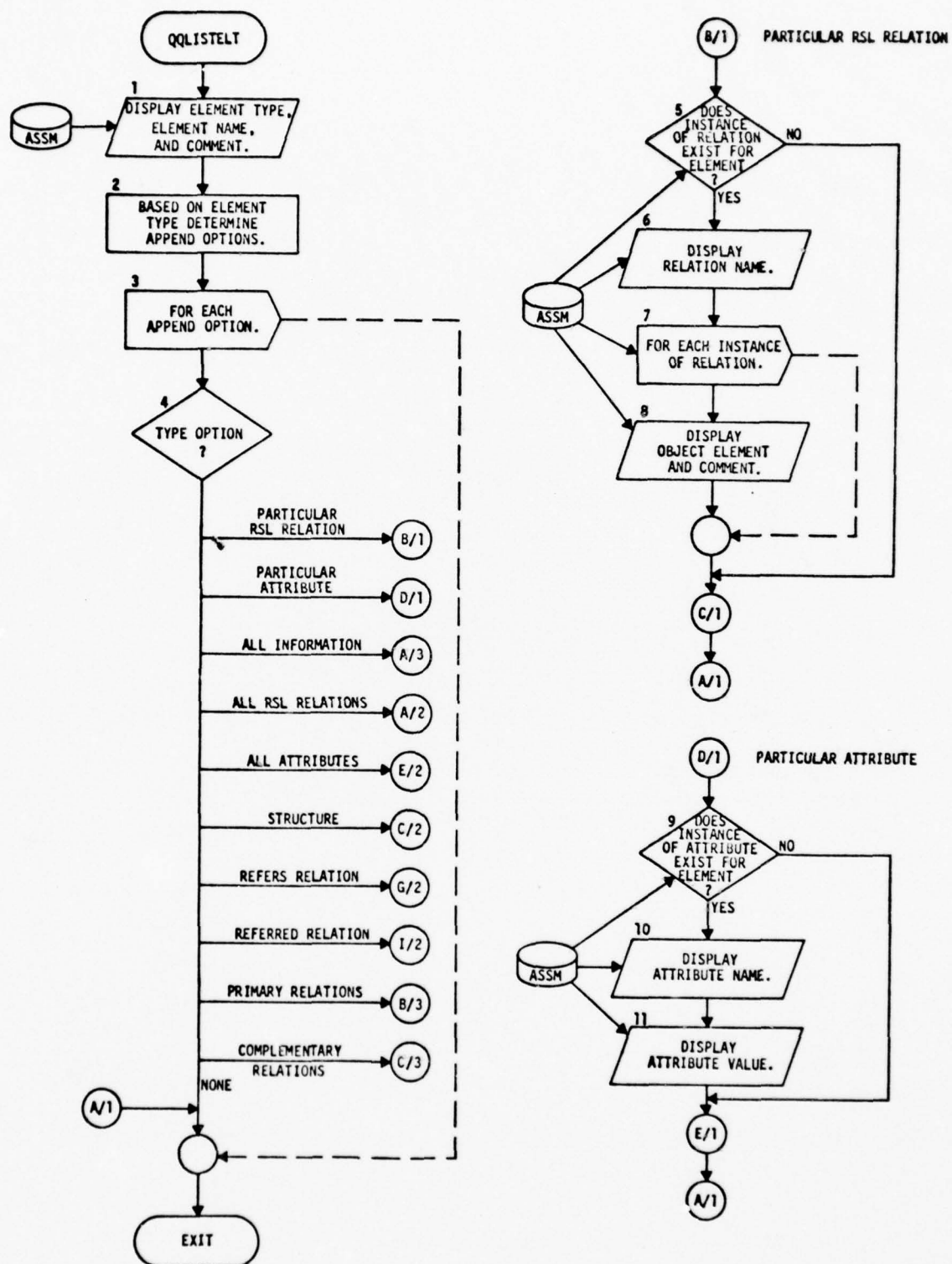
Figure 3-35 List Element (QQLISTELT)
