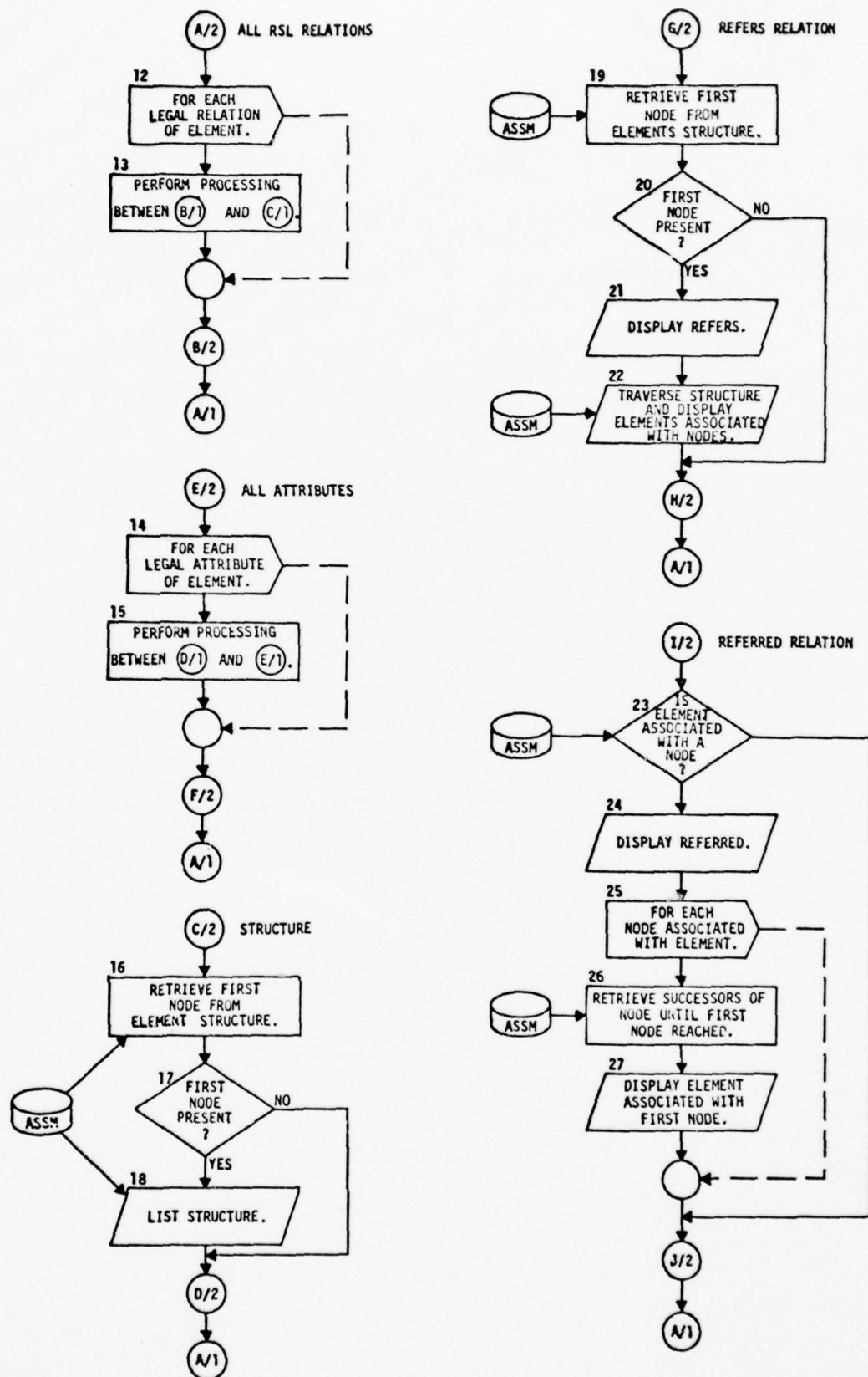
Figure 3-35 List Element (QQLISTELT) (Continued)
