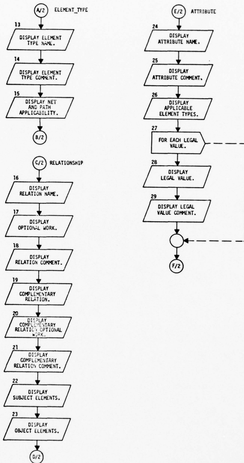
Figure 3-36 List RSL (QQLSTRSL) (Continued)
