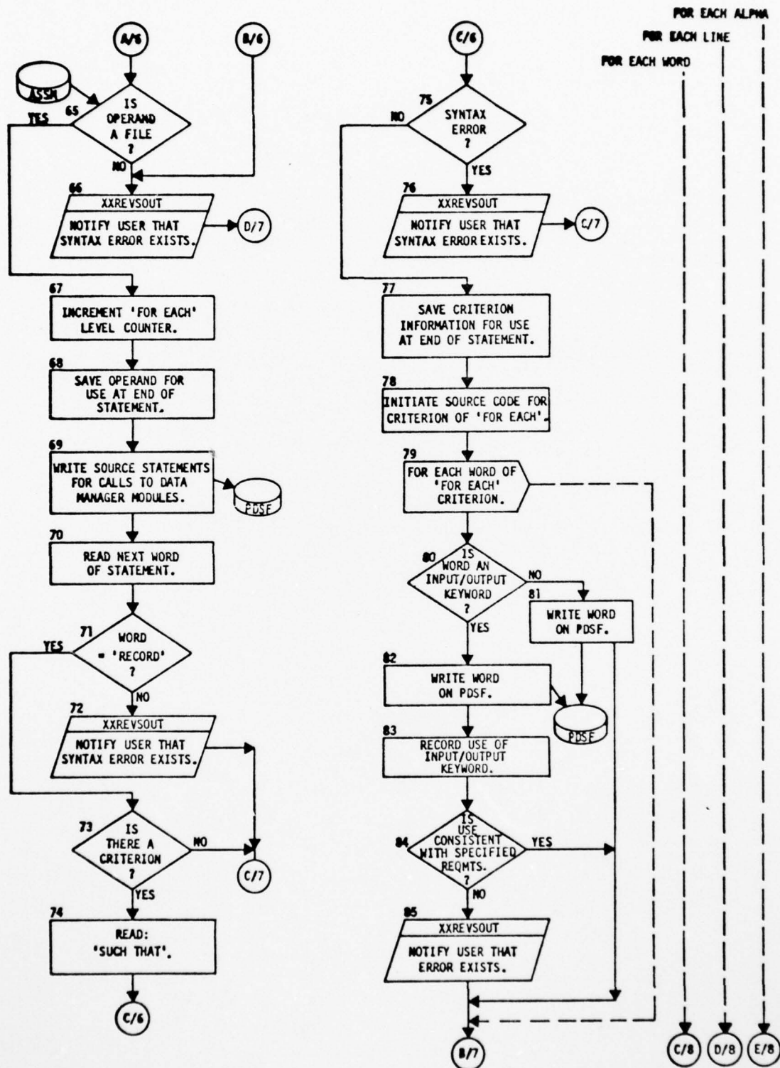
Figure 3-55 Alpha Translation (GGTRALFA) (Continued)
