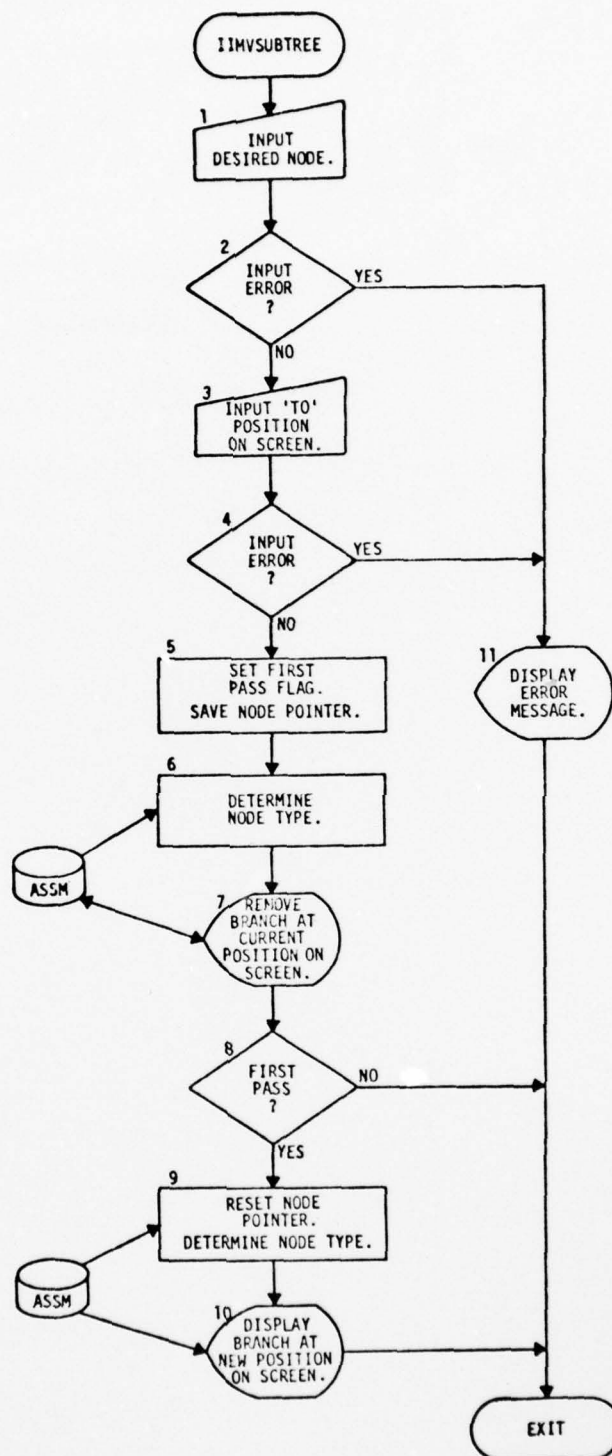
Figure 3-26.2 Move Subtree (IIMVSUBTREE)
