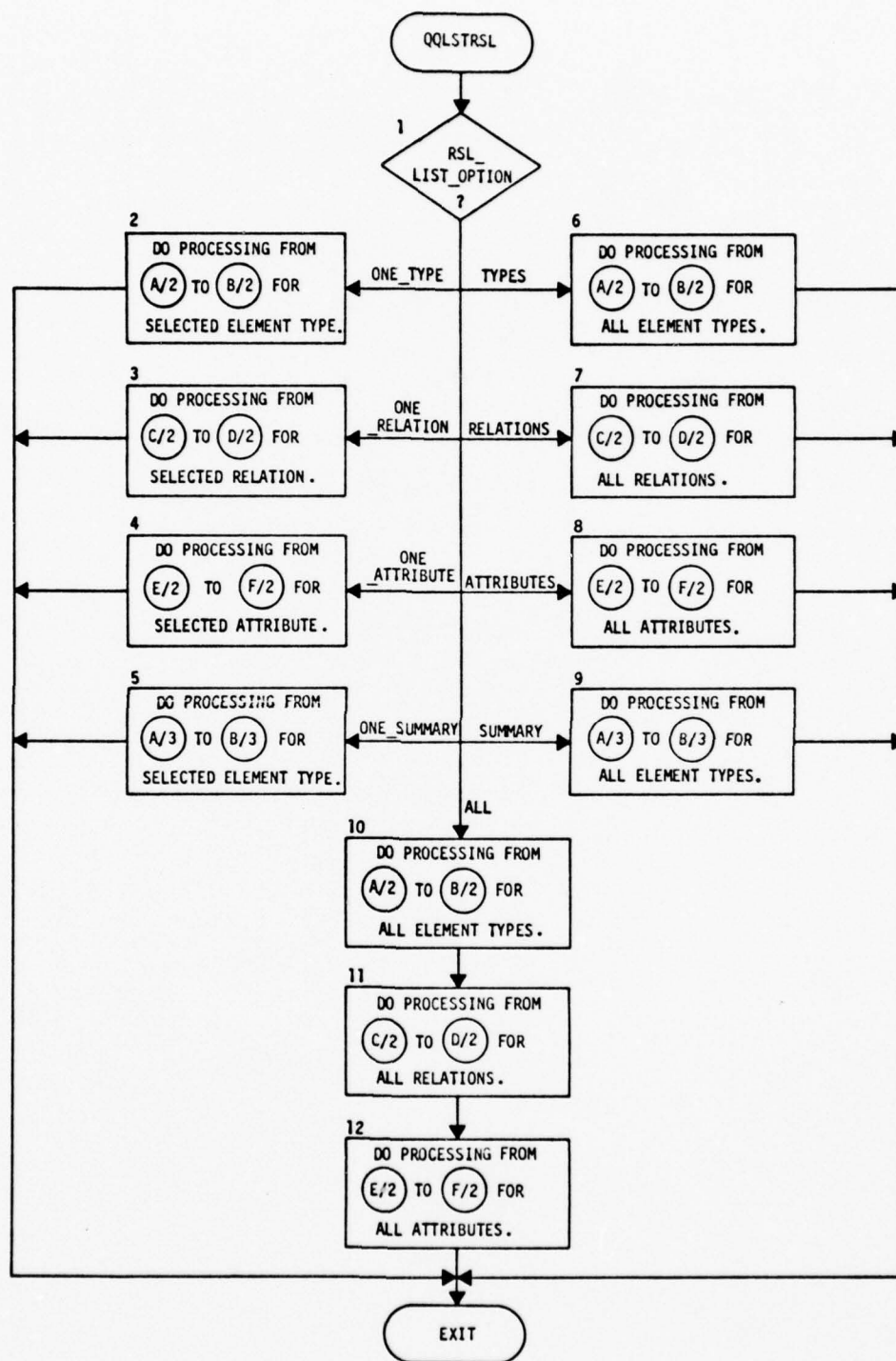
Figure 3-36 List RSL (QQLSTRSL)
