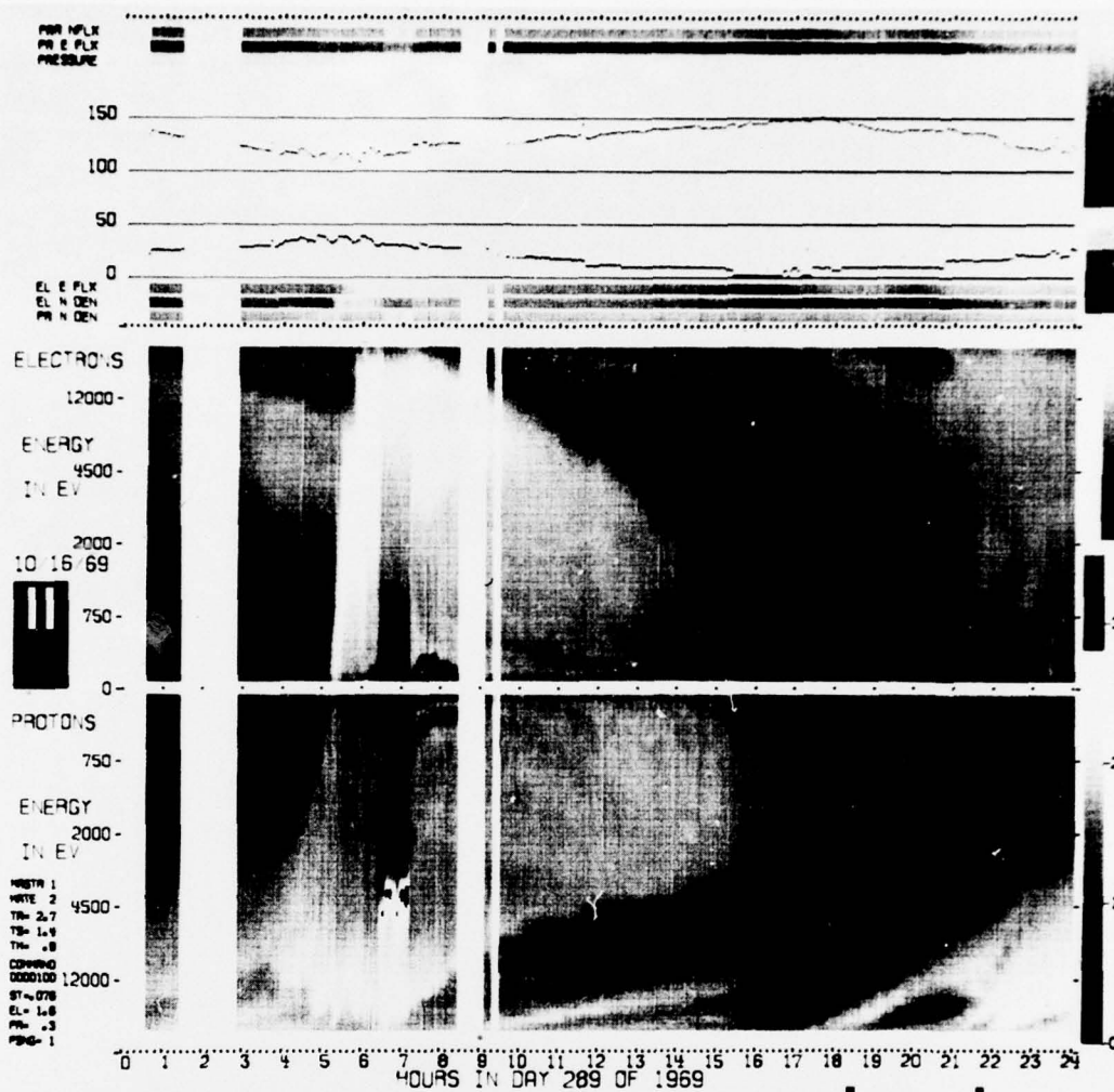
Figure 12. Day 289, 1969, Spectrogram From ATS-5 Which Exhibits the Buildup (during an injection event) and Decay (during eclipse) of Differential Charge on the Satellite
