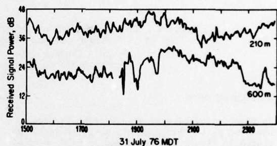
Figure C8. Temporal variation of received signal power for two heights (210 m, 600 m). System averaging time constant was 2 min.
