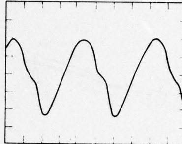
Figure B3. Microphone output with microphone positioned as shown in Figure B1. (one div = 848 dynes/cm 2 .) (Negative pressure is up.)
