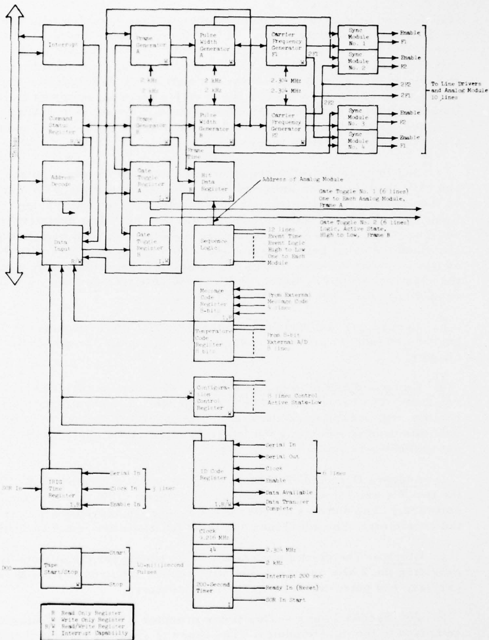
FIGURE 3-24 Block Diagram, Radar Controller
