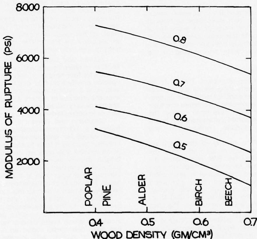
Figure 12.--Relationship between wood density and modulus of rupture for four particleboard densities.
