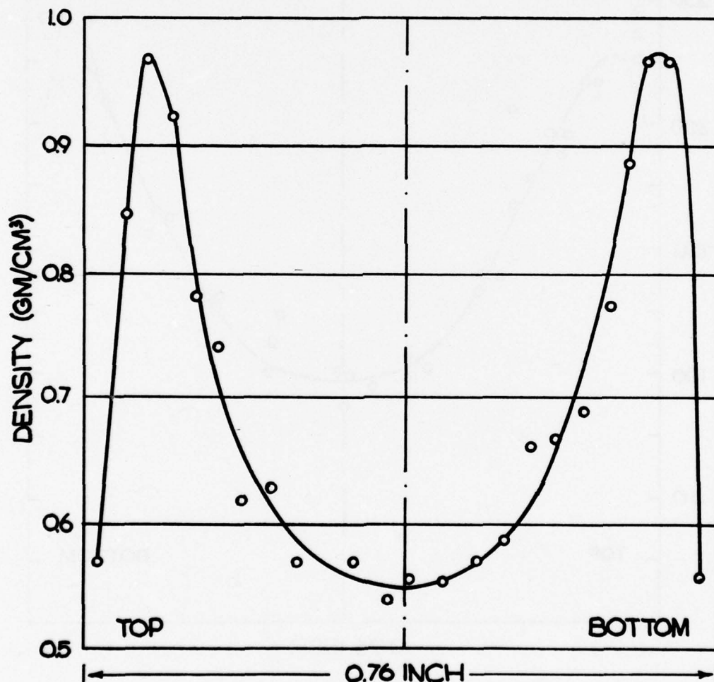
Figure 1.--Vertical density gradient of a three-layer particleboard. (From Plath and Schnitzler 1974) (M 144 401)
