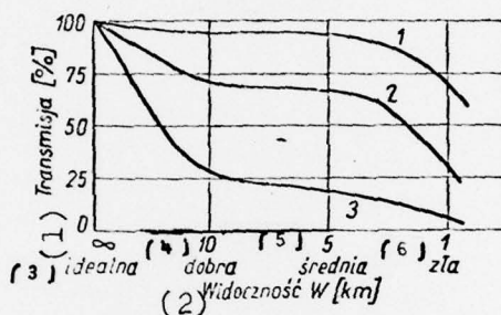
Figure 2. Dependence of the light transmission on the state of visibility of the atmosphere: Curve 1 - for a distance of 200 m; curve 2 - for a distance of 1 km; curve 3 - for a distance of 8 km. Key: (1) Transmission; (2) Visibility; (3) ideal; (4) good; (5) average; (6) bad.
