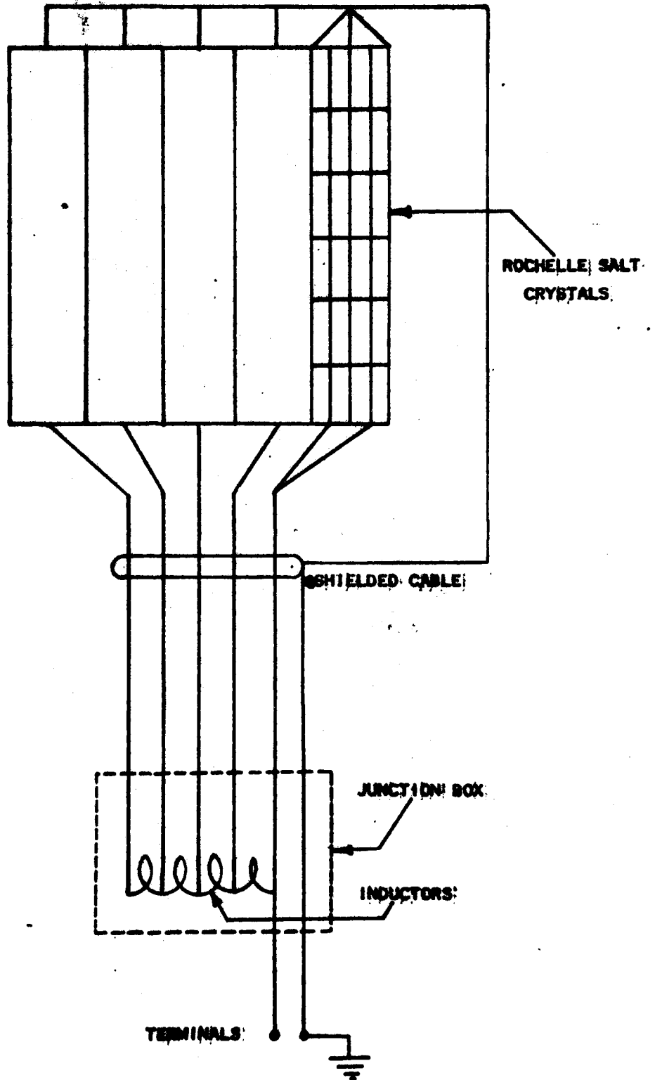
Figure 1., Schematic of Transducer and Log Line
